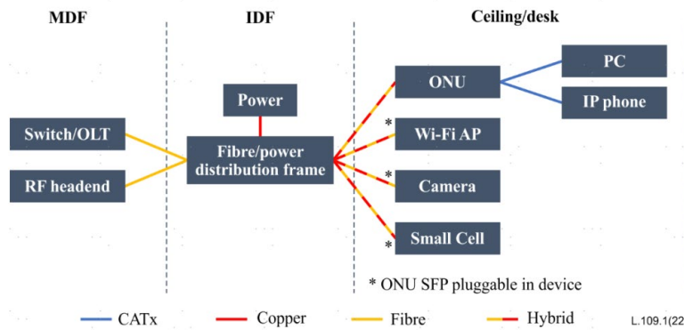
Power and data delivery networking based on OEHC
