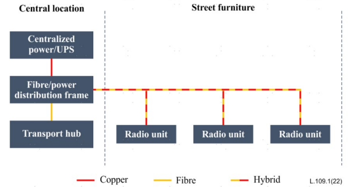
Centralised fibre connectivity and power delivery network based on multi fibre OEHC
