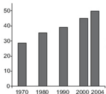
Figure 1: Total Greenhouse Gases (in Gigatonnes of Carbon Dioxide equivalents – GtCO 2 -eq)
