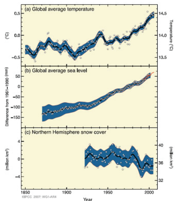
Figure 2: Long-term changes related to the climate
