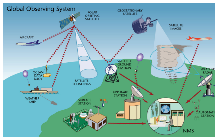
Figure 4: WMO Global Climate Observing System
