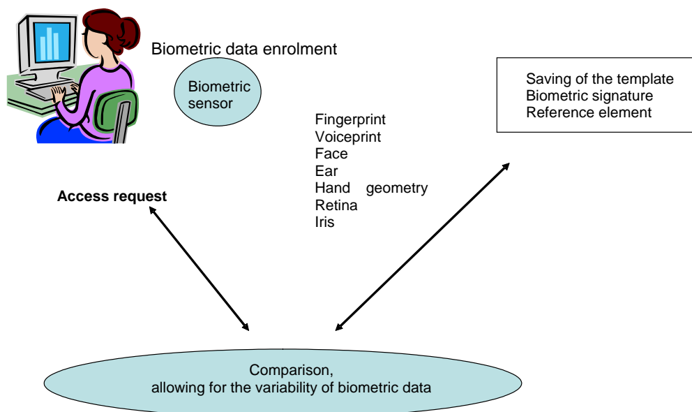
Figure III.12 – Biometric access control
