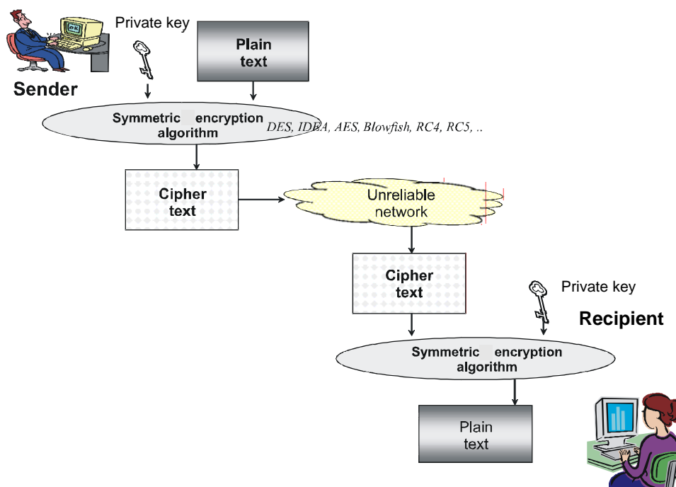
Figure III.5 – Symmetric encryption
