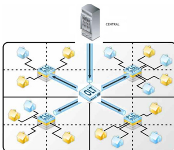
Figure 9: FTTH network topology
