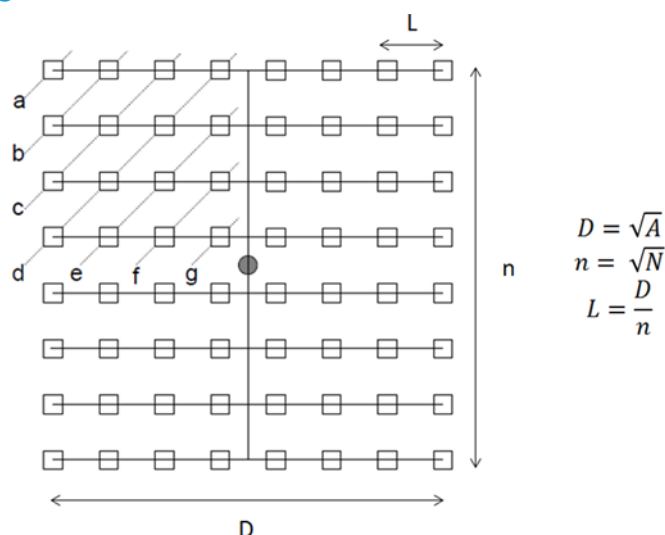
Figure 10: SSL geometric model
