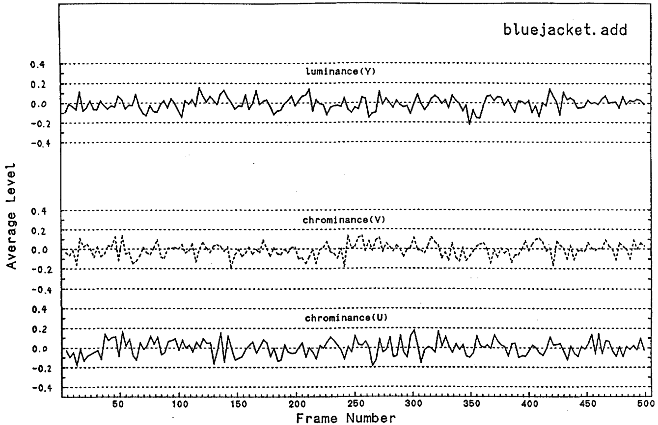
Fig. 4: average of the interframe difference signal
