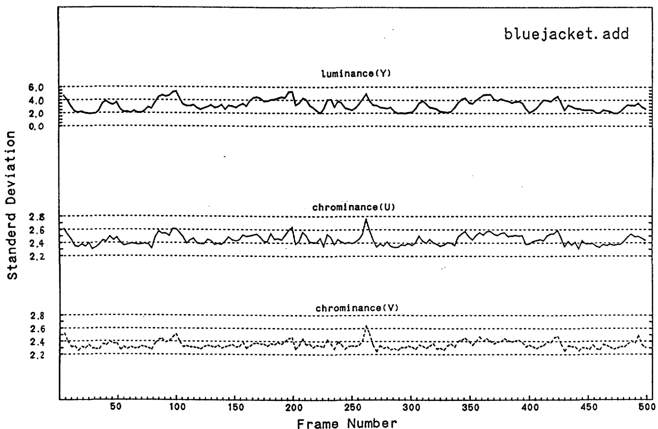
Fig. 5: standard deviation of the interframe difference signal
