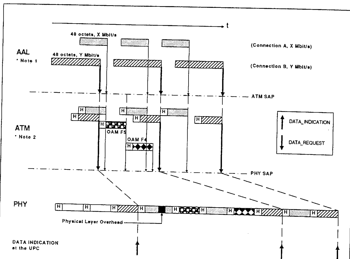
Figure 3/I.371 - Origins of Cell Delay Variation
