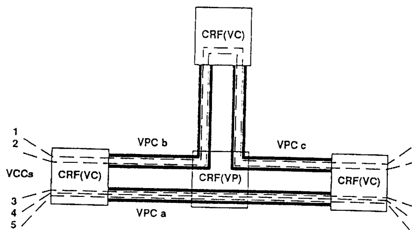
Figure 5/I.371 - Mapping Cell Loss Ratios for Virtual Channel Connections and Virtual Path Connections
