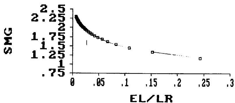
Figure 3: SMG vs. EL/LR
