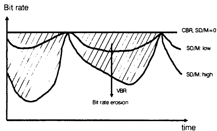
Figure 1: VBR as an erosion of CBR
