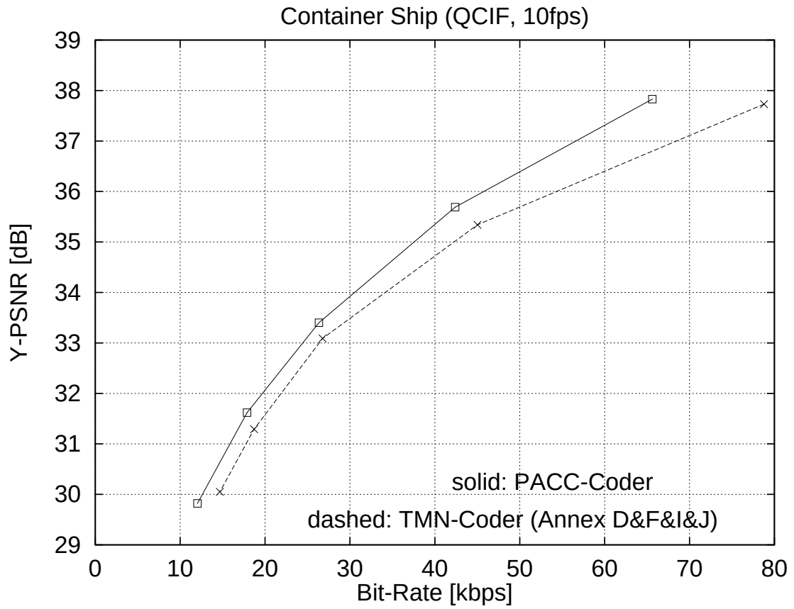
Fig. 11: RD-Comparison of PACC and TMN for CONTAINER SHIP.
