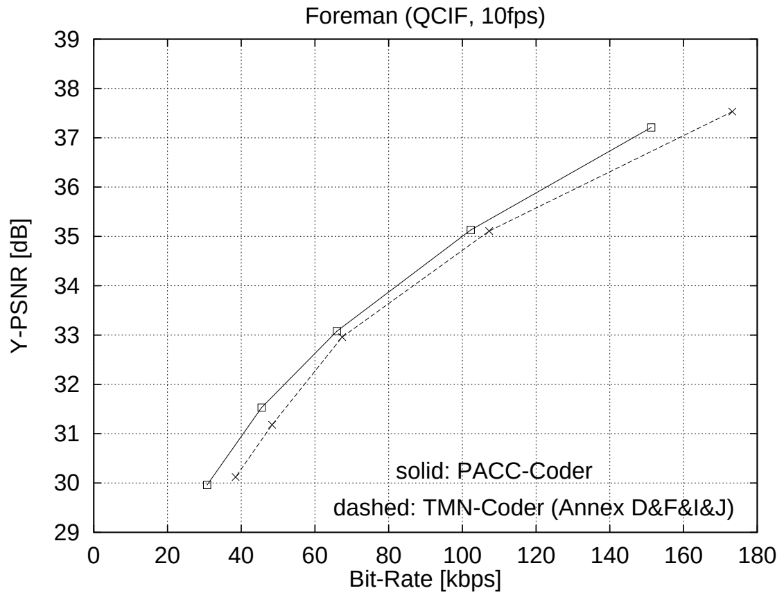
Fig. 14: RD-Comparison of PACC and TMN for FOREMAN.
