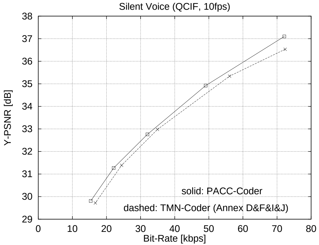
Fig. 15: RD-Comparison of PACC and TMN for SILENT VOICE.
