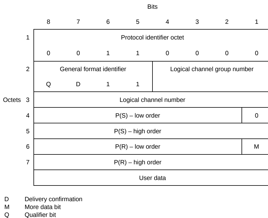
FIGURE 13-2/X.75 Data packet format (modulo 32768)
