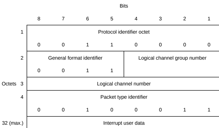
FIGURE 14-2/X.75 Interrupt packet format (modulo 32768)
