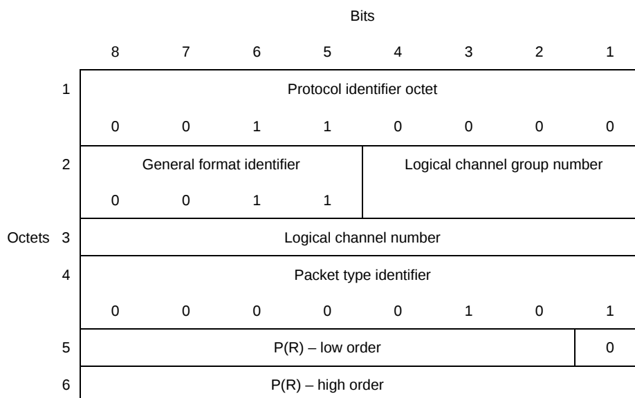
FIGURE 19-2/X.75 RNR packet format (modulo 32768)
