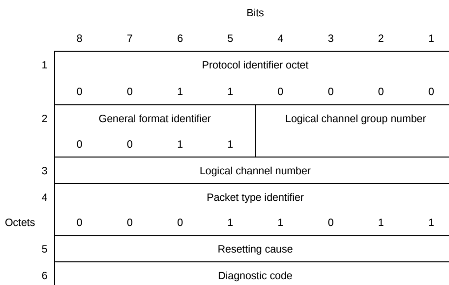
FIGURE 20-2/X.75 Reset request packet format (modulo 32768)
