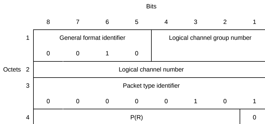
FIGURE 19/X.75 RNR packet format (modulo 128)
