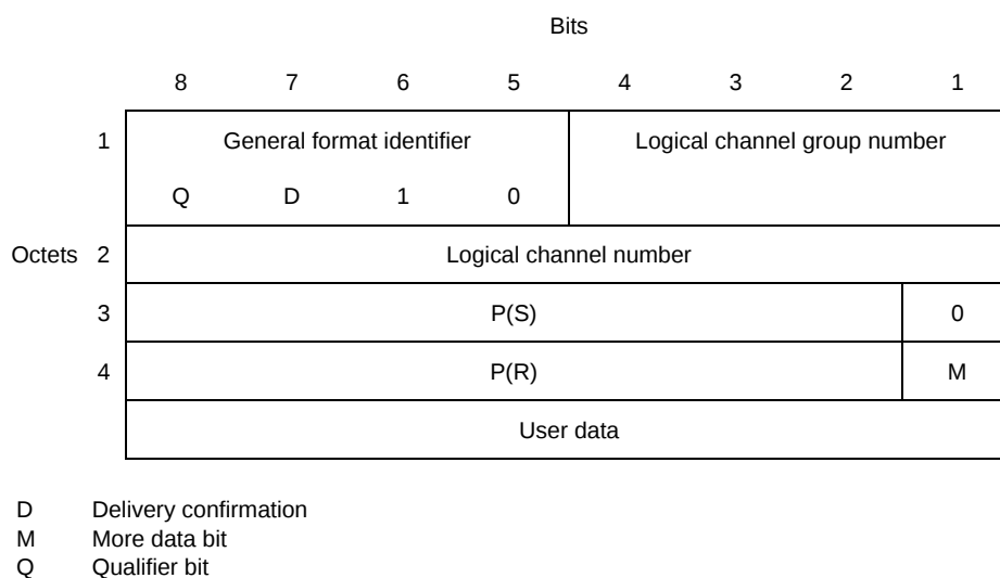
FIGURE 13/X.75 Data packet format (modulo 128)
