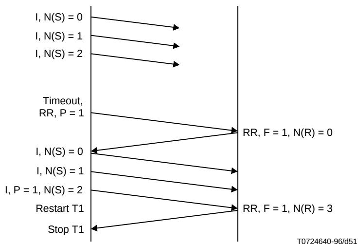
FIGURE IV.3/X.75 I frame recovery, when last few I frames in sequence of I frames are lost
