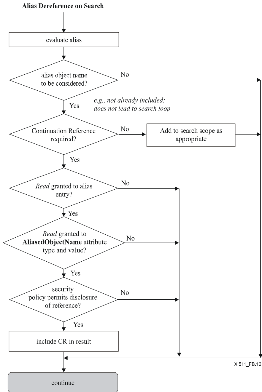
Figure B.10 – Alias Dereference in Search
