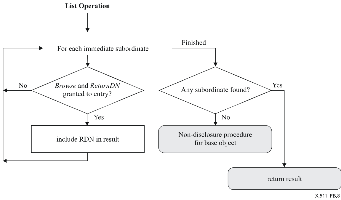
Figure B.8 – List Operation
