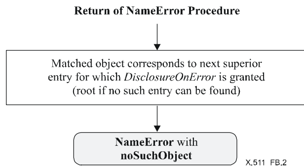
Figure B.2 – Return of Name Error
