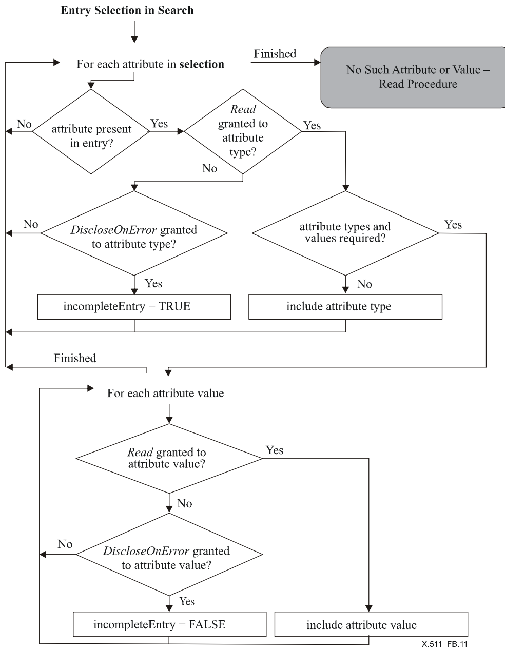
Figure B.11 – Entry Selection in Search
