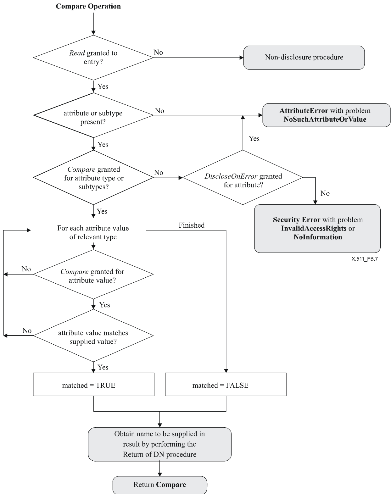
Figure B.7 – Compare Operation
