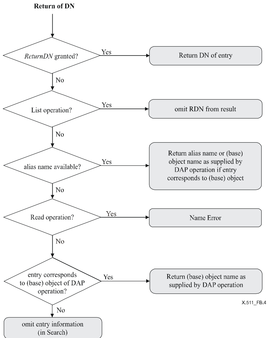
Figure B.4 – Return of Distinguished Name
