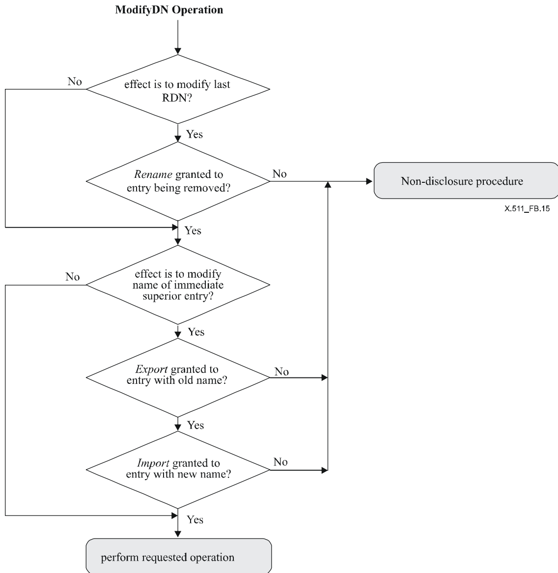
Figure B.15 – ModifyDN Operation
