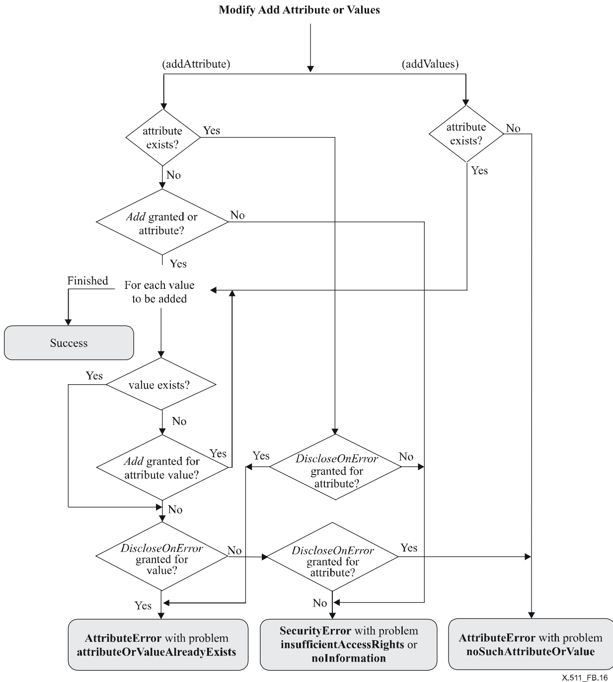
Figure B.16 – Modify Add Attribute or Values
