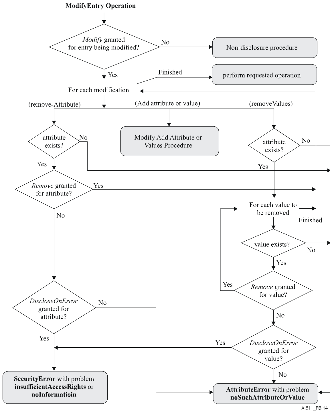
Figure B.14 – Modify Entry Operation
