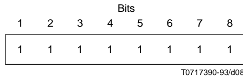
FIGURE 9/X.32 User data identifier element
