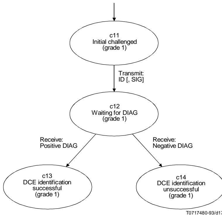
FIGURE A.2/X.32 Diagram of states for DCE acting as challenged party for security grade 1 identification
