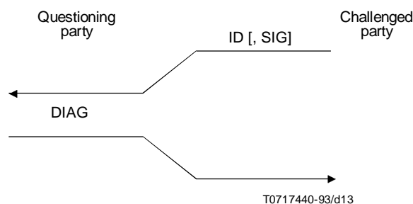
FIGURE 14/X.32 Security grade 1
