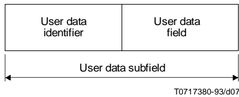
FIGURE 8/X.32 User data subfield
