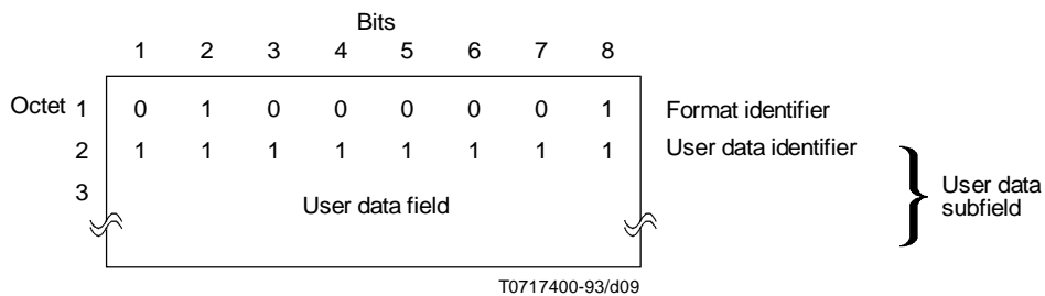
FIGURE 10/X.32 XID information field format
