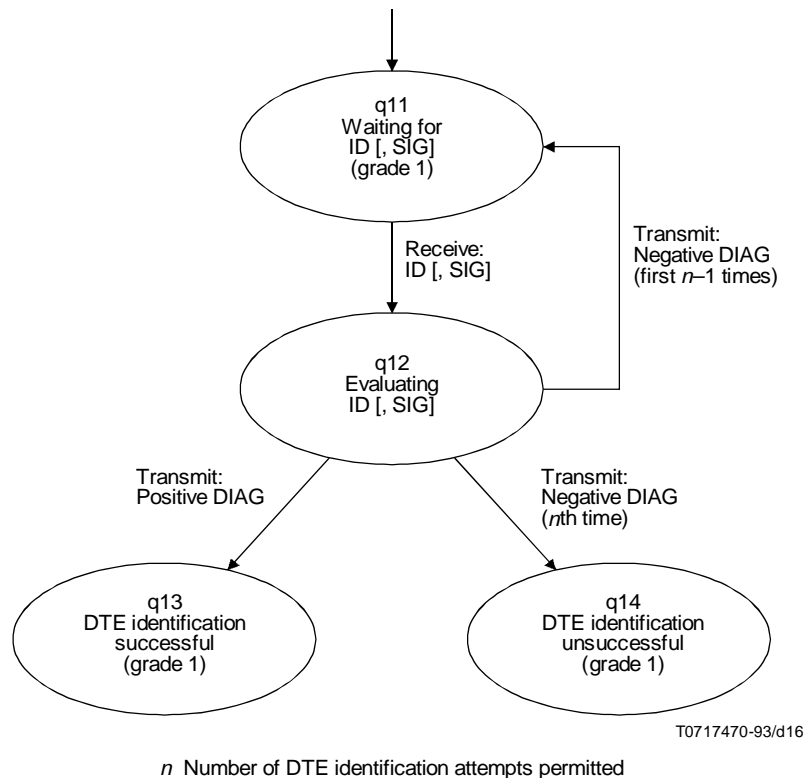
FIGURE A.1/X.32 Diagram of states for DCE acting as questioning party for security grade 1 identification
