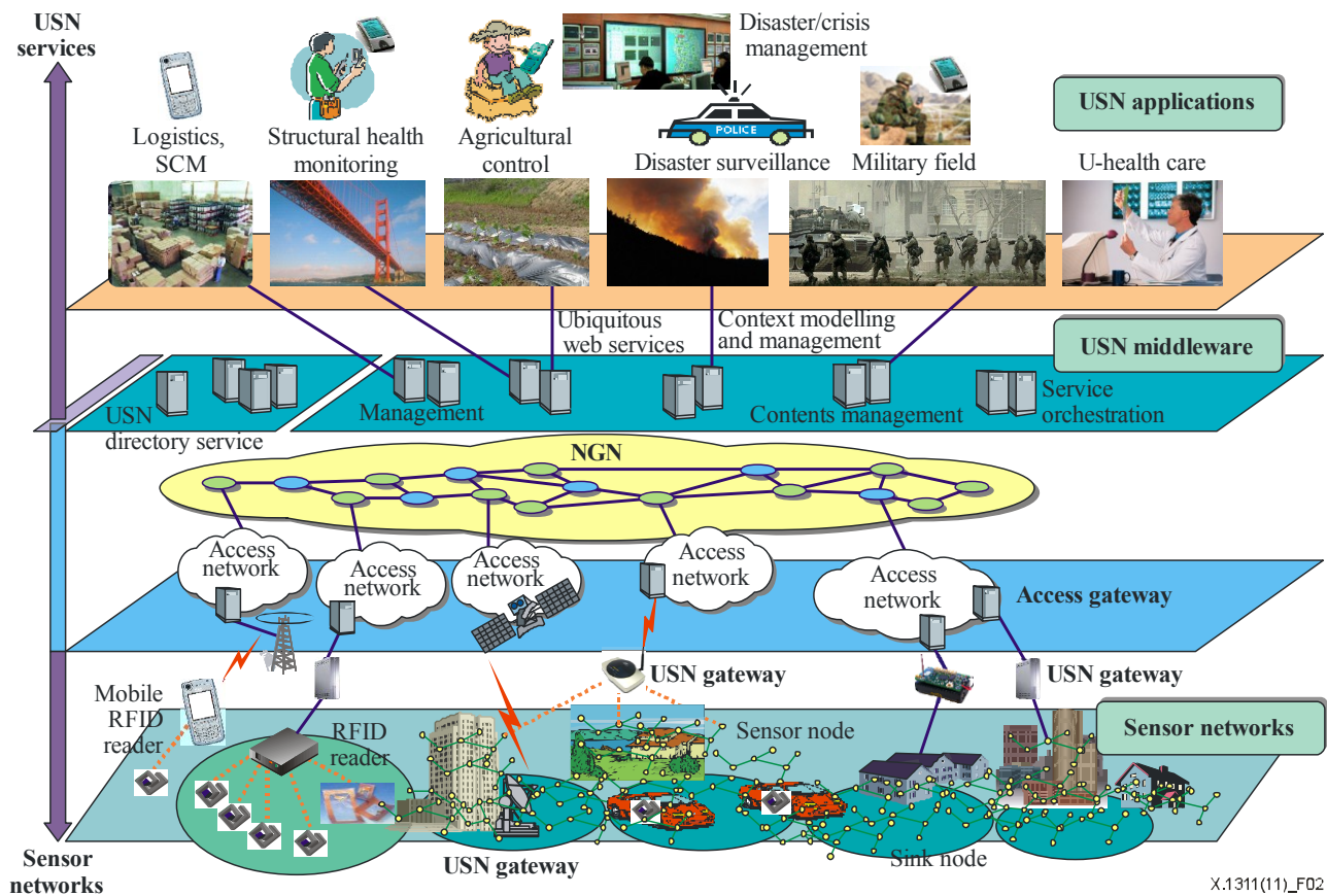
Figure 2 – Overall structure of USN
