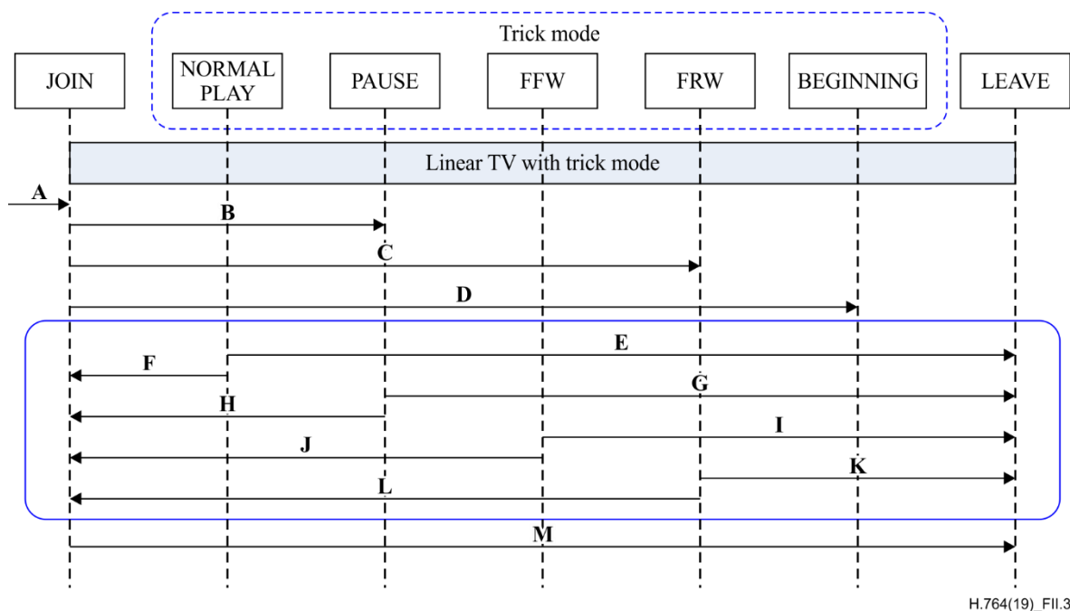
Figure II.3 – State transition for Event object in a linear TV with trick mode scenario
