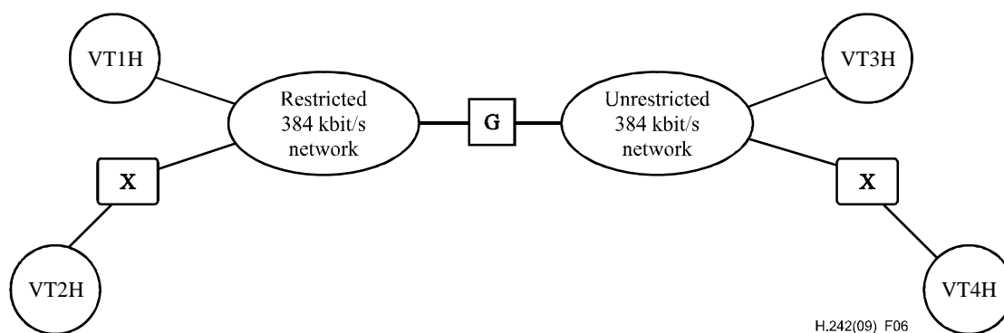
Figure 6 – Unrestricted/restricted 384 kbit/s network
