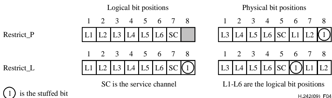
Figure 4 – Restrict_P and Restrict_L modes
