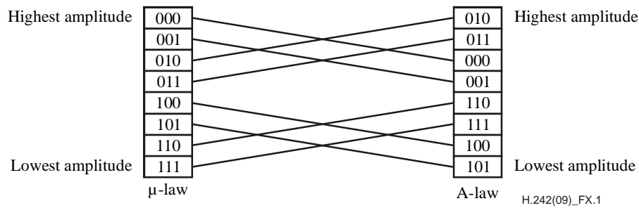
Figure X.1 – Order of segments according to amplitude, \mu -law and A-law PCM
