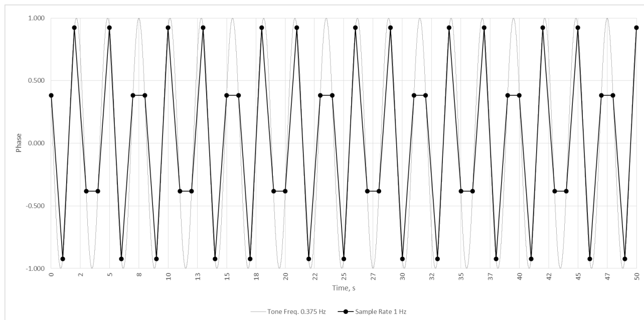
Figure VI.4 – Sub-Nyquist artefact for m = 1 , n = 2 , \epsilon = 0.125 Hz
