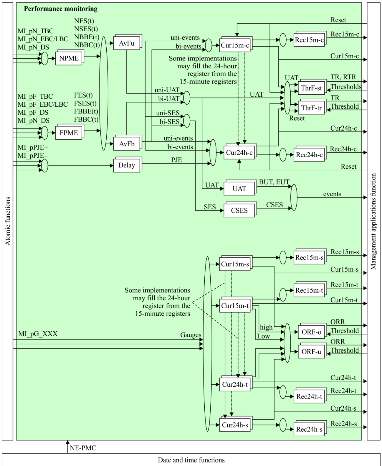
Figure 38 – Performance monitoring inside the EMF
