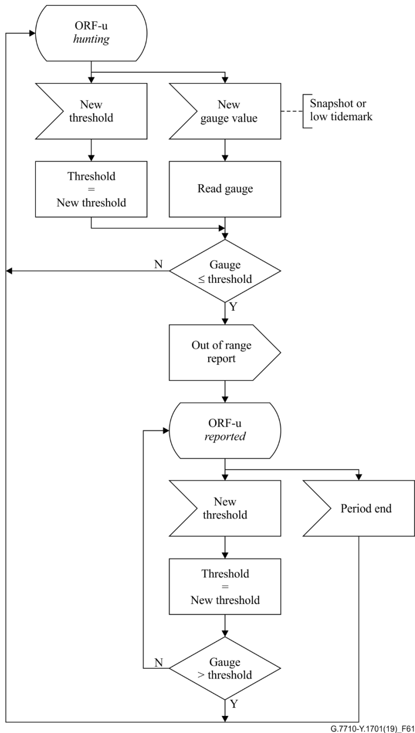
Figure 61 – Out of range function for gauge underflow detection
