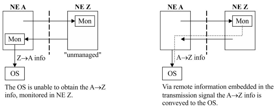
Figure 33 – Single-ended maintenance through far-end monitoring
