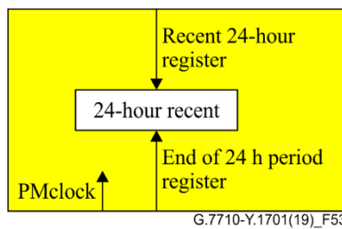
Figure 53 – Rec24h-c, Rec24h-s, Rec24h-t
