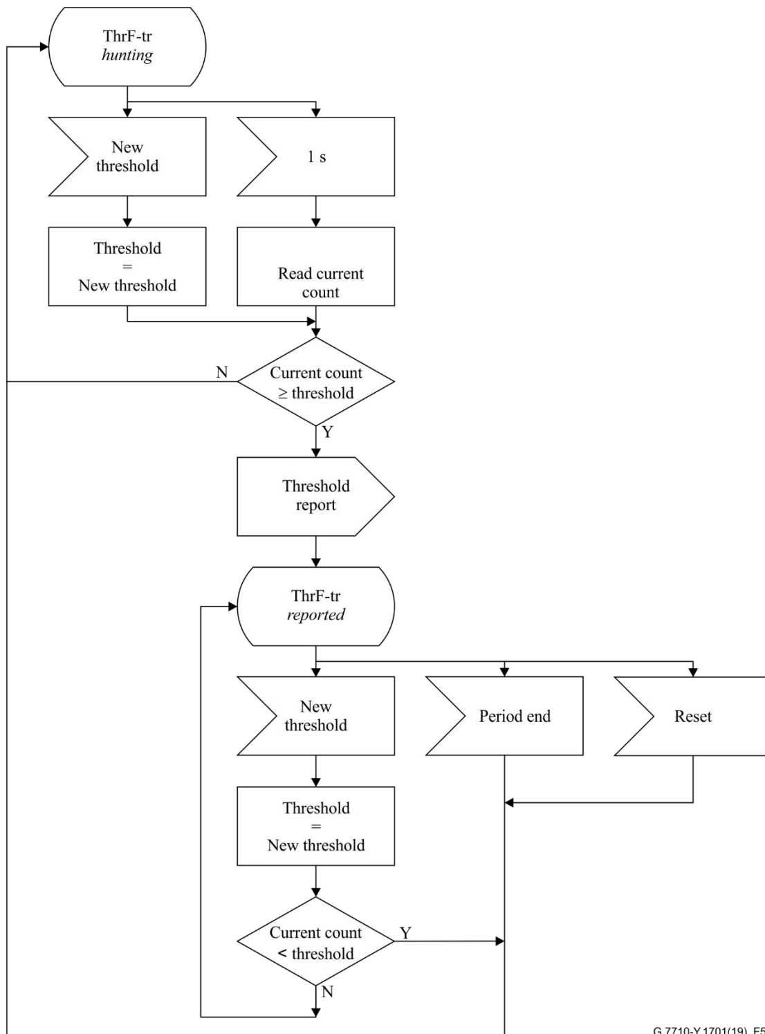
Figure 55 – Transient condition threshold function
