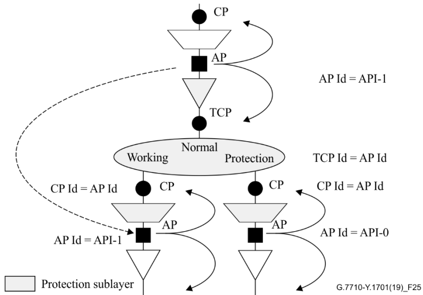
Figure 24 – CP/FP and TCP/TFP identification scheme
