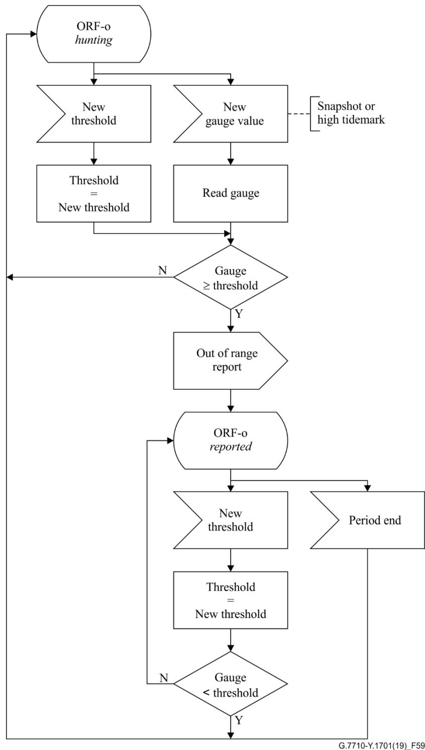
Figure 59 – Out of range function for gauge overflow detection
