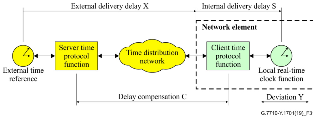
Figure 31 – Local RTC function alignment with an external time reference
