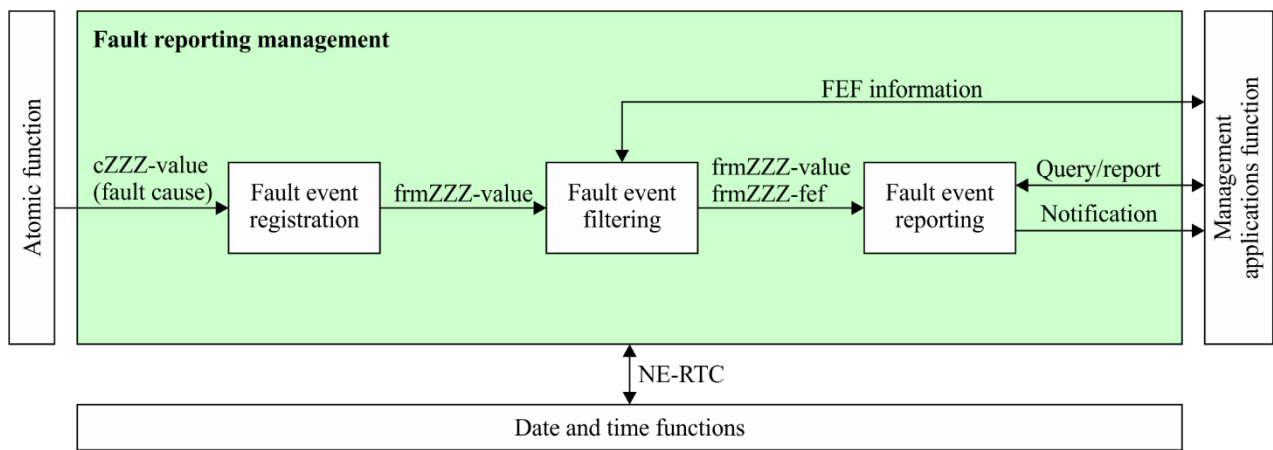
Figure 62 – FRM functional diagram
