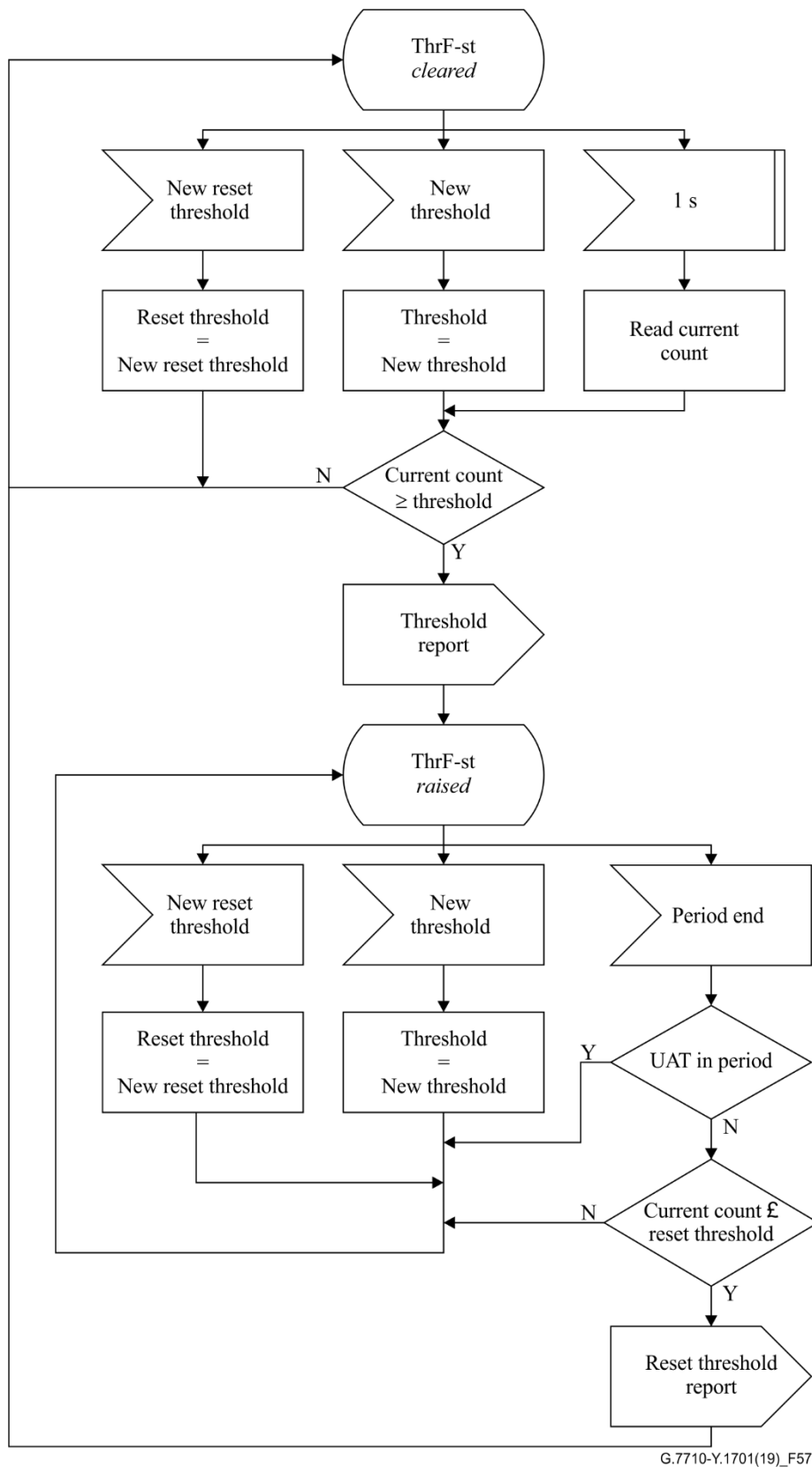
Figure 57 – Standing condition threshold function
