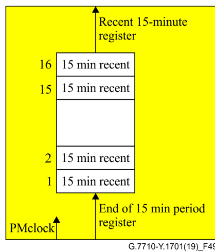
Figure 49 – Rec15m-c, Rec15m-s, Rec15m-t
