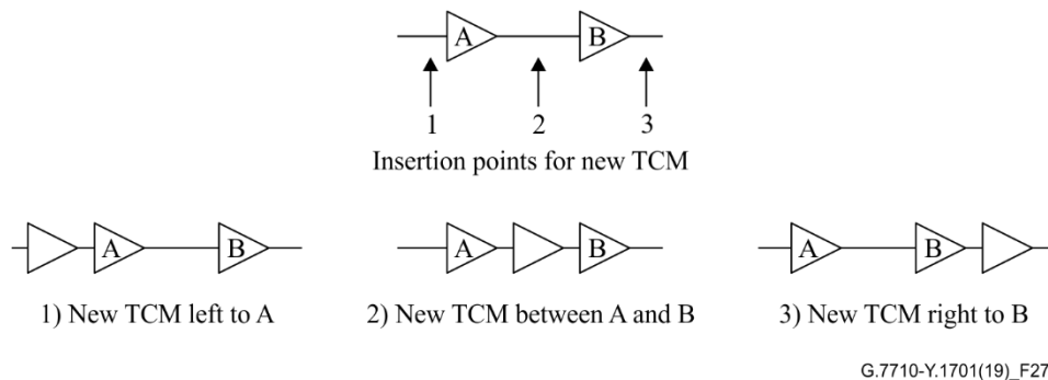
Figure 27 – TCM activation provisioning
