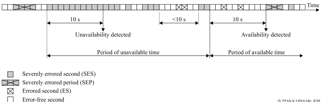
Figure 35 – SDH example of unavailability determination
