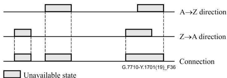
Figure 36 – Example of the unavailable state of a bidirectional connection
