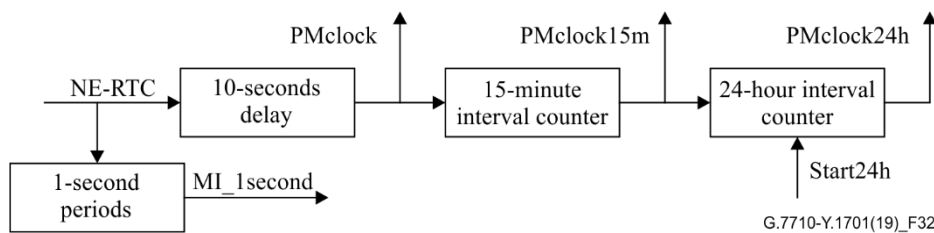
Figure 32 – Performance monitoring clock function
