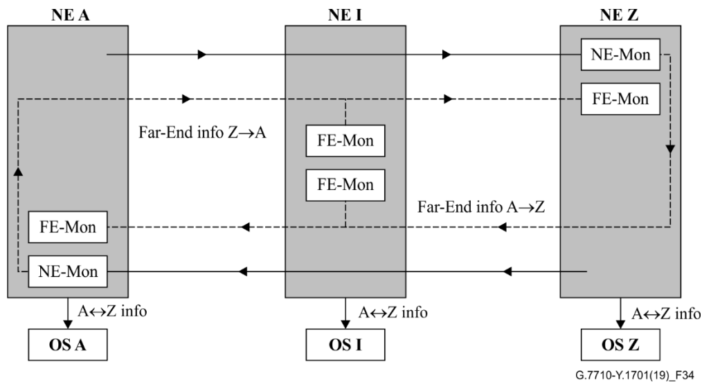
Figure 34 – Single point QoS measurements
