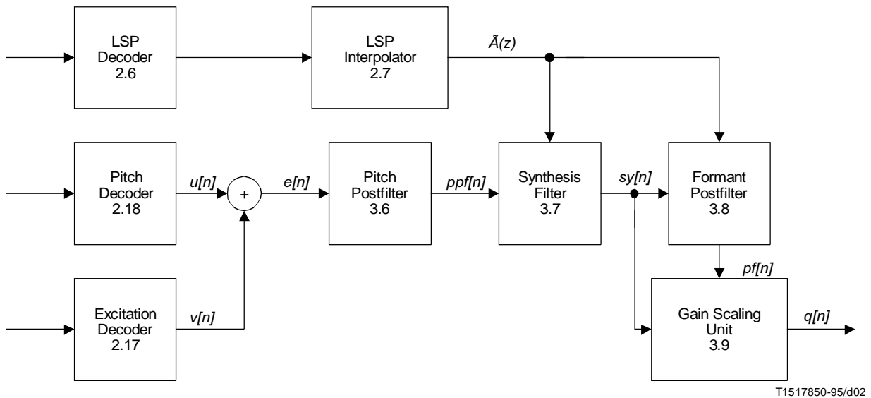
FIGURE 2/G.723.1
