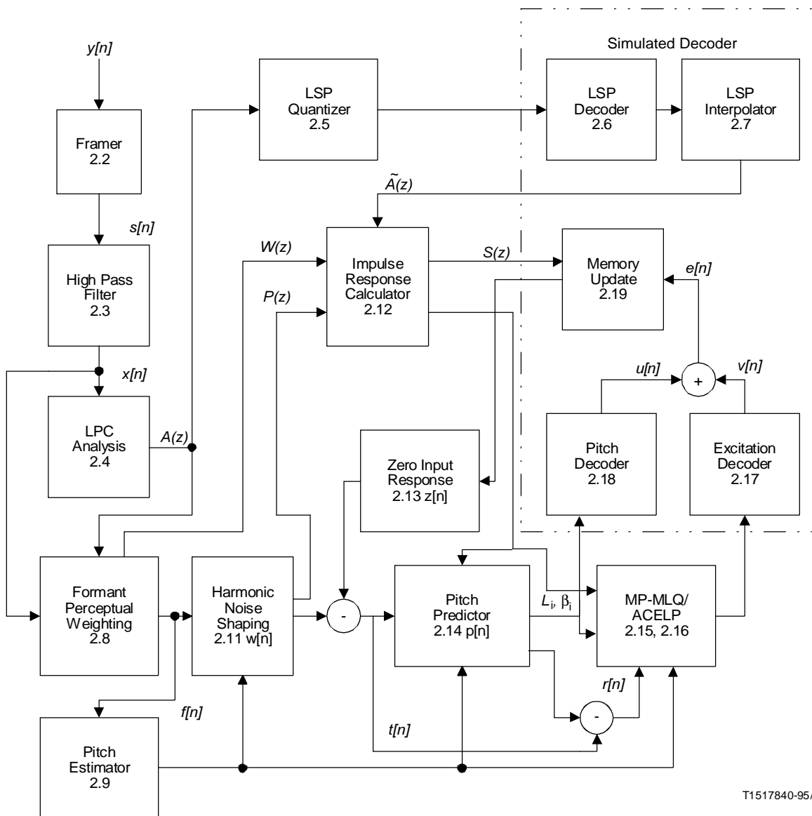
FIGURE 1/G.723.1
