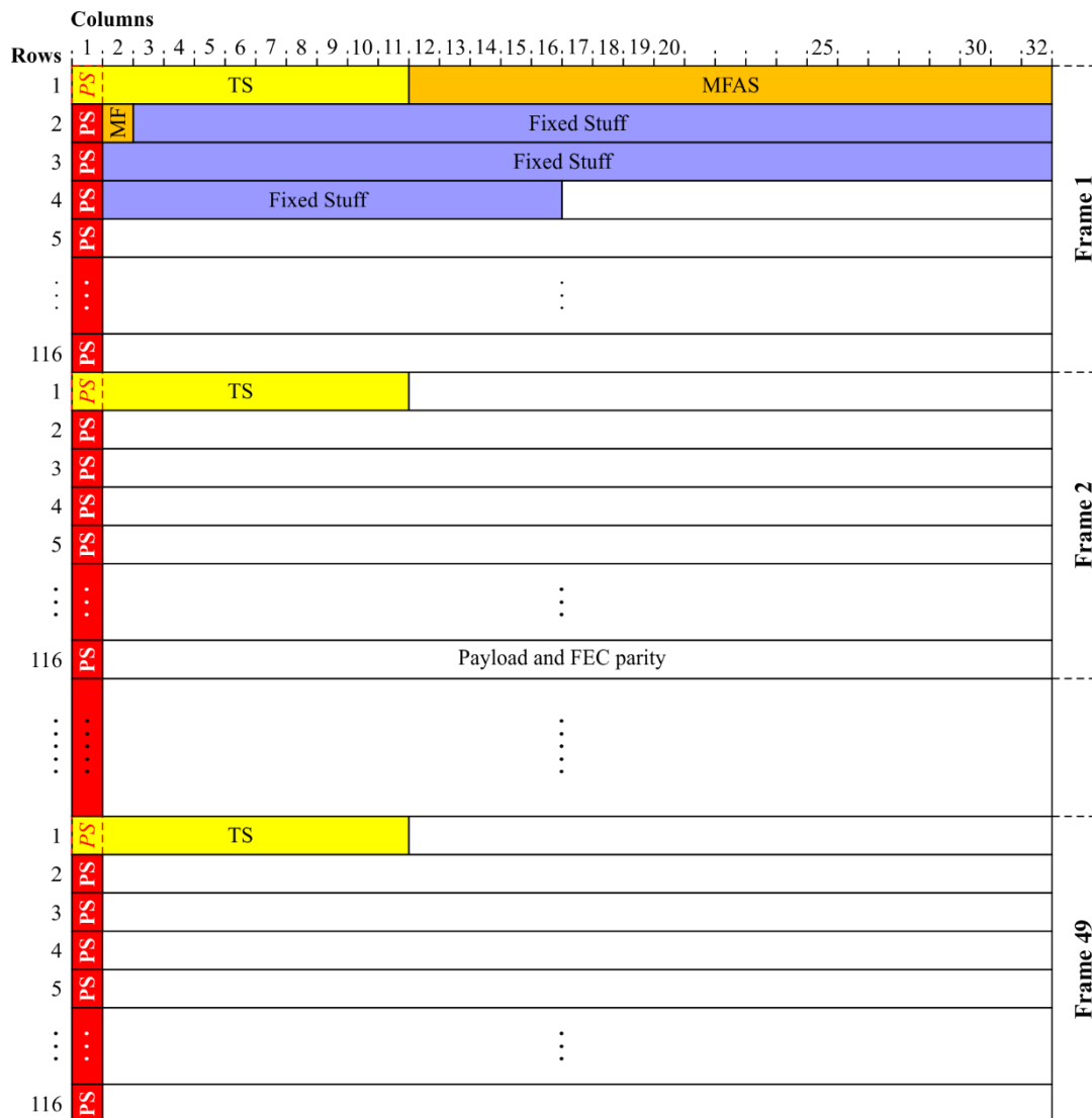
Figure 15-1 – FlexO-x-DSH 49-frame multi-frame structure
