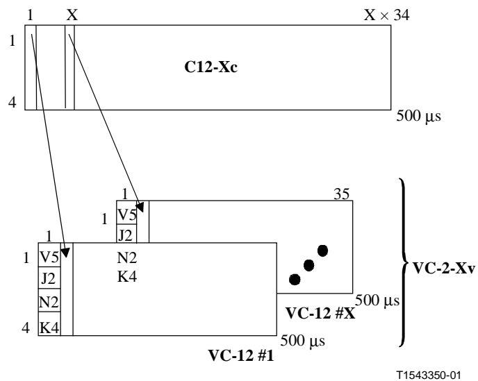
Figure 11-7/G.707/Y.1322 – Structure du conteneur VC-12-Xv
