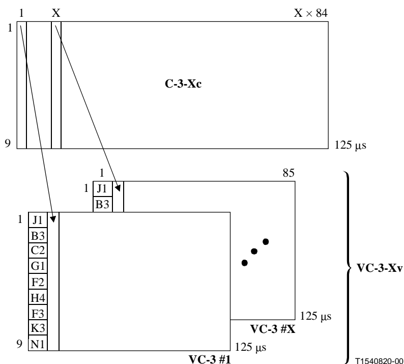
Figure 11-2/G.707/Y.1322 – Structure d'un conteneur VC-3-Xv
