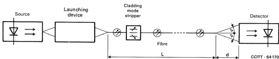
FIGURE B-5/G.651
