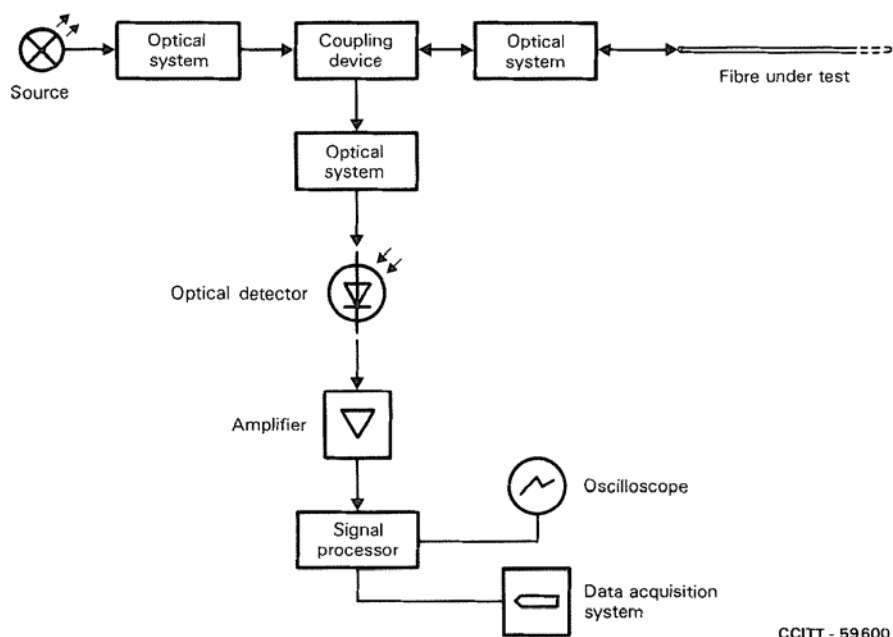
a) Scheme of apparatus
