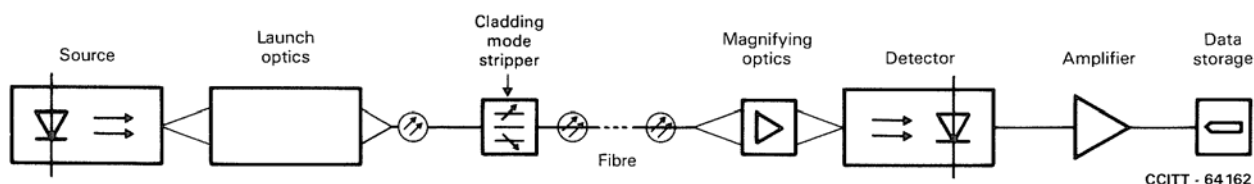
FIGURE B-4/G.651
