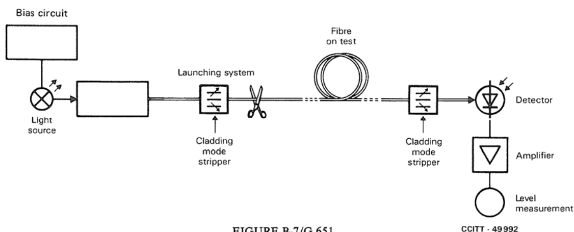
FIGURE B-7/G.651
