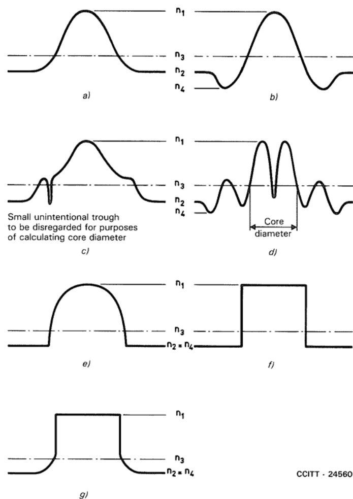
FIGURE A-1/G.651
