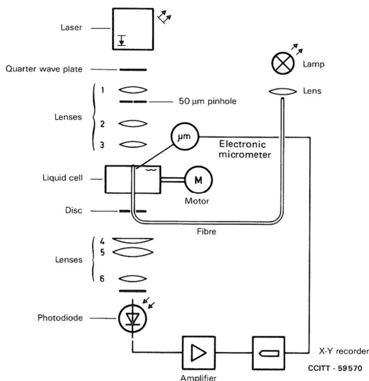
FIGURE B-3/G.651
