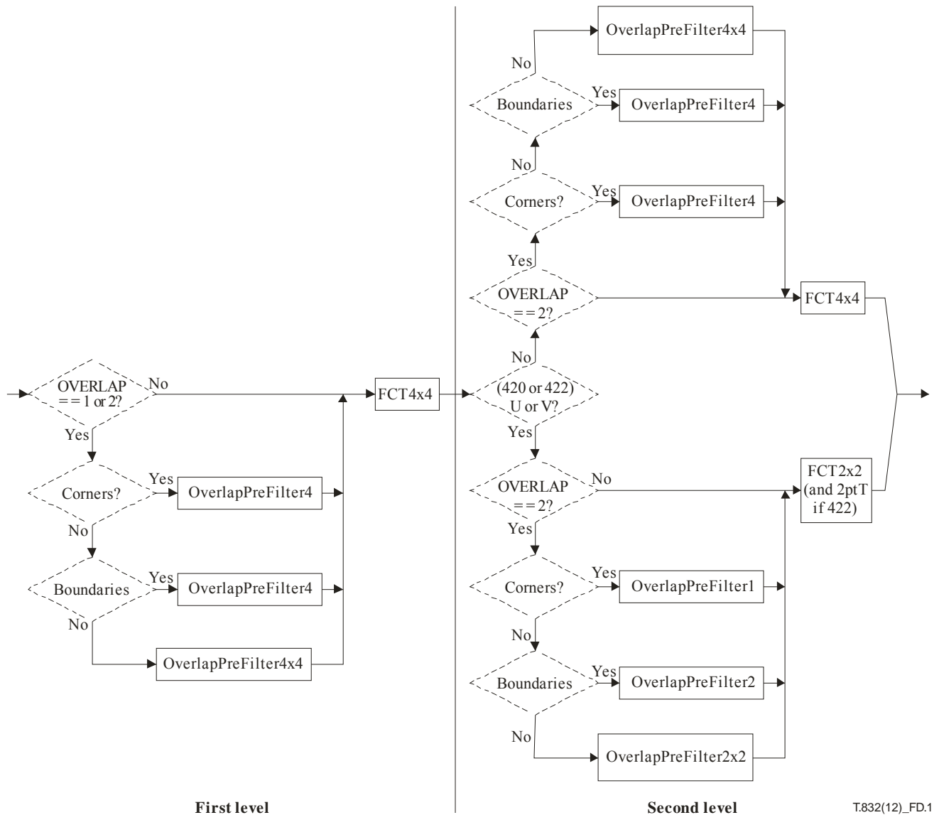
Figure D.1 – Encoder transform
