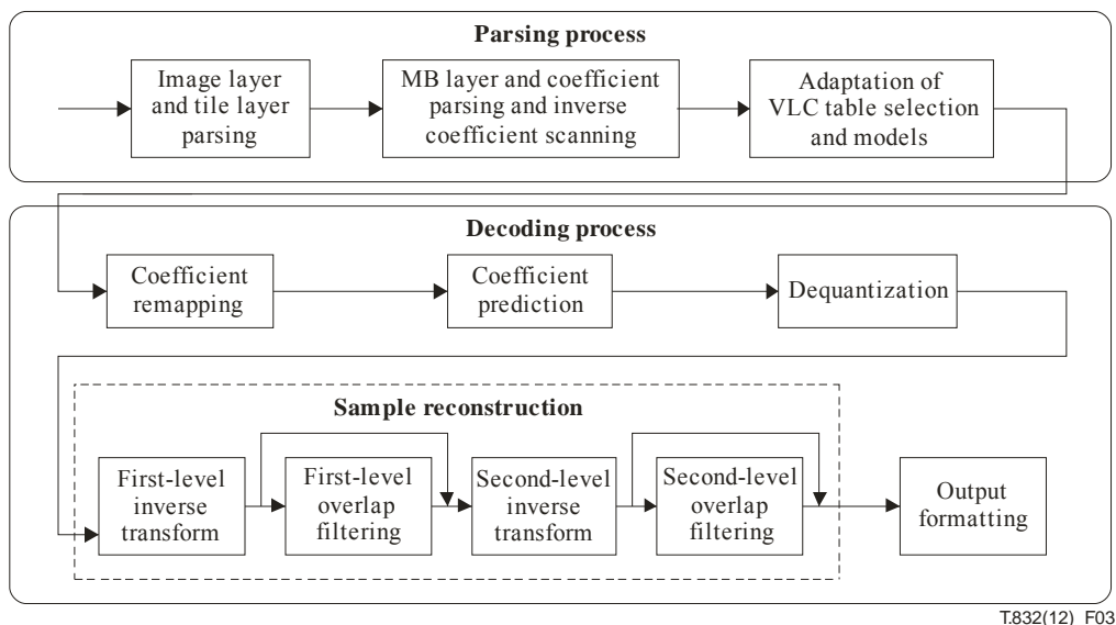
Figure 3 – Informative decoding process block diagram
