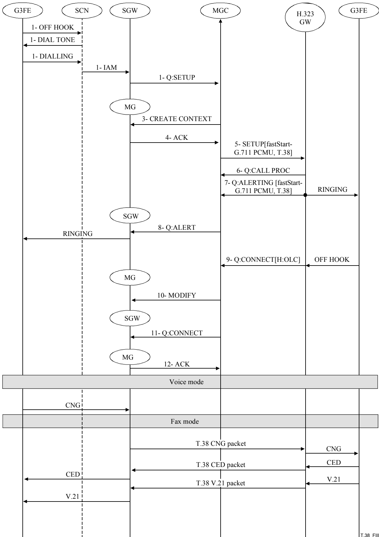
Figure III.4/T.38 – Voice to fax call setup with H.248 and H.323 endpoints that support T.38 Autonomous Transition between VoIP and FoIP
