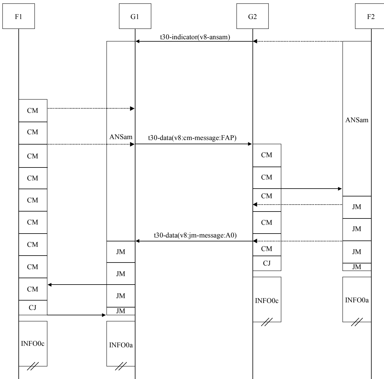
Figure IV.1/T.38 – V.8 signalling (using profiles and acks)
