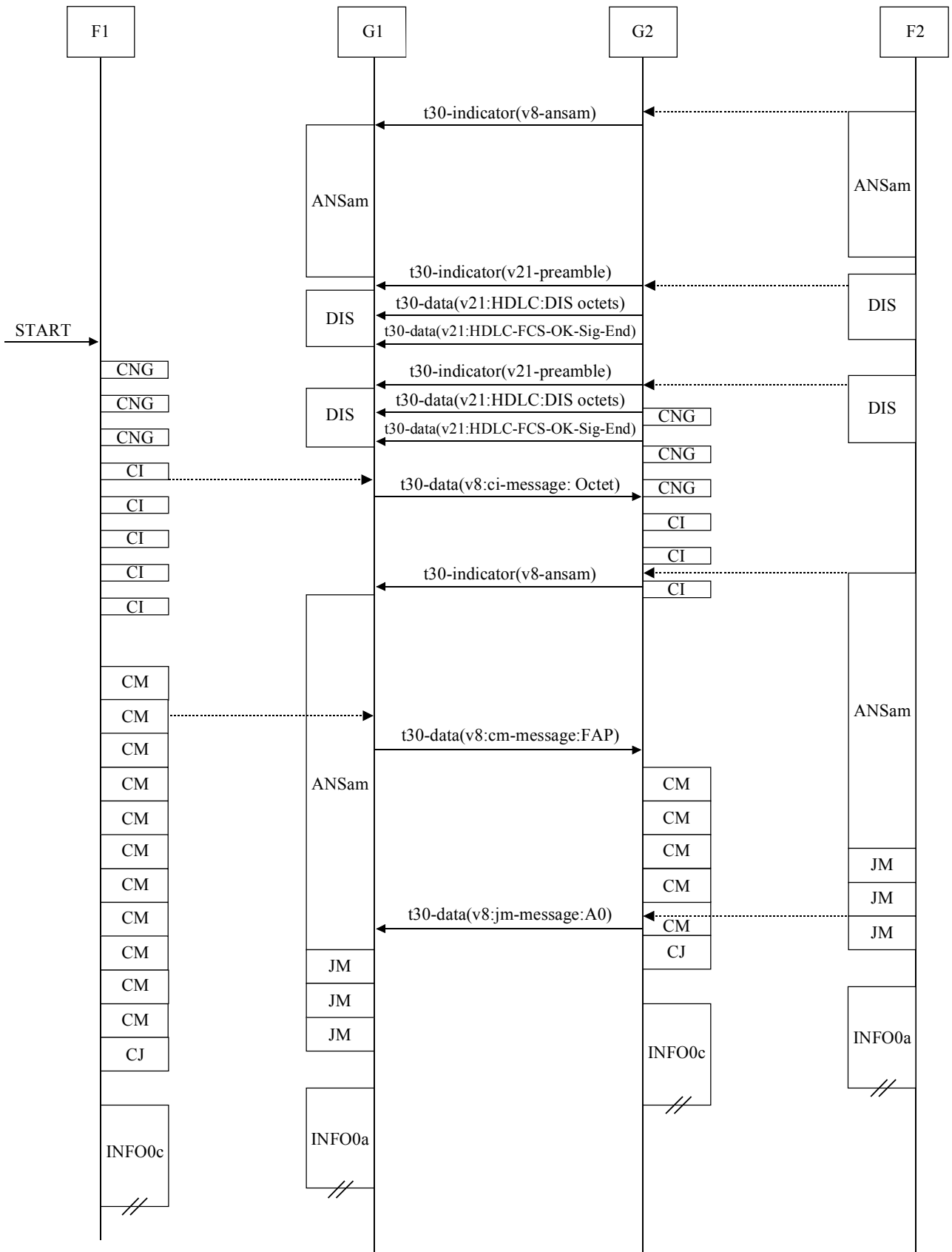
Figure IV.10/T.38 – Manual Transmit (DIS has bit 6 set to 1 to indicate V.8 capability)
