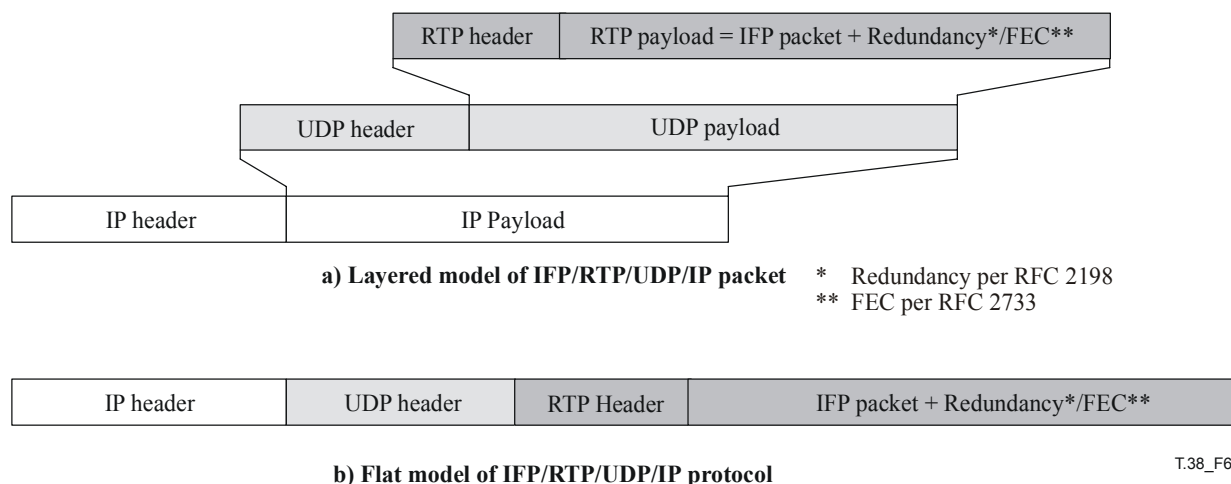
Figure 6/T.38 – High-level RTP/UDP/IP packet structure
