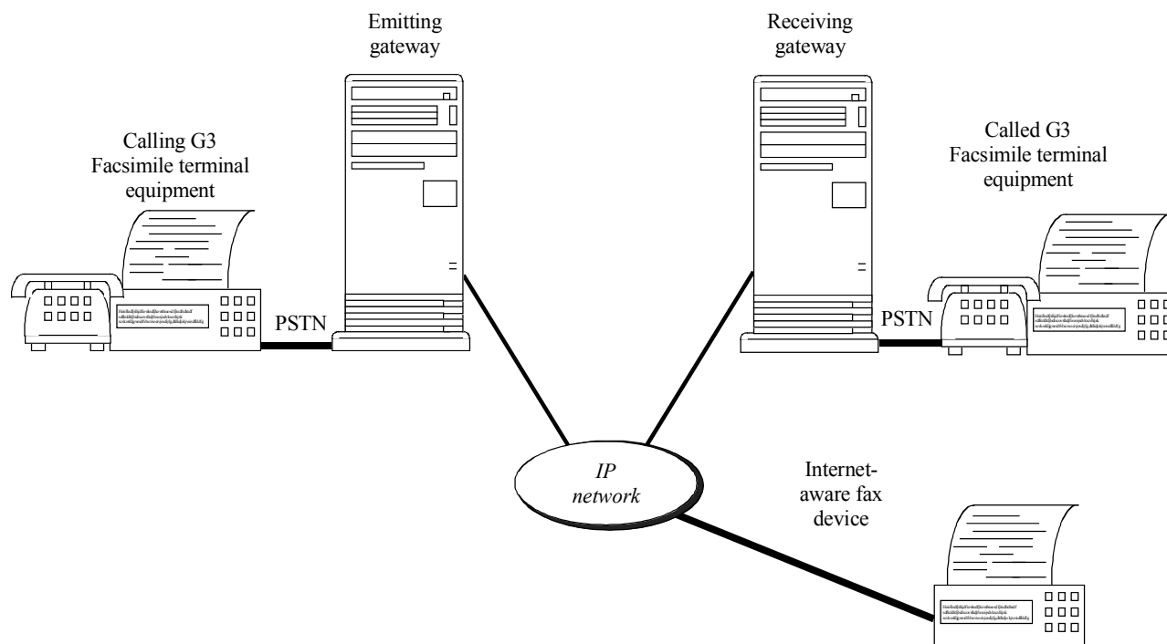
Figure 1/T.38 – Model for facsimile transmission over IP Networks
