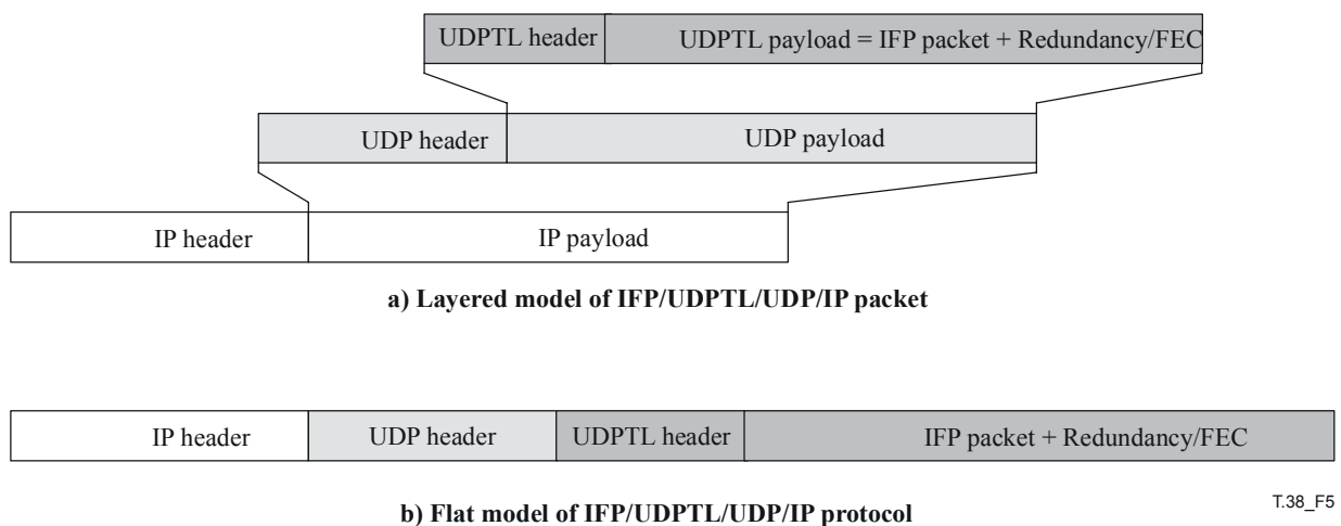
Figure 5/T.38 – High-level UDPTL/UDP/IP packet structure
