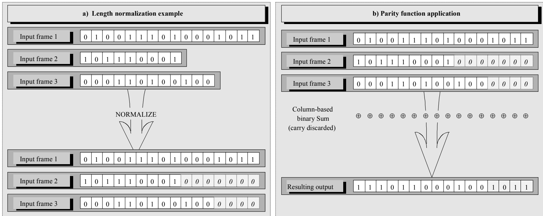
Figure C.1/T.38 – Illustration of Length normalization and Parity function operation
