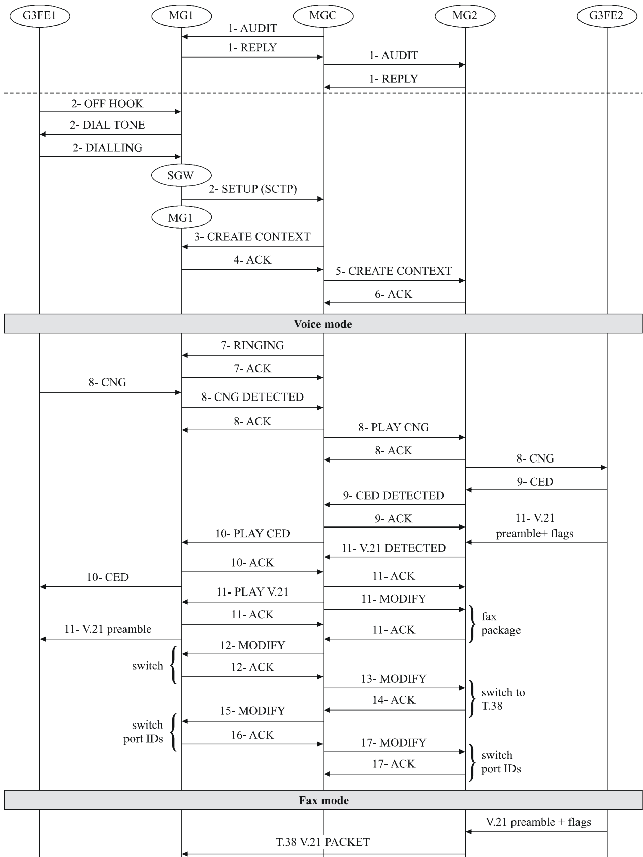
Figure III.1/T.38 – Voice to fax call setup with H.248 endpoints
