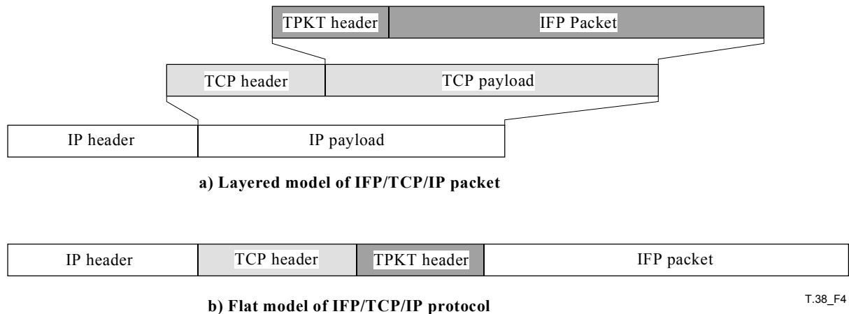
Figure 4/T.38 – High-level TCP/TPKT/IP packet structure
