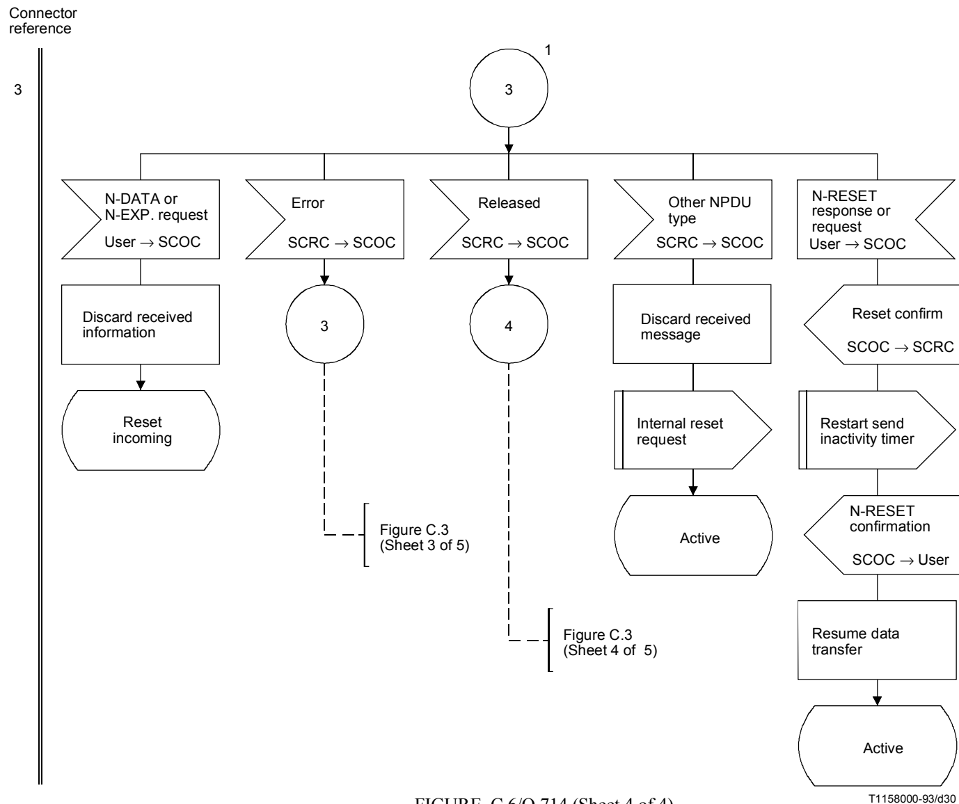
FIGURE C.6/Q.714 (Sheet 4 of 4) Reset procedures at originating and destination node for SCCP connection-oriented control (SCOC)
