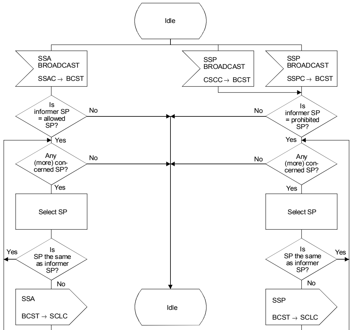
FIGURE D.10/Q.714
