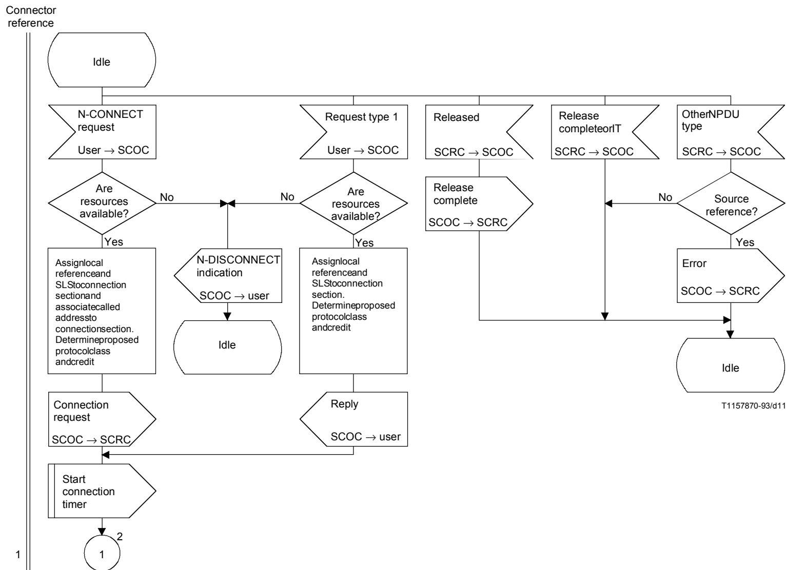
FIGURE C.2/Q.714 (sheet 1 of 6)
