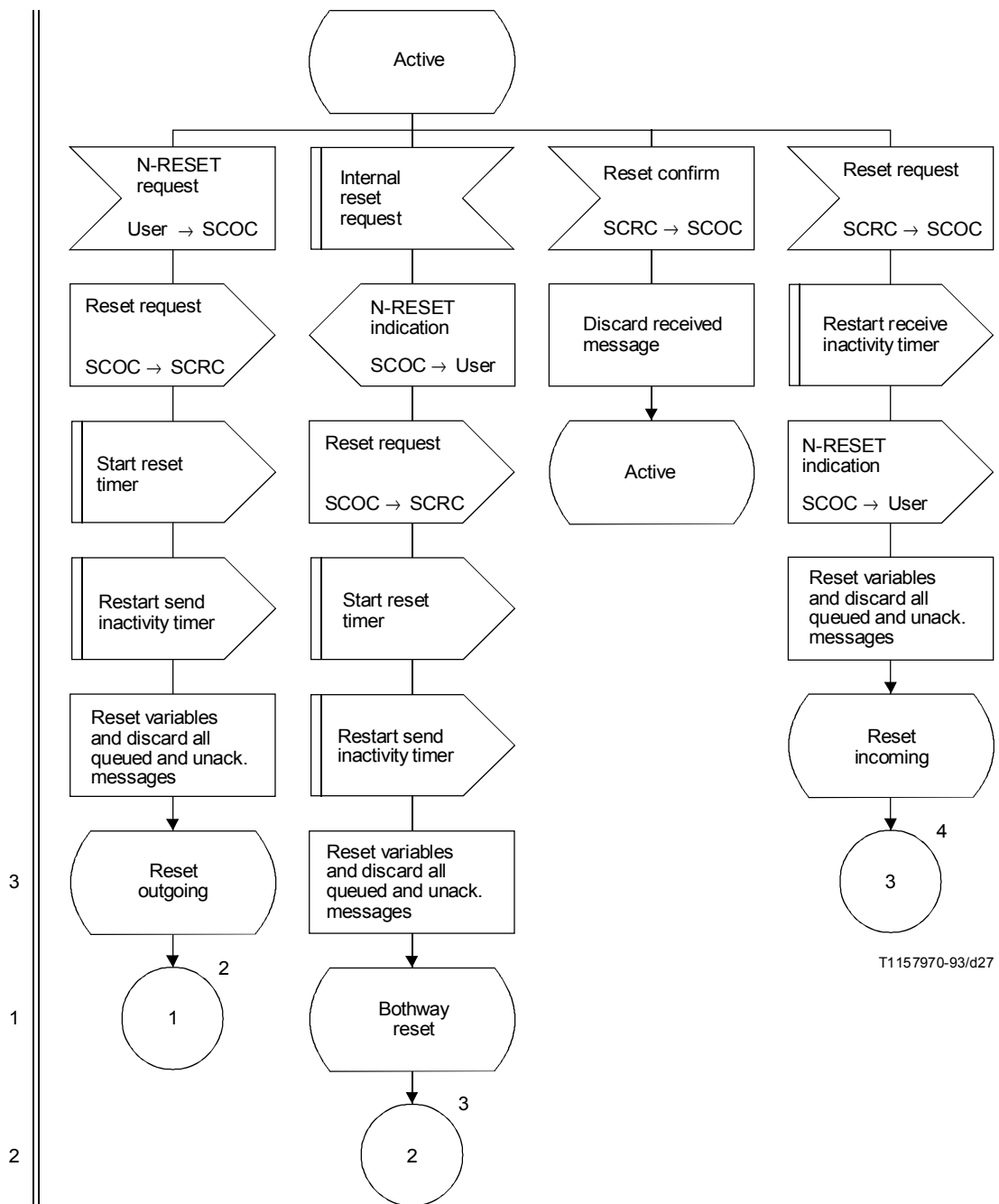
FIGURE C.6/Q.714 (Sheet 1 of 4)
