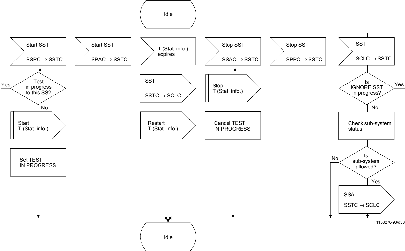
FIGURE D.7/Q.714 Sub-system Status Test Control (SSTC)
