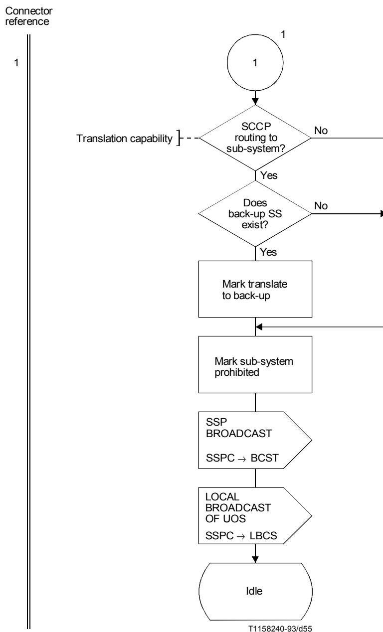
FIGURE D.5/Q.714 (Sheet 2 of 2) Sub-system prohibited control (SSPC)
