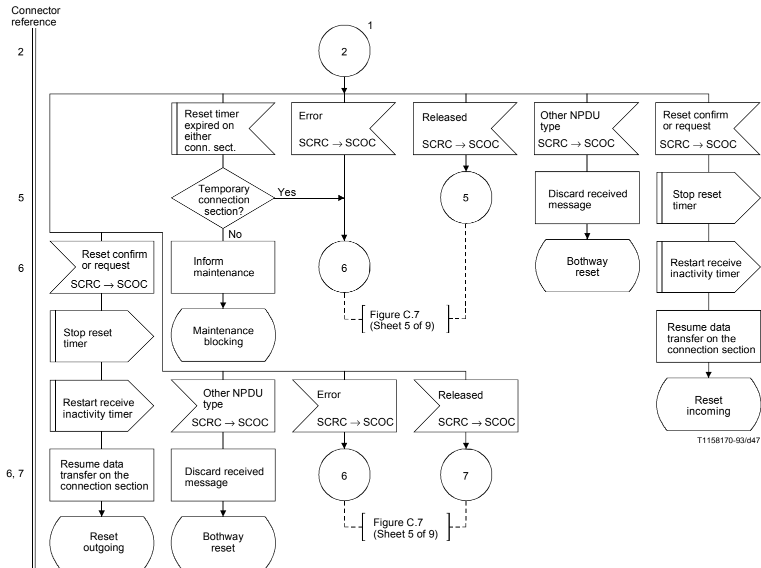
FIGURE C.10/Q.714 (Sheet 3 of 4)
