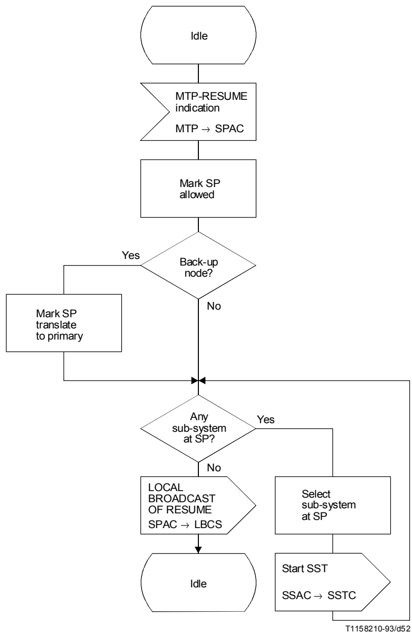
FIGURE D.3/Q.714 Signalling point allowed control (SPAC)
