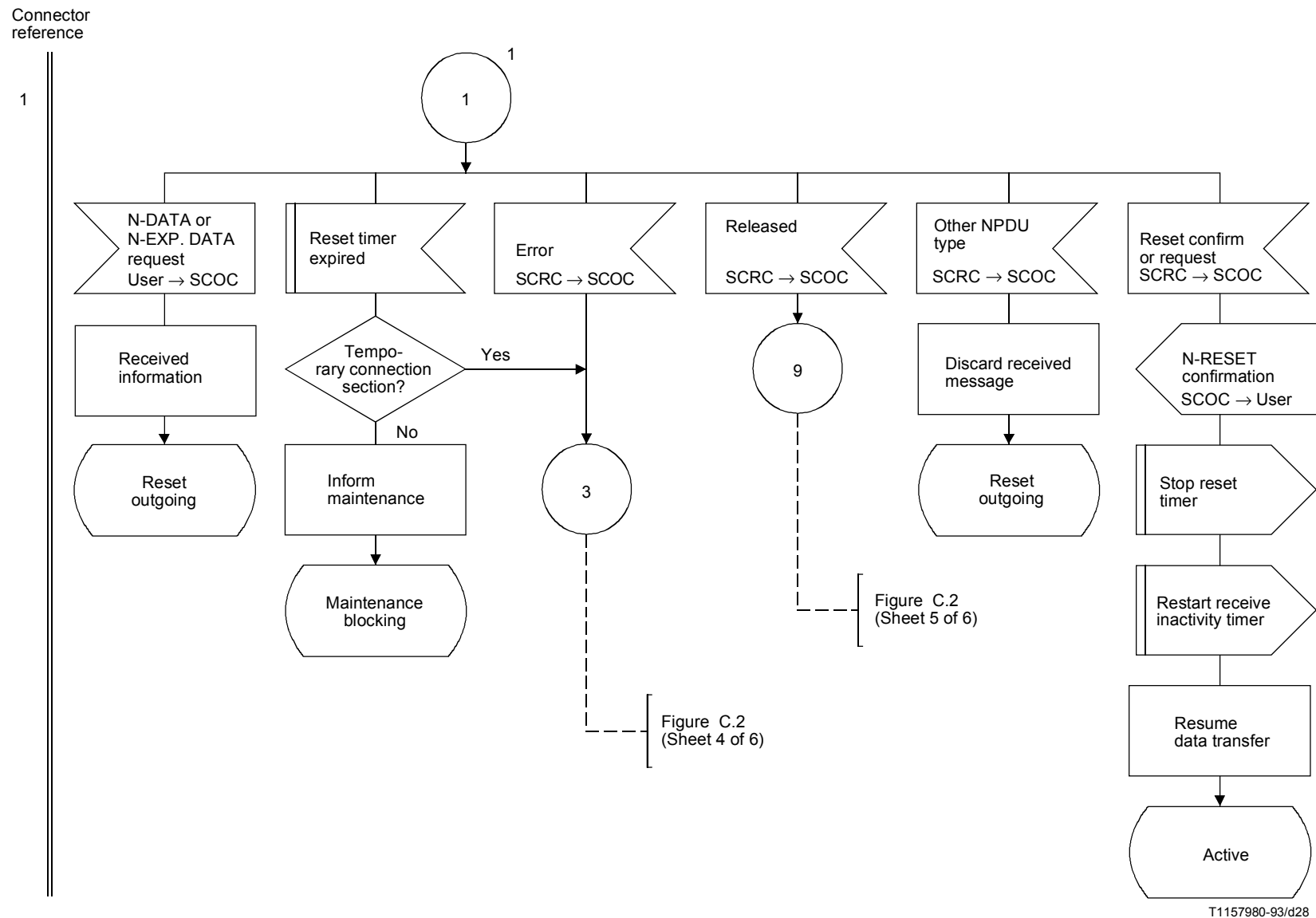
FIGURE C.6/Q.714 (Sheet 2 of 4) Reset procedures at originating and destination node for SCCP connection-oriented control (SCOC)
