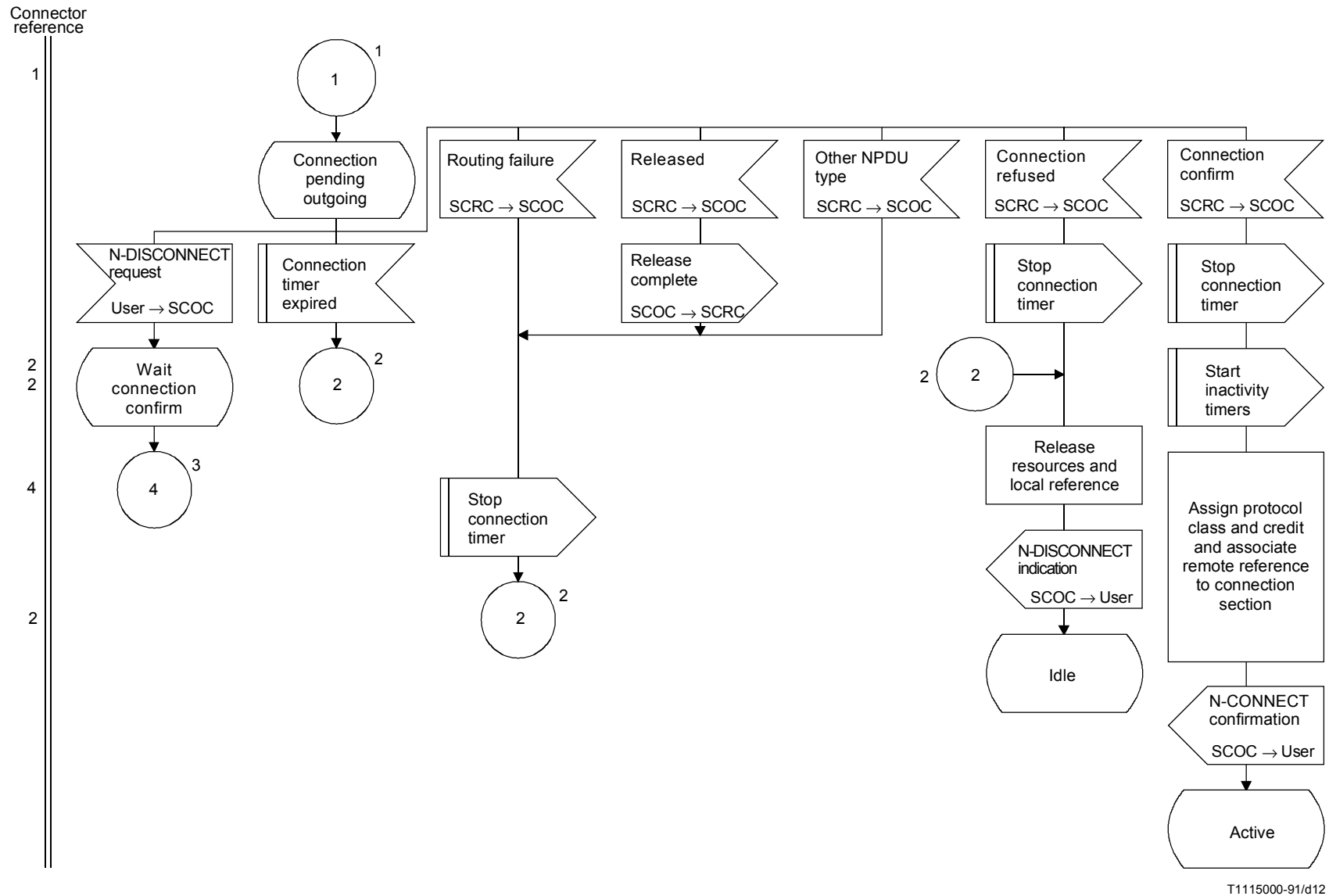
FIGURE C.2/Q.714 (sheet 2 of 6) Connection establishment procedures at originating node for SCCP connection-oriented control (SCOC)
