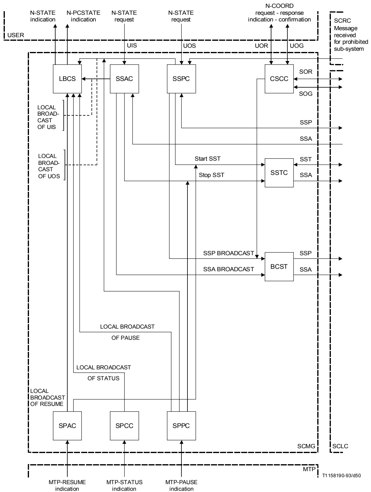
FIGURE D.1/Q.714 SCCP management overview (SCMG)
