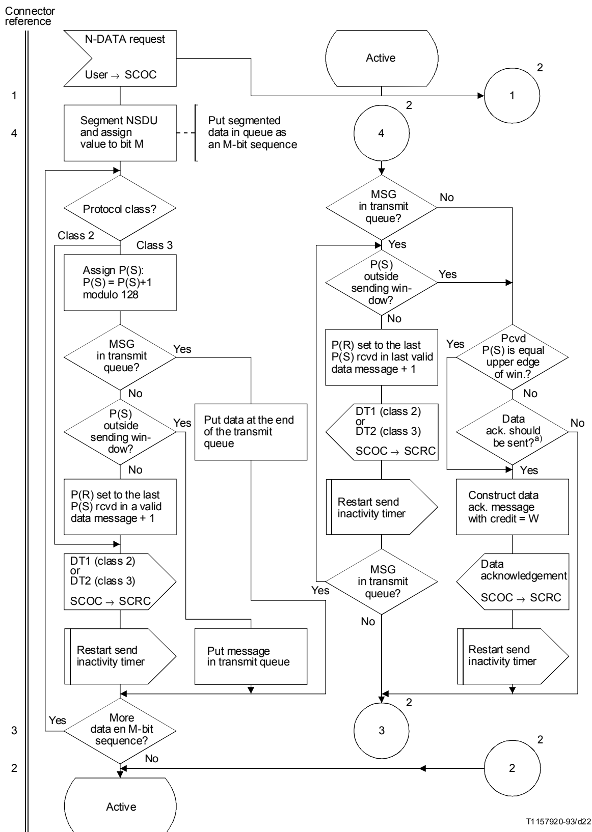
FIGURE C.4/Q.714 (Sheet 1 of 4)
