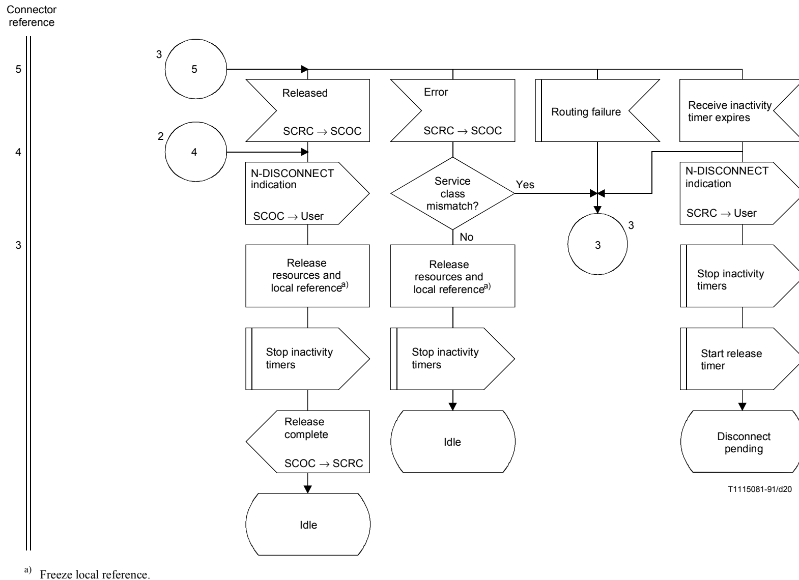
FIGURE C.3/Q.714 (sheet 4 of 5) Connection release procedures at destination node for SCCP connection-oriented control (SCOC)
