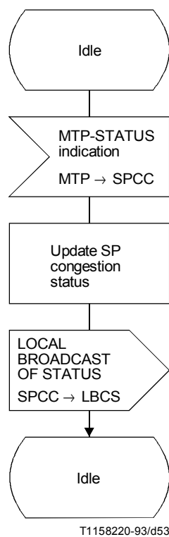
FIGURE D.4/Q.714 Signalling point congested control (SPCC)
