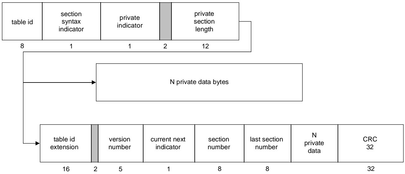
Figure F.6 – Private section diagram
