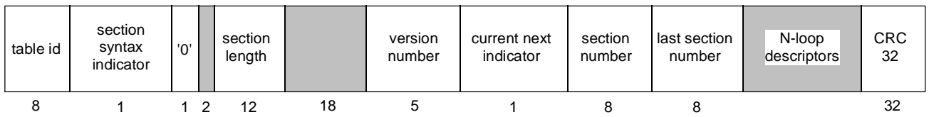
Figure F.4 – Conditional Access section diagram
