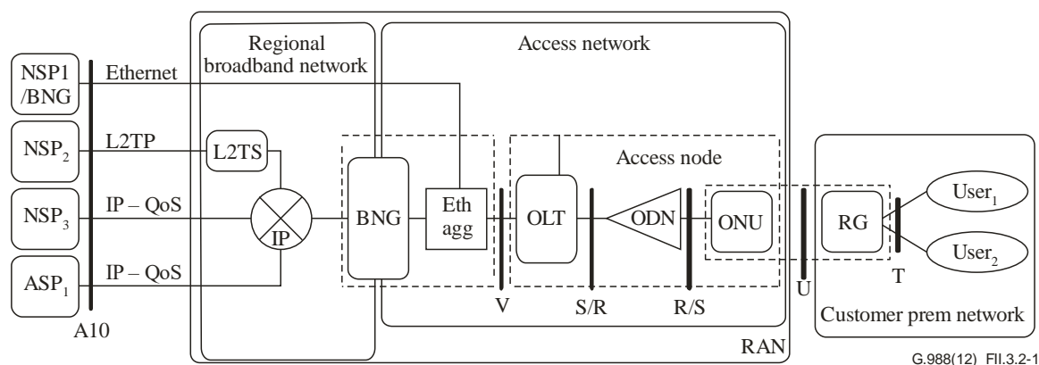
Figure II.3.2-1 – High-level architecture
