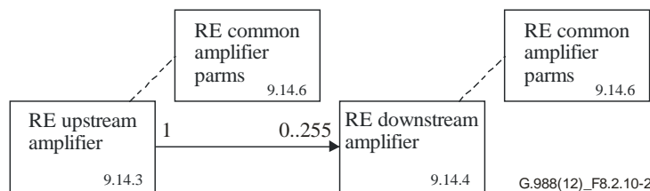
Figure 8.2.10-1 – Mid-span PON reach extender core (repeater)
