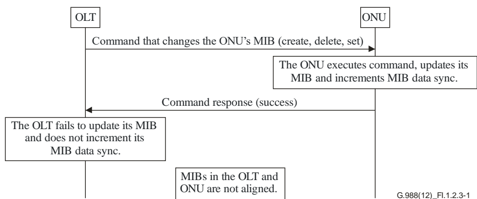
Figure I.1.2.3-1 – Mismatch of MIBs at the ONU and OLT under OLT command
