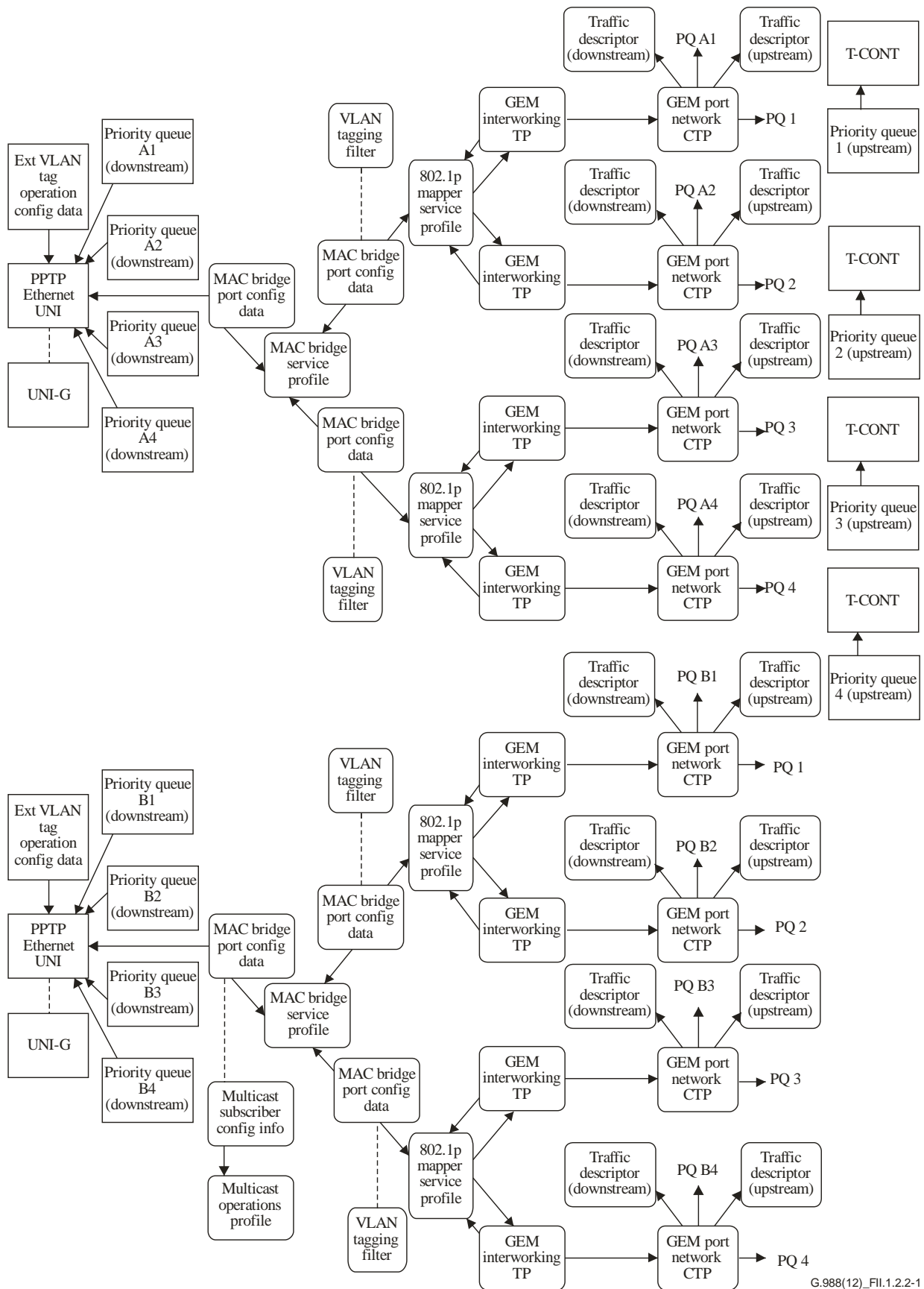
Figure II.1.2.2-1 – Multi-UNI L2-OCM
