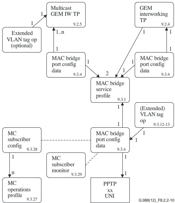
Figure 8.2.2-10 – Illustration of a multicast service
