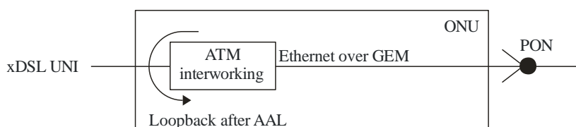
Figure 9.13.4-1 – AAL loopback configuration
