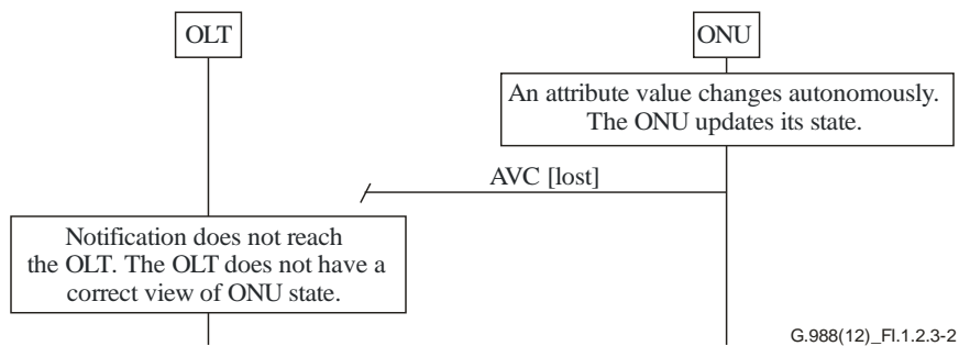
Figure I.1.2.3-2 – Lost AVC
