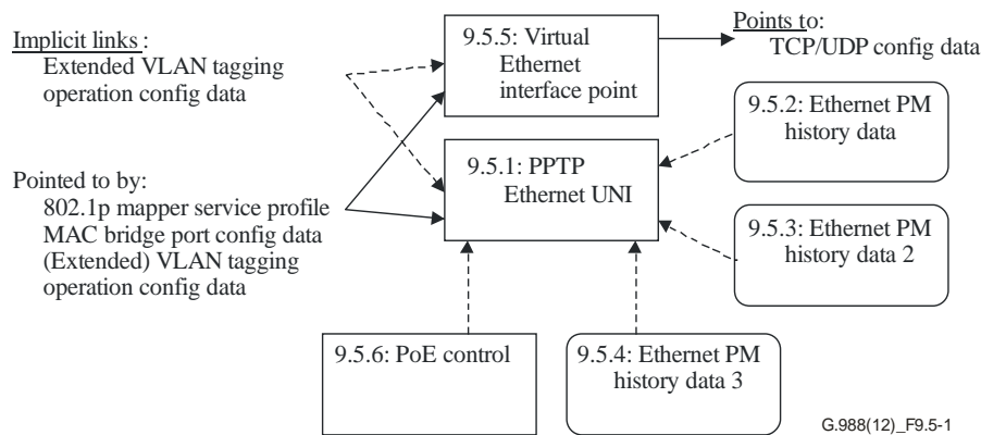
Figure 9.5-1 – Managed entities associated with Ethernet UNIs
