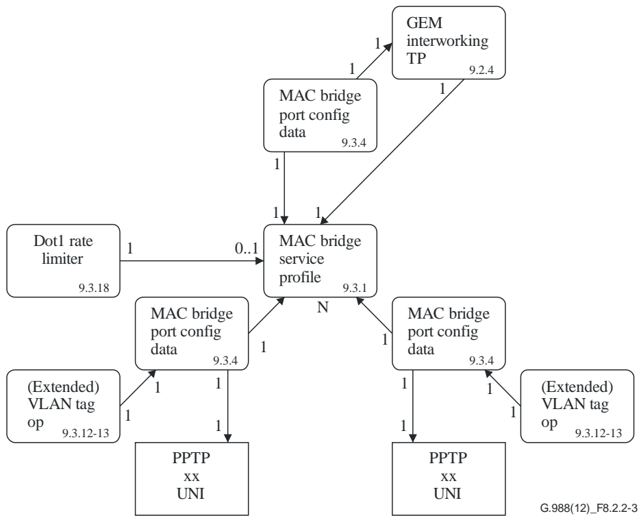
Figure 8.2.2-3 – Illustration of N:1 bridging
