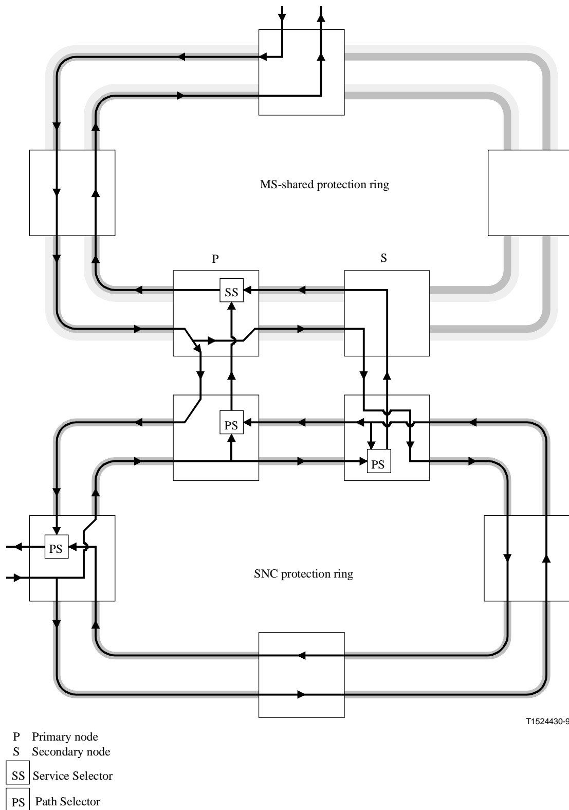
Figure 11/G.842 – Ring interworking between an MS-shared protection ring and a HO SNCP ring
