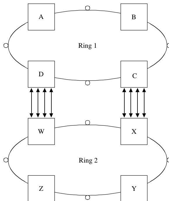
Figure 3/G.842 – Example of dual node interconnection
