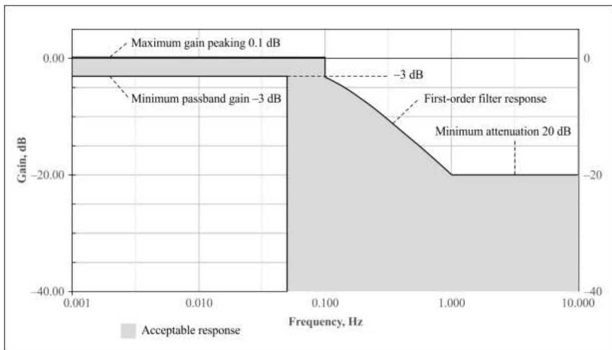
Figure VI.5 – Frequency response of acceptable PTP filter implementation (Classes A, B and C)
