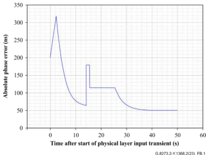
Figure B.1 – Phase error limit for PTP and 1 PPS output phase error transient after the start of the physical layer frequency input transient
