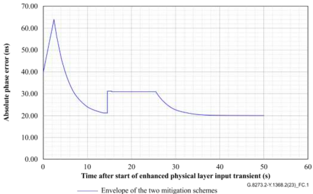
Figure C.1 – Phase error limit for PTP and 1 PPS output phase error transient after the start of the enhanced physical layer frequency input transient
