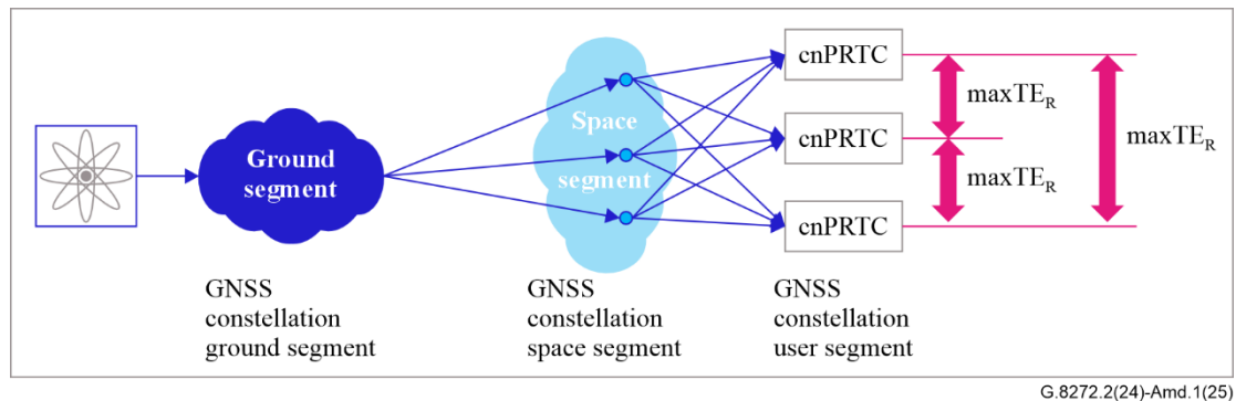
Figure 3 – cnPRTC coherency concept example, based on GNSS
