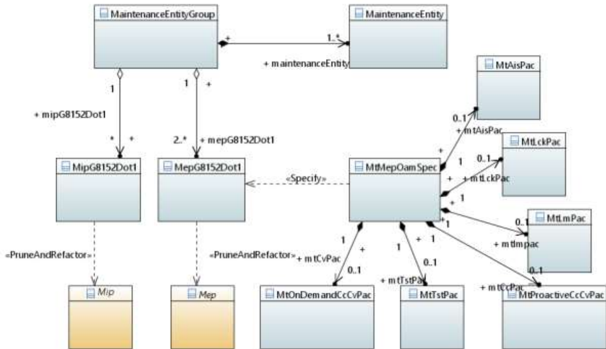
Figure I.1 – OAM configuration
