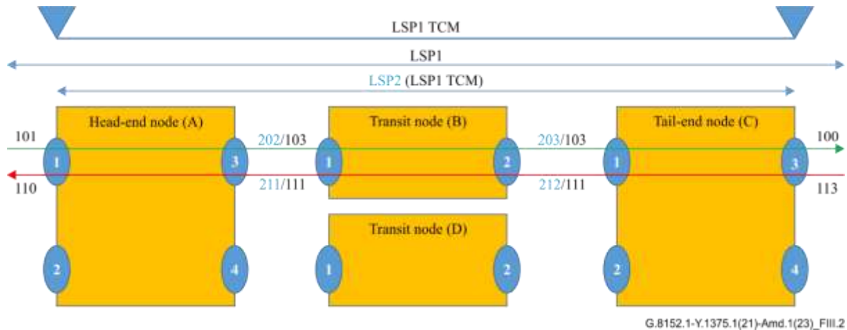
Figure III.2 – Example reference network for LSP TCM
