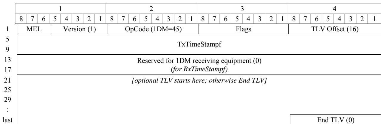
Figure 9.14-1 – 1DM PDU format
