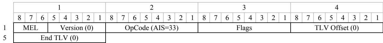
Figure 9.7-1 – AIS PDU format
