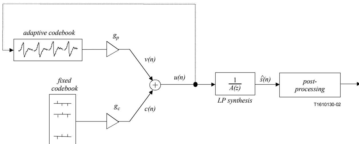
Figure 1/G.722.2 – Simplified block diagram of the CELP synthesis model
