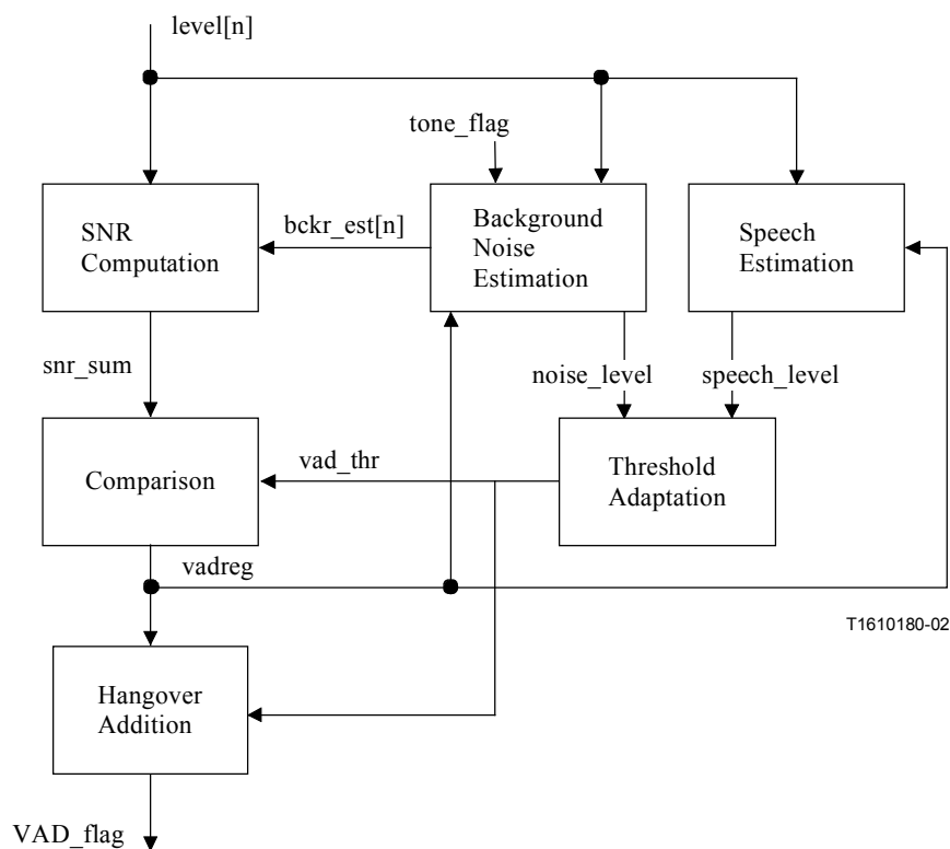
Figure 6/G.722.2 – Simplified block diagram of the VAD decision algorithm
