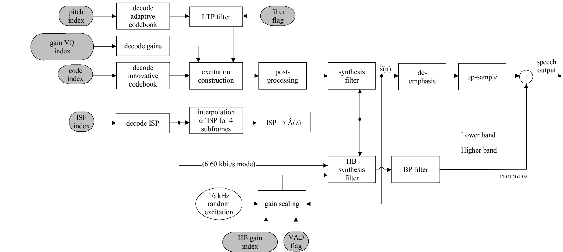
Figure 3 /G.722.2 – Detailed block diagram of the ACELP decoder
