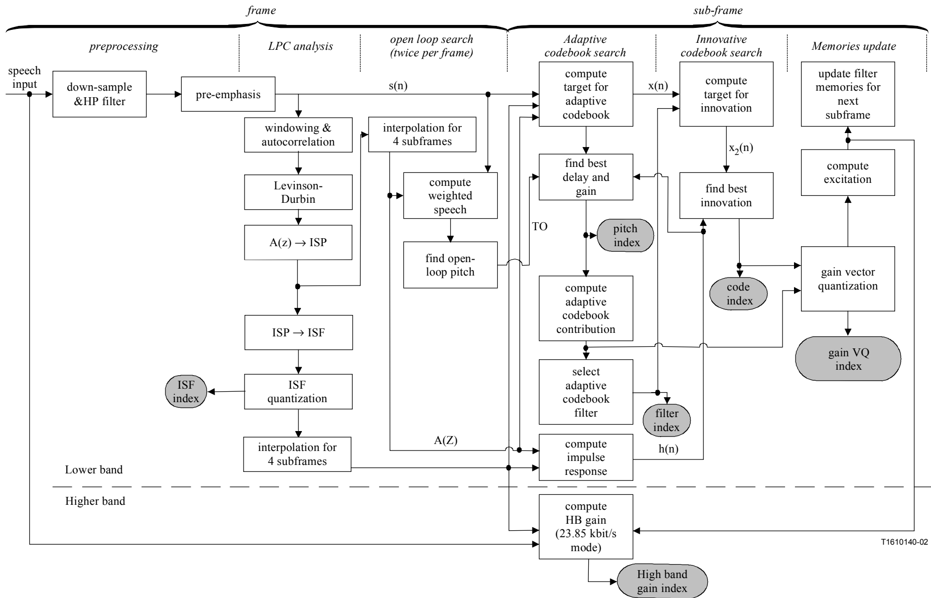
Figure 2/G.722.2–Detailed block diagram of the ACELP encoder
