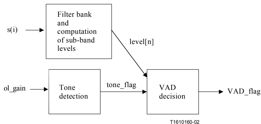
Figure 4/G.722.2 – Simplified block diagram of the VAD algorithm
