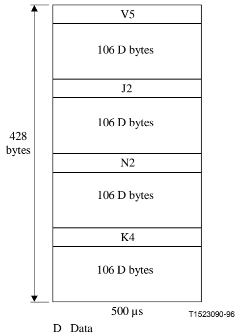
Figure 10-21/G.707/Y.1322 – Mapping of ATM cells into VC-2
