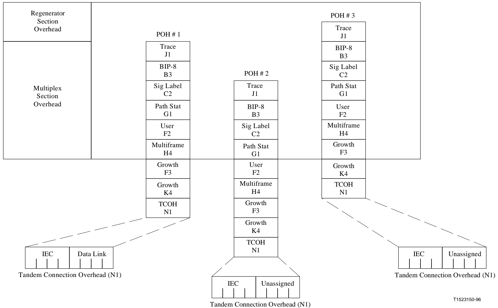
Figure C.1/G.707/Y.1322 – Tandem Connection Overhead in STM-1 rate (AU-3 based) Tandem Connection
