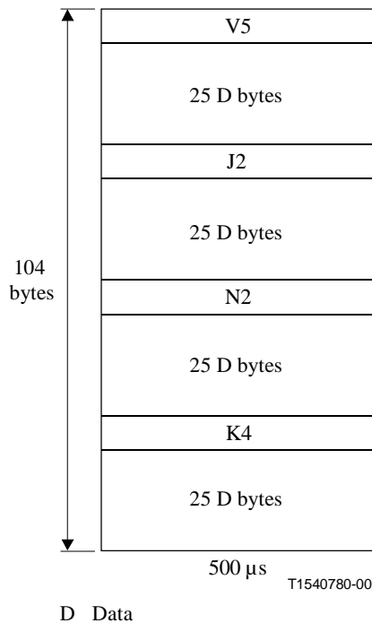
Figure 10-23/G.707/Y.1322 – Mapping of ATM cells into VC-11
