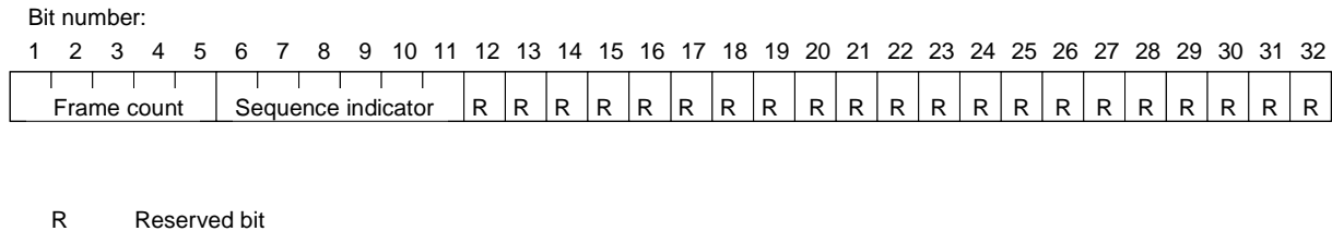
Figure 11-9/G.707 – K4 bit 2 multiframe
