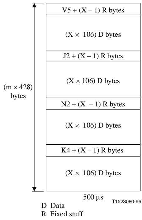
Figure 10-20/G.707/Y.1322 – Mapping of ATM cells into VC-2-Xc using contiguous concatenation
