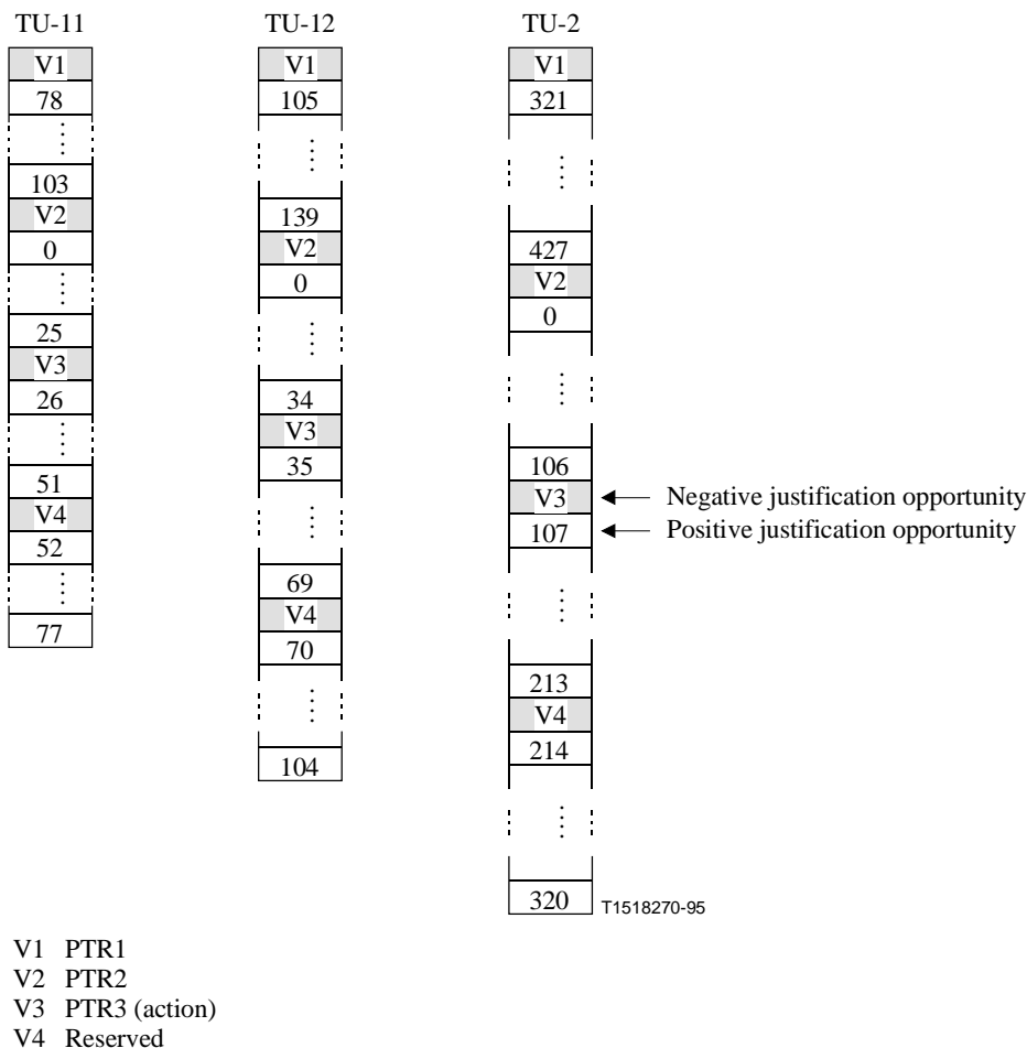
Figure 8-11/G.707/Y.1322 – TU-2/TU-1 pointer offsets
