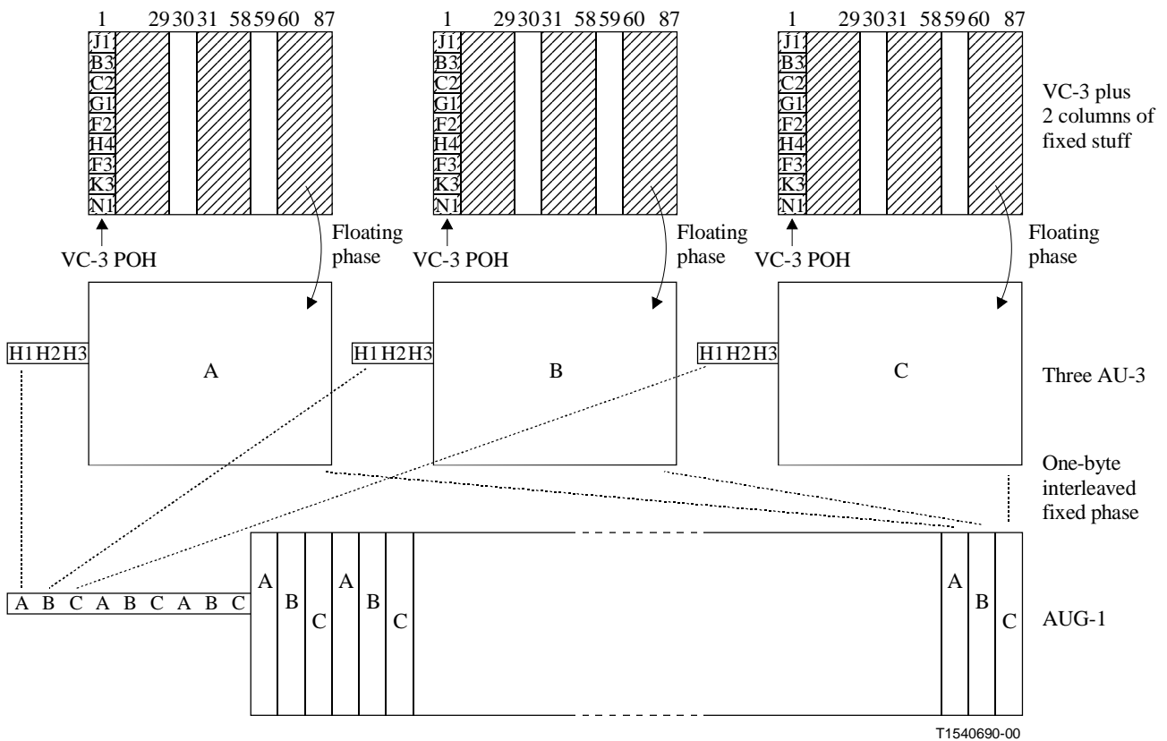
Figure 7-4/G.707/Y.1322 – Multiplexing of AU-3s via AUG-1
