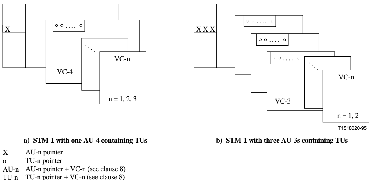
Figure 6-8/G.707/Y.1322 – Two-stage multiplex
