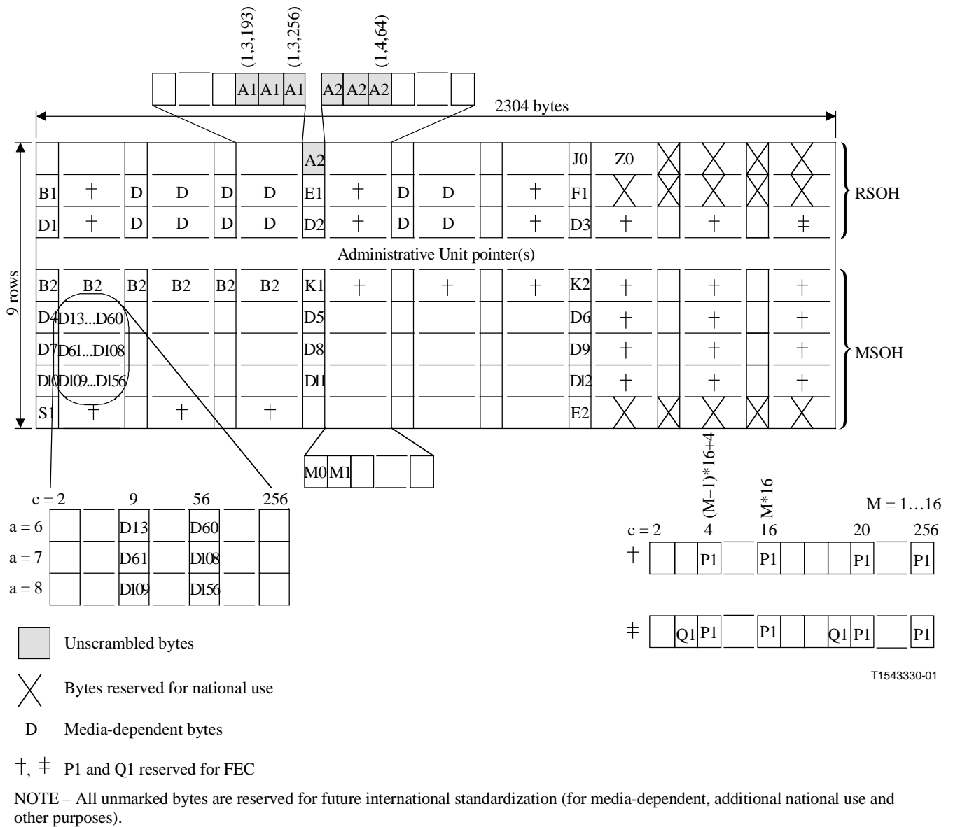
Figure 9-7/G.707/Y.1322 – STM-256 SOH
