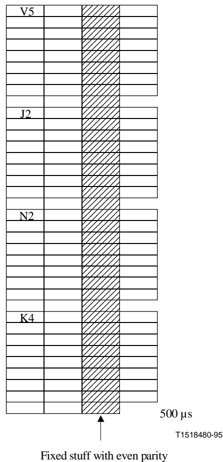
Figure 10-17/G.707/Y.1322 – Conversion of VC-11 to VC-12 for transport by TU-12
