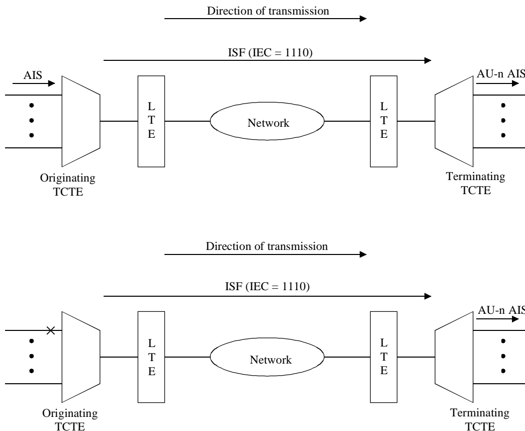
Figure C.8/G.707/Y.1322 – Tandem Connection with incoming signal failures
