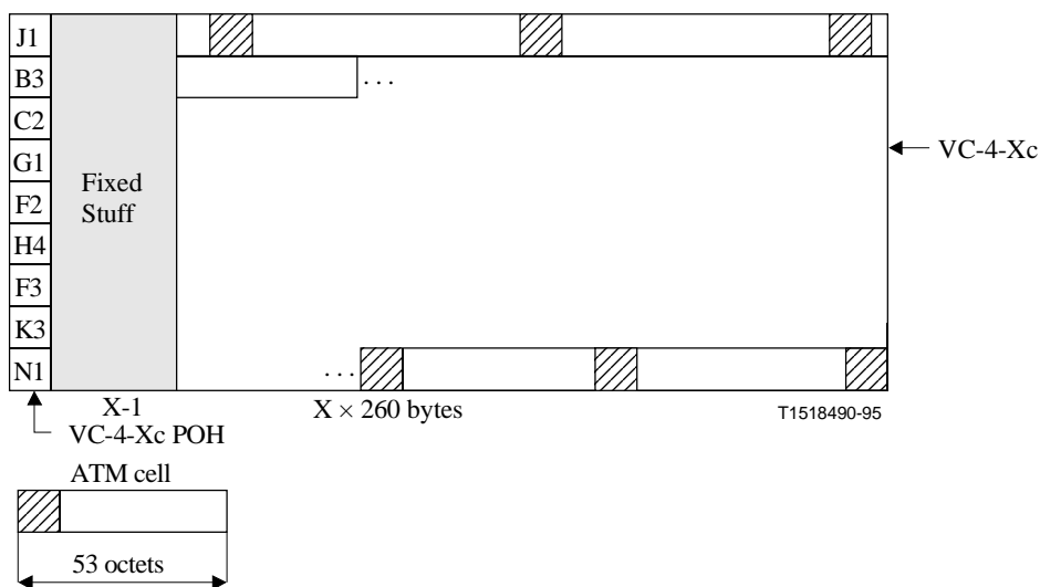
Figure 10-18/G.707/Y.1322 – Mapping of ATM cells into VC-4-Xc
