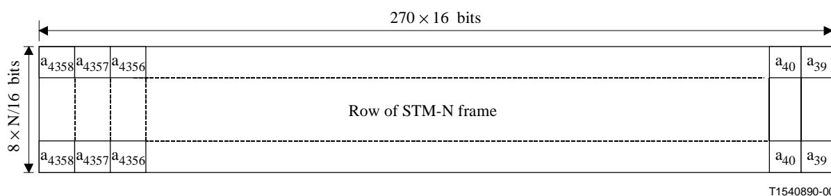
Figure A.1/G.707 – FEC information bits in row K of STM-N frame
