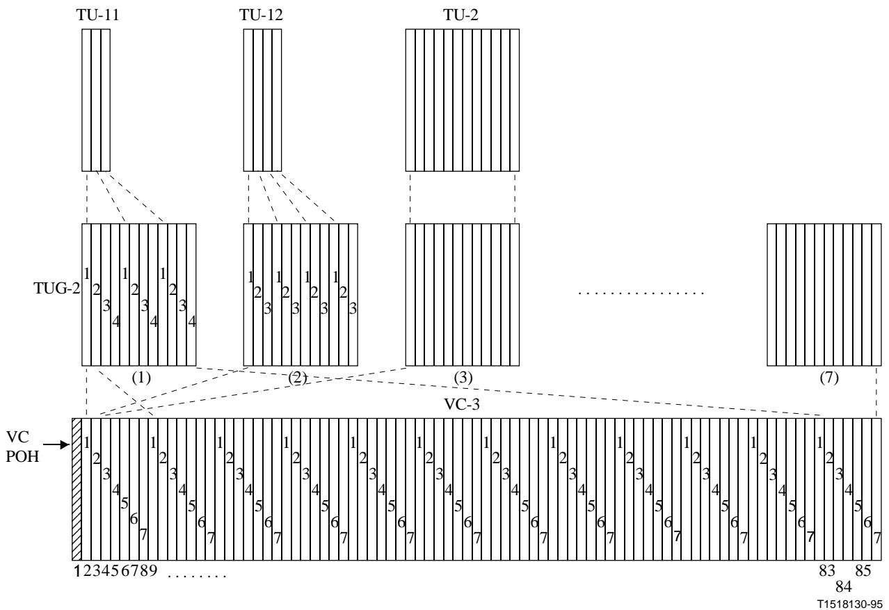
Figure 7-11/G.707/Y.1322 – Arrangement of seven TUG-2s multiplexed into a VC-3
