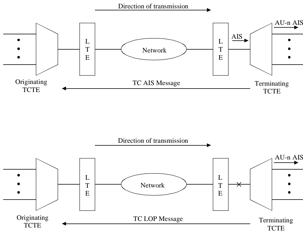
Figure C.9/G.707/Y.1322 – Signal failures within the Tandem Connection
