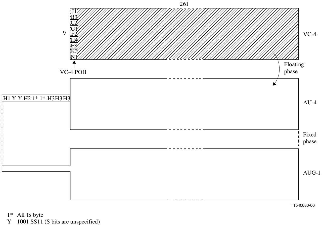
Figure 7-3/G.707/Y.1322 – Multiplexing of AU-4 via AUG-1
