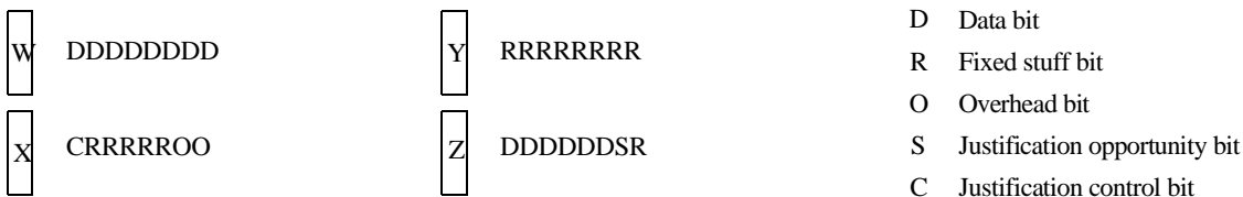
Figure 10-3/G.707/Y.1322 – Asynchronous mapping of 139 264 kbit/s tributary into VC-4
