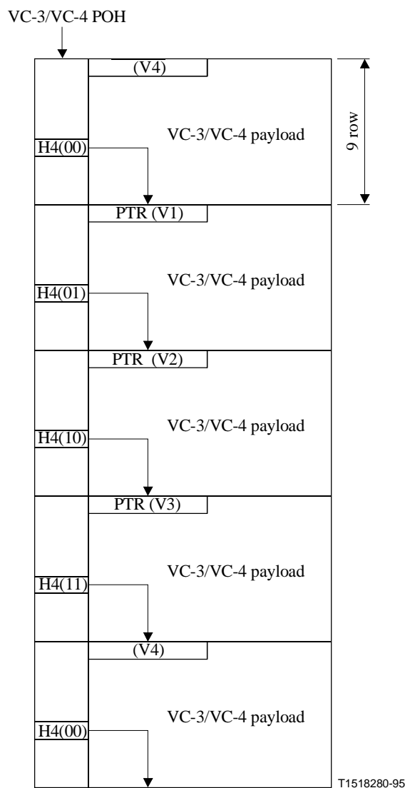
Figure 8-12/G.707/Y.1322 – TU-1/2 500 μs multiframe indication using H4 byte
