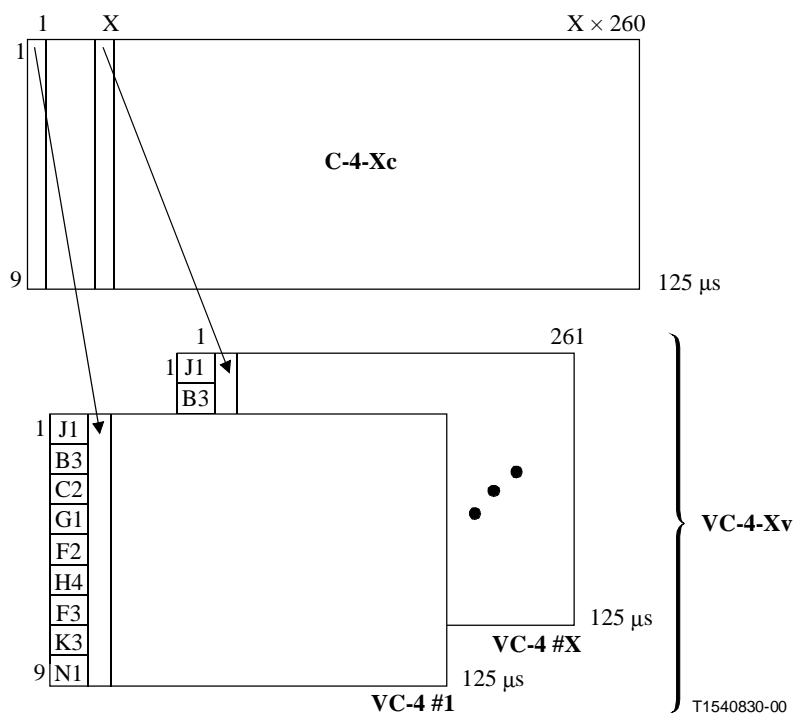
Figure 11-3/G.707/Y.1322 – VC-4-Xv structure
