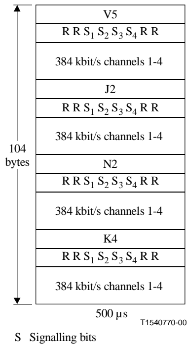
Figure 10-15/G.707/Y.1322 – Byte synchronous mapping for 384 kbit/s tributaries
