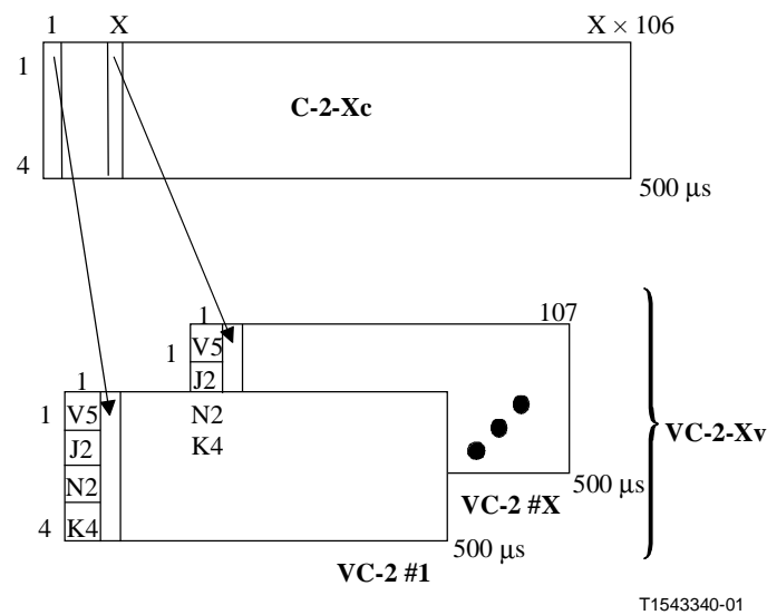
Figure 11-6/G.707 – VC-2-Xv structure
