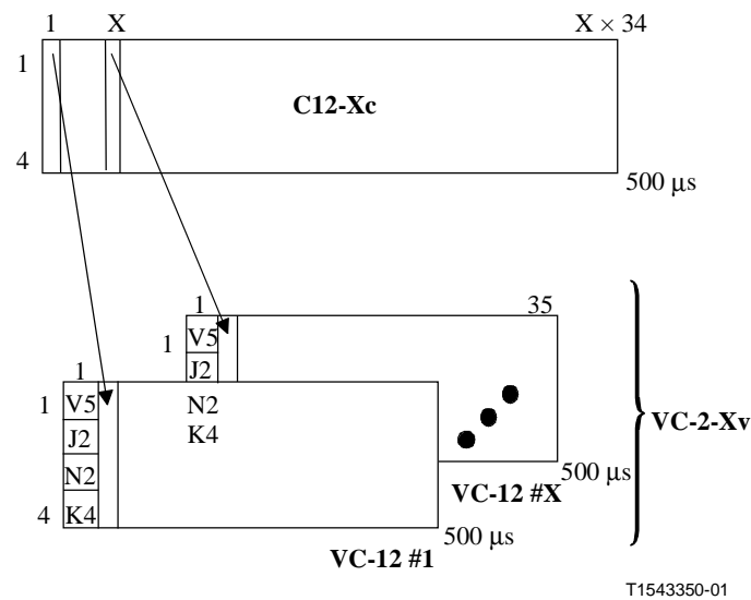
Figure 11-7/G.707 – VC-12-Xv structure
