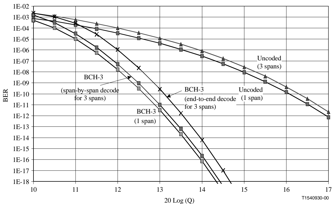
Figure X.3/G.707/Y.1322 – Comparison of end-to-end versus span-by-span FEC
