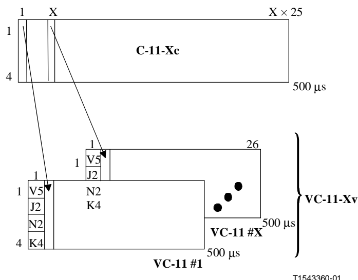
Figure 11-8/G.707 – VC-11-Xv structure
