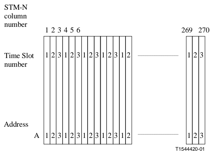
Figure 7-26/G.707/Y.1322 – AU-3 numbering scheme within an STM-1's AU pointer row and payload columns
