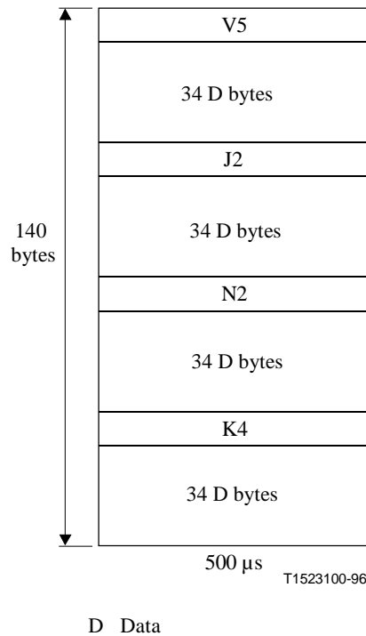
Figure 10-22/G.707/Y.1322 – Mapping of ATM cells into VC-12
