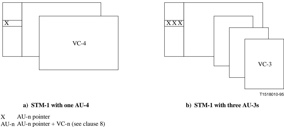
Figure 6-7/G.707/Y.1322 – Administrative Units in STM-1 frame
