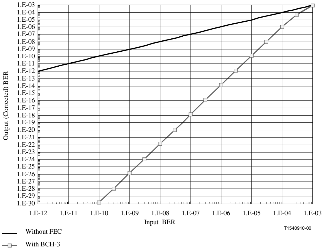
Figure X.1/G.707 – Theoretical output (corrected) BER versus input BER (BCH-3)
