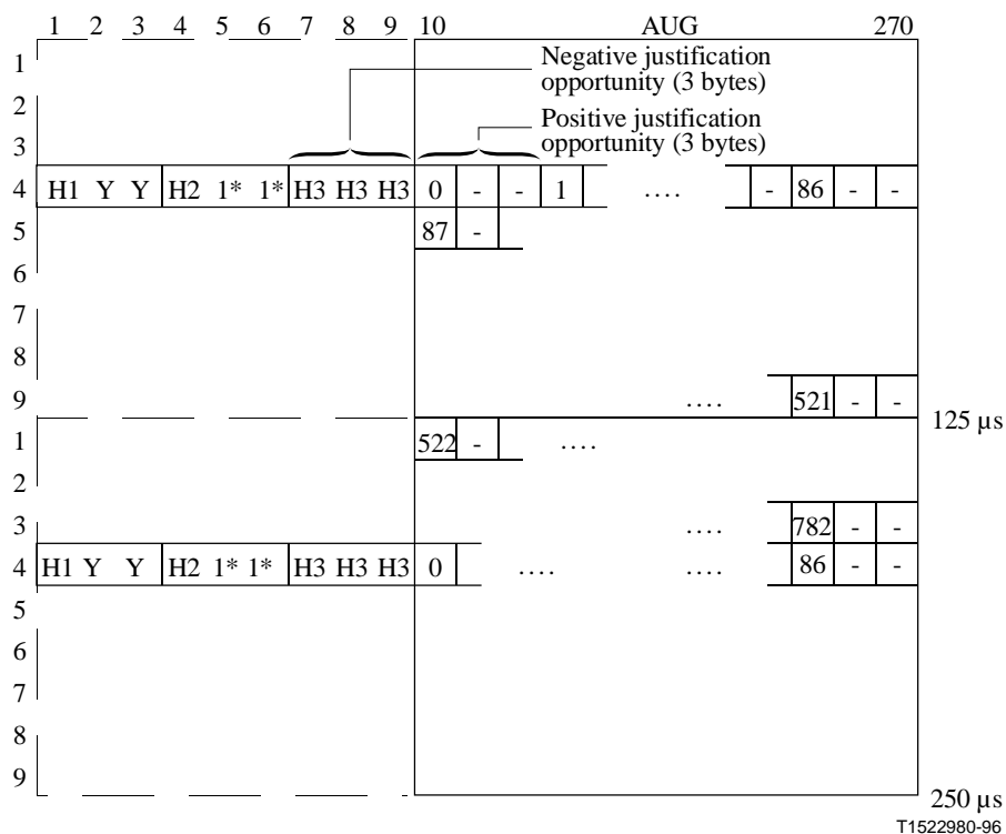
Figure 8-1/G.707/Y.1322 – AU-4 pointer offset numbering
