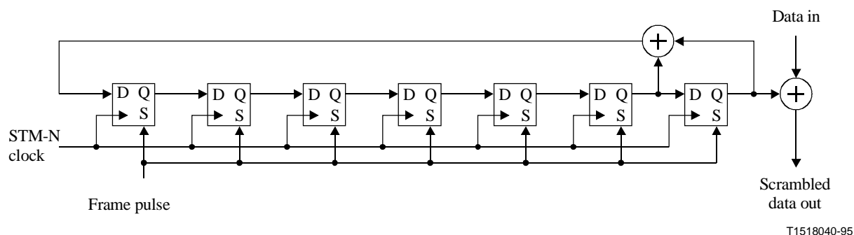
Figure 6-10/G.707/Y.1322 – Frame synchronous scrambler (functional diagram)
