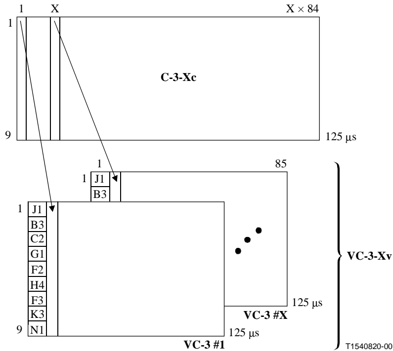
Figure 11-2/G.707/Y.1322 – VC-3-Xv structure
