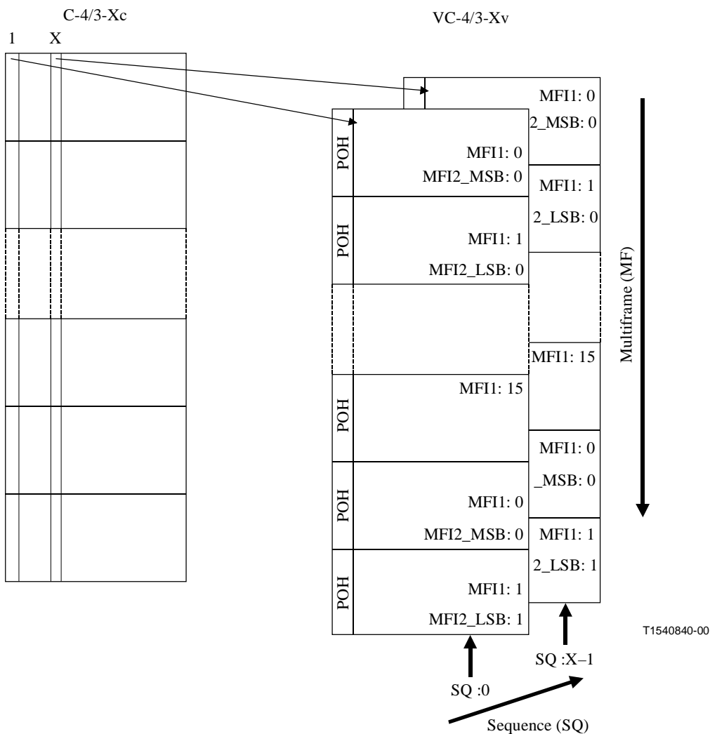
Figure 11-4/G.707/Y.1322 – VC-3/4-Xv multiframe and sequence indicator
