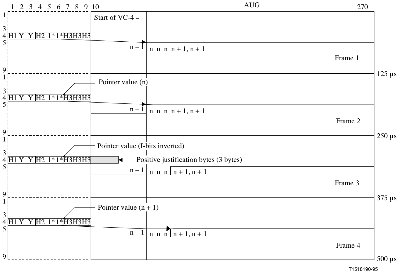
Figure 8-4/G.707/Y.1322 – AU-4 pointer adjustment operation – Positive justification
