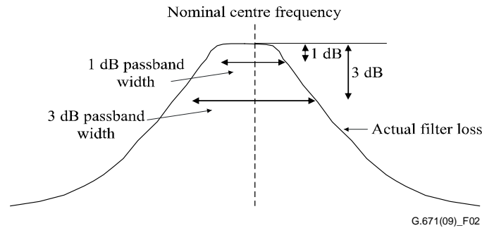
Figure 2 – Illustration of 1 dB and 3 dB passband width
