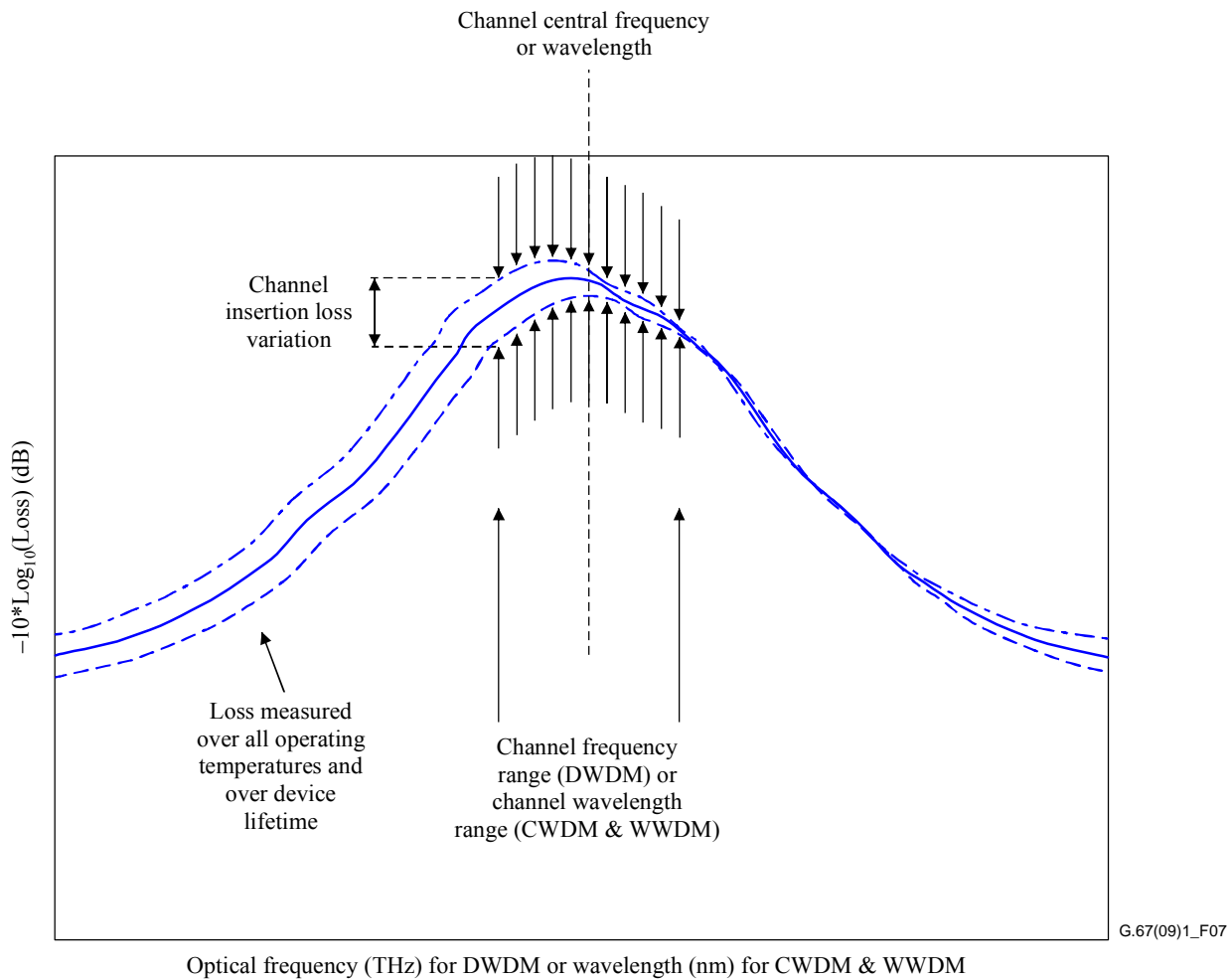
Figure 7 – Illustration of channel insertion loss variation of a WDM device
