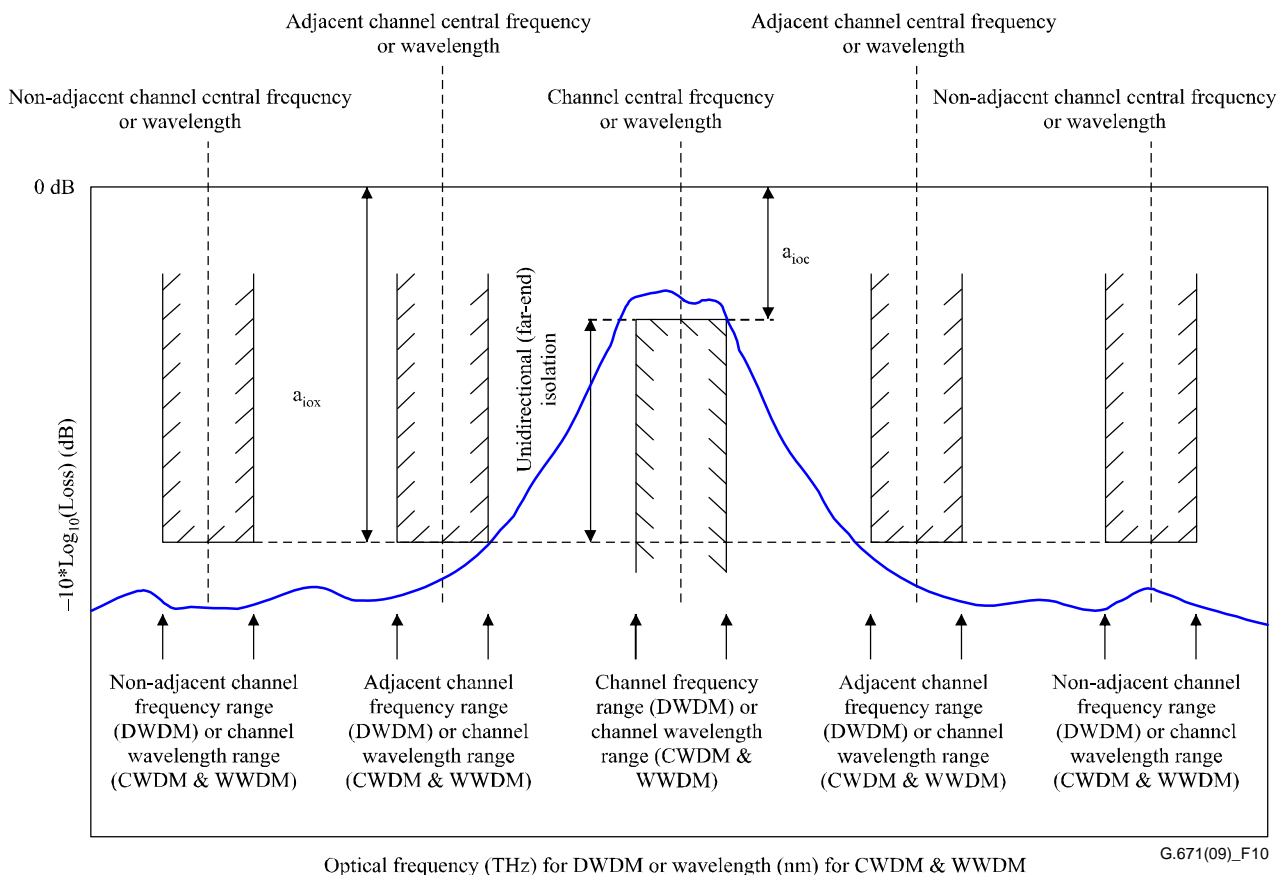
Figure 10 – Illustration of unidirectional (far-end) isolation of a WDM device
