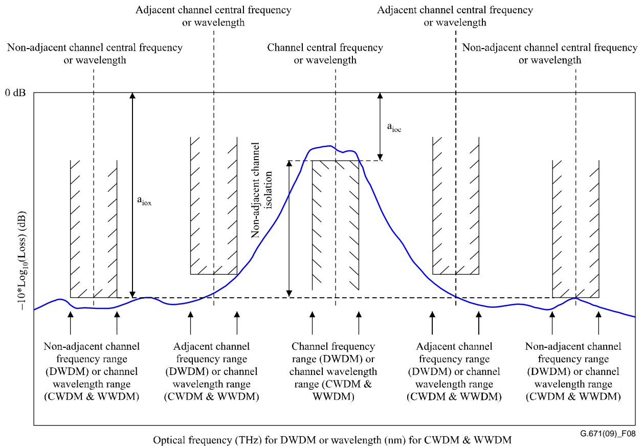
Figure 8 – Illustration of non-adjacent channel isolation for a WDM device
