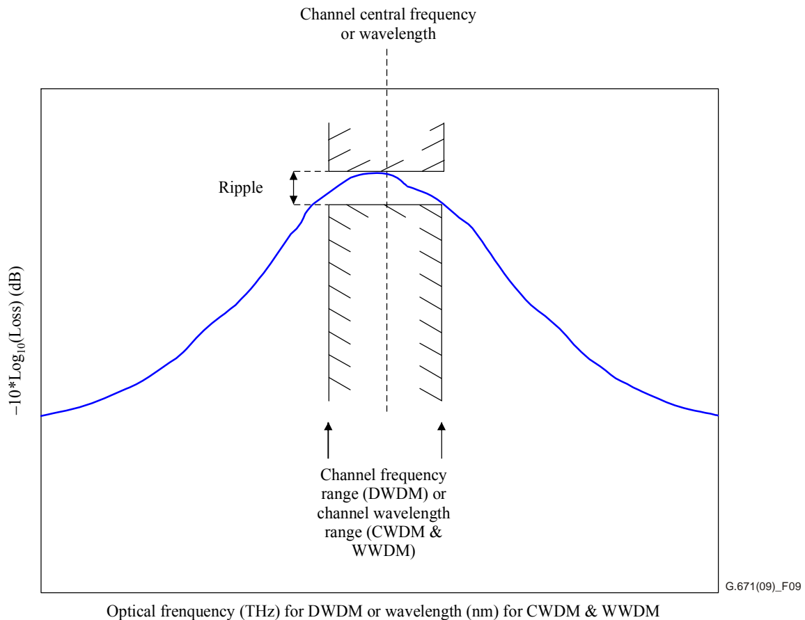
Figure 9 – Illustration of ripple for a WDM device
