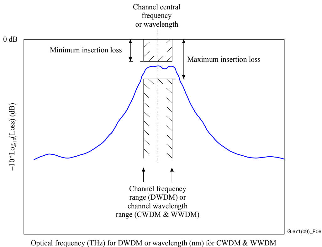
Figure 6 – Illustration of maximum and minimum insertion loss of a WDM device
