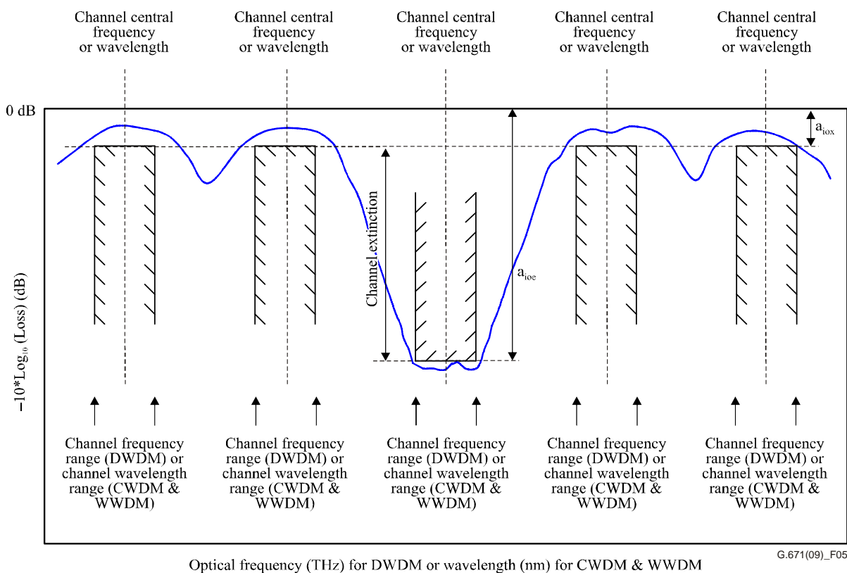
Figure 5 – Illustration of channel extinction of a WDM device
