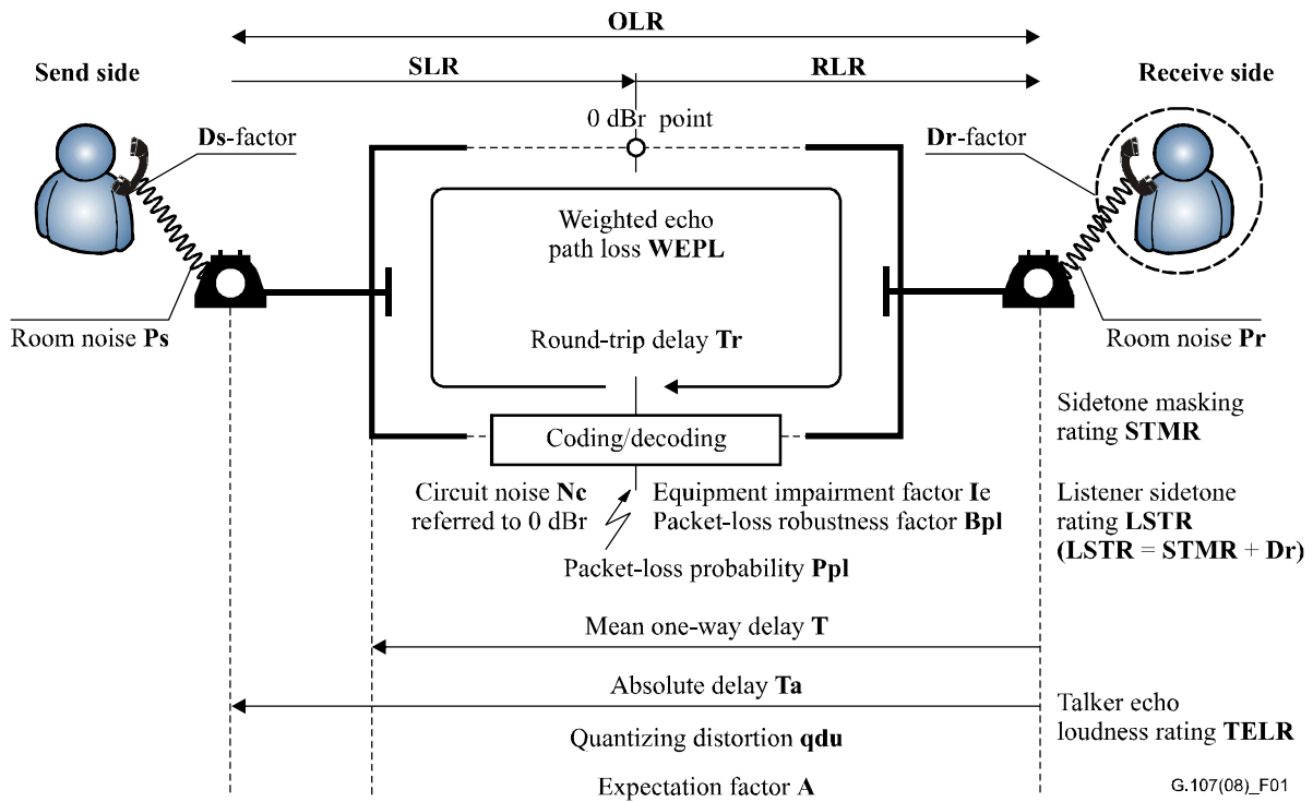
Figure 2 – Reference connection of the wideband E-model
