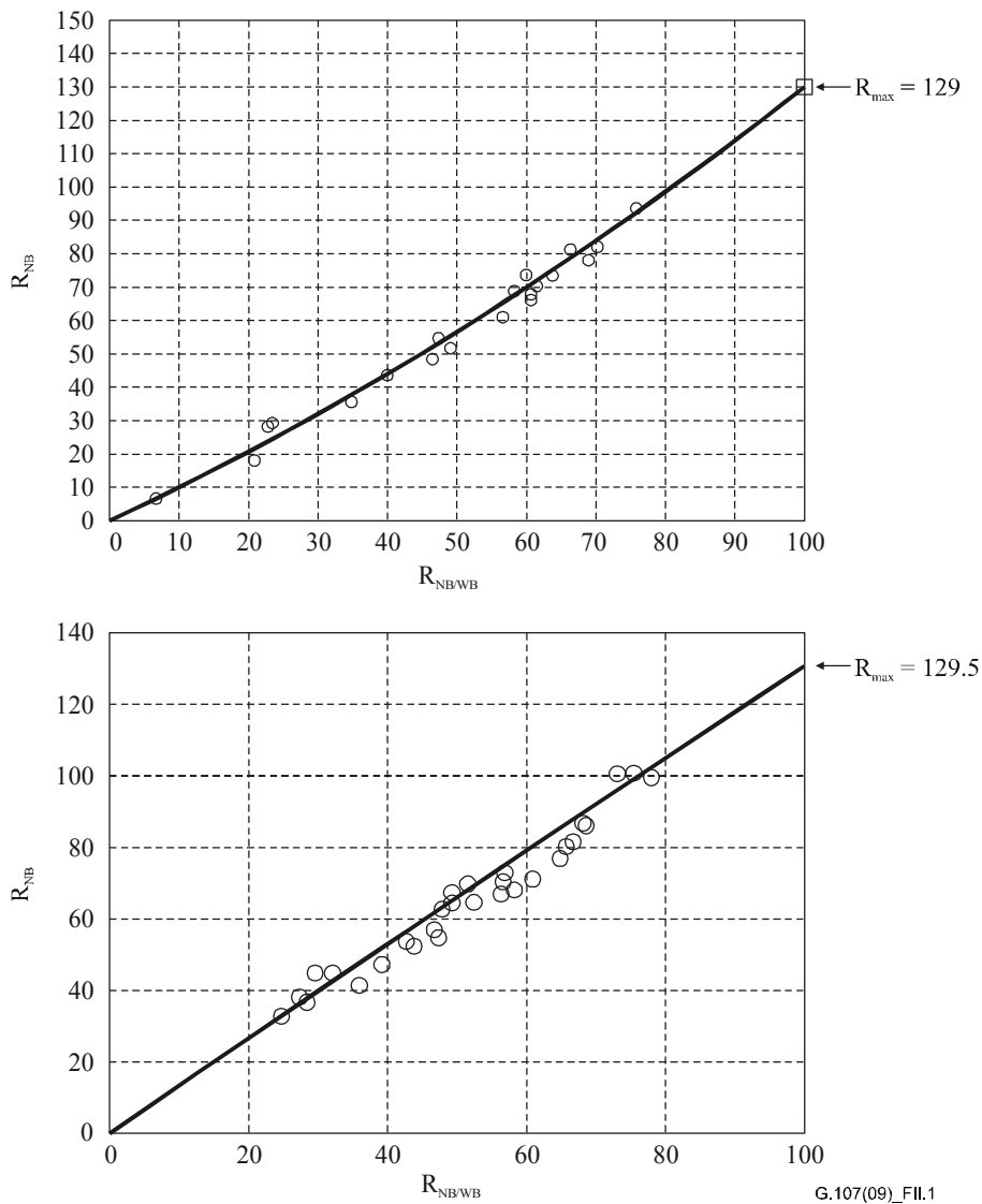
Figure 1 – Comparison between R -values derived in a NB and in a mixed NB/WB context
