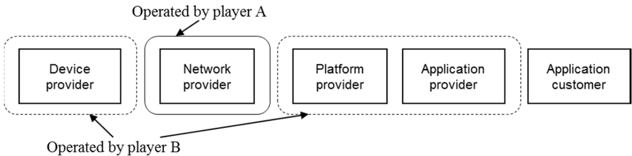
Figure I.5 – Model 4
