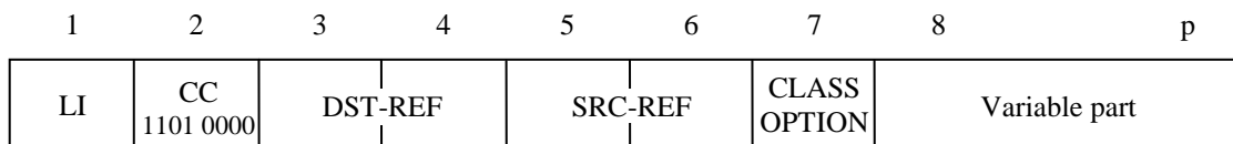
Figure 7 – Connection confirm (CC TPDU)
