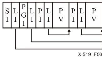
Figure 3 – SPDU with parameters – Grouped
