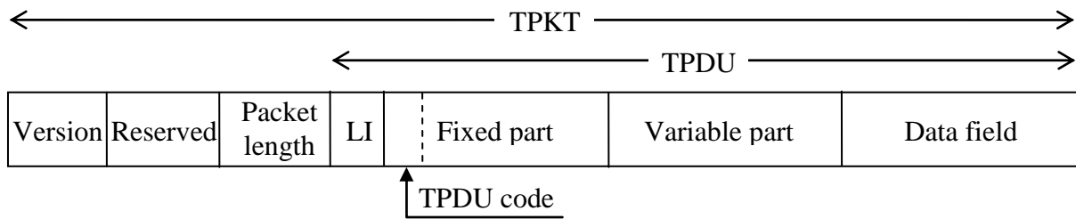
Figure 4 – TPKT structure
