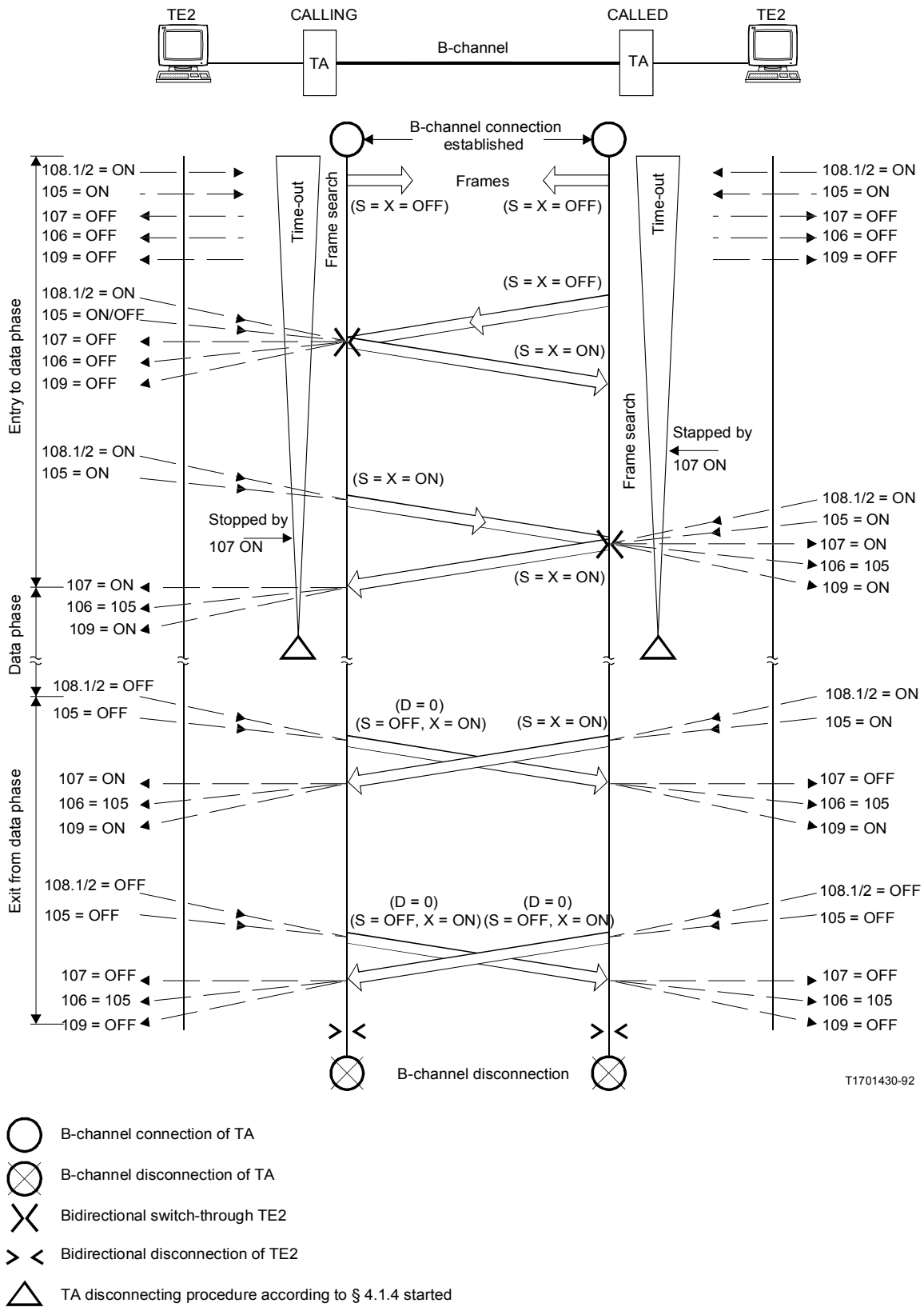
FIGURE 3/V.110 TA synchronization of entry to and exit from data transfer phase
