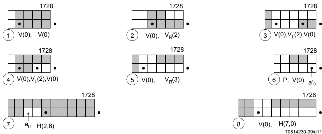
Figure 10/T.4 – Coding examples: First part of scan line
