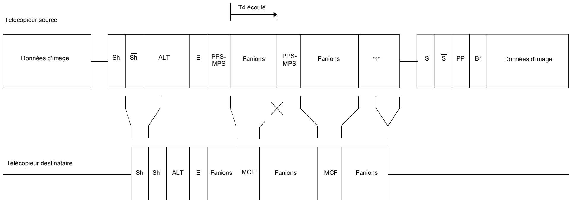
Figure F.5-7/T.30 – Commande de retransmission
