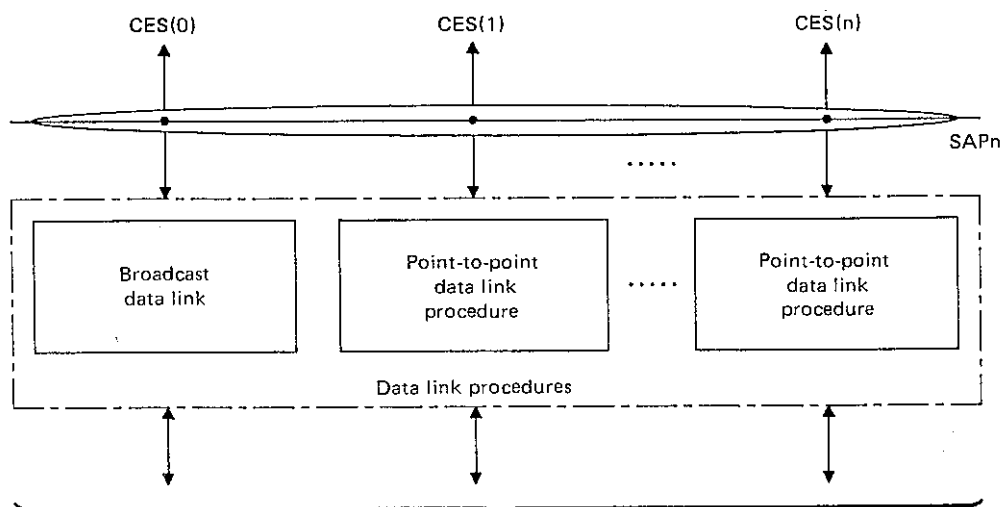
FIGURE 11/Q.920 Data link procedure structure
