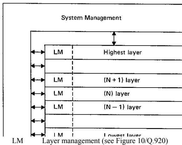
FIGURE 1/Q.920 Layering
