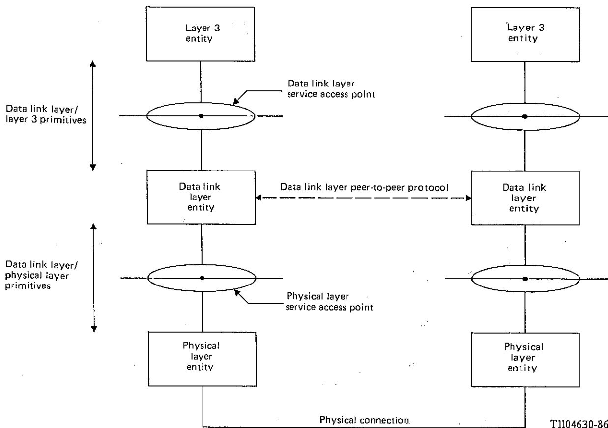
FIGURE 5/Q.920 Data link layer reference model
