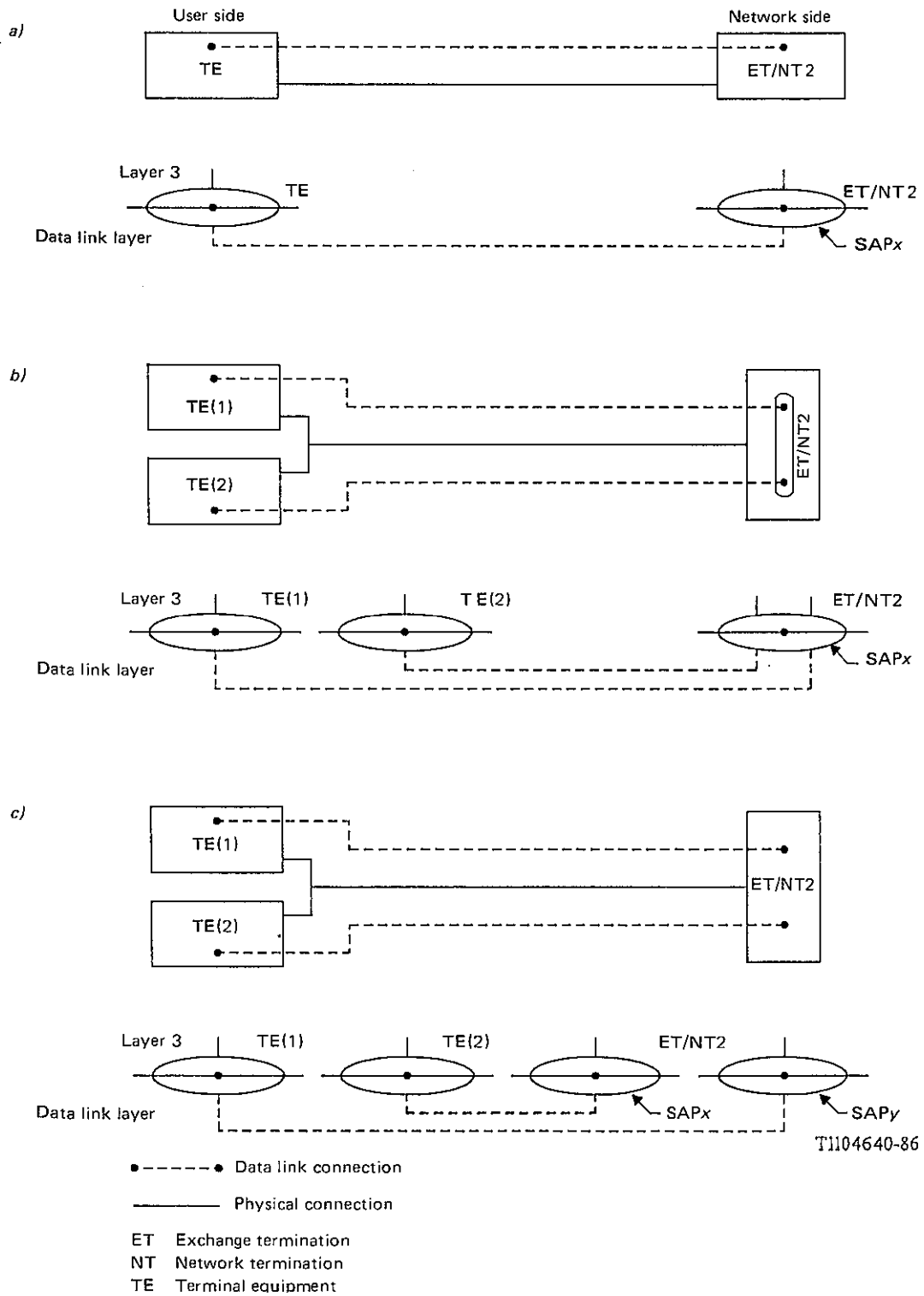
FIGURE 6/Q.920 Point-to-point data link connections
