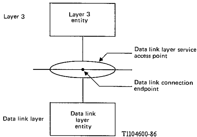
FIGURE 2/Q.920 Entities, service access points and endpoints
