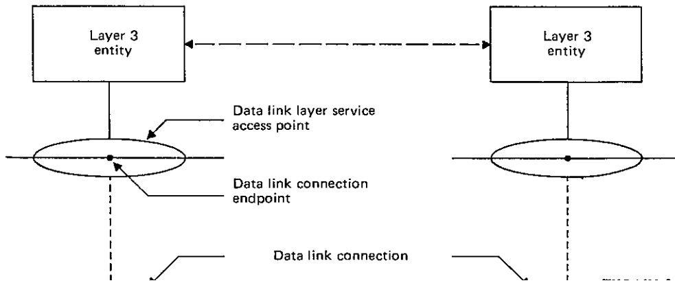
FIGURE 3/Q.920 Peer-to-peer relationship
