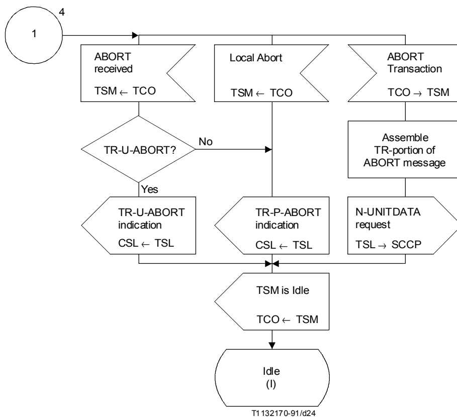
FIGURE A.4/Q.774 (sheet 5 of 5) Transaction state machine
