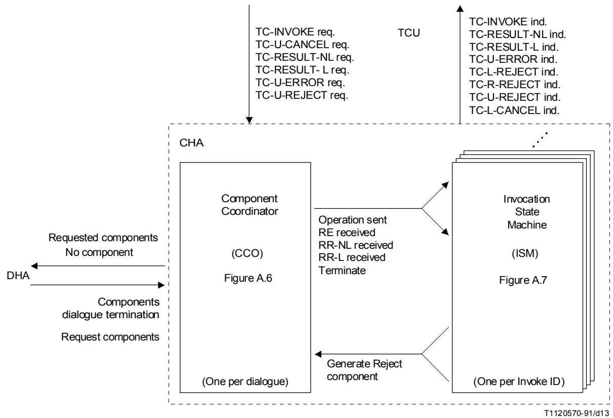
FIGURE A.2c/Q.774 Overview block diagram of CHA
