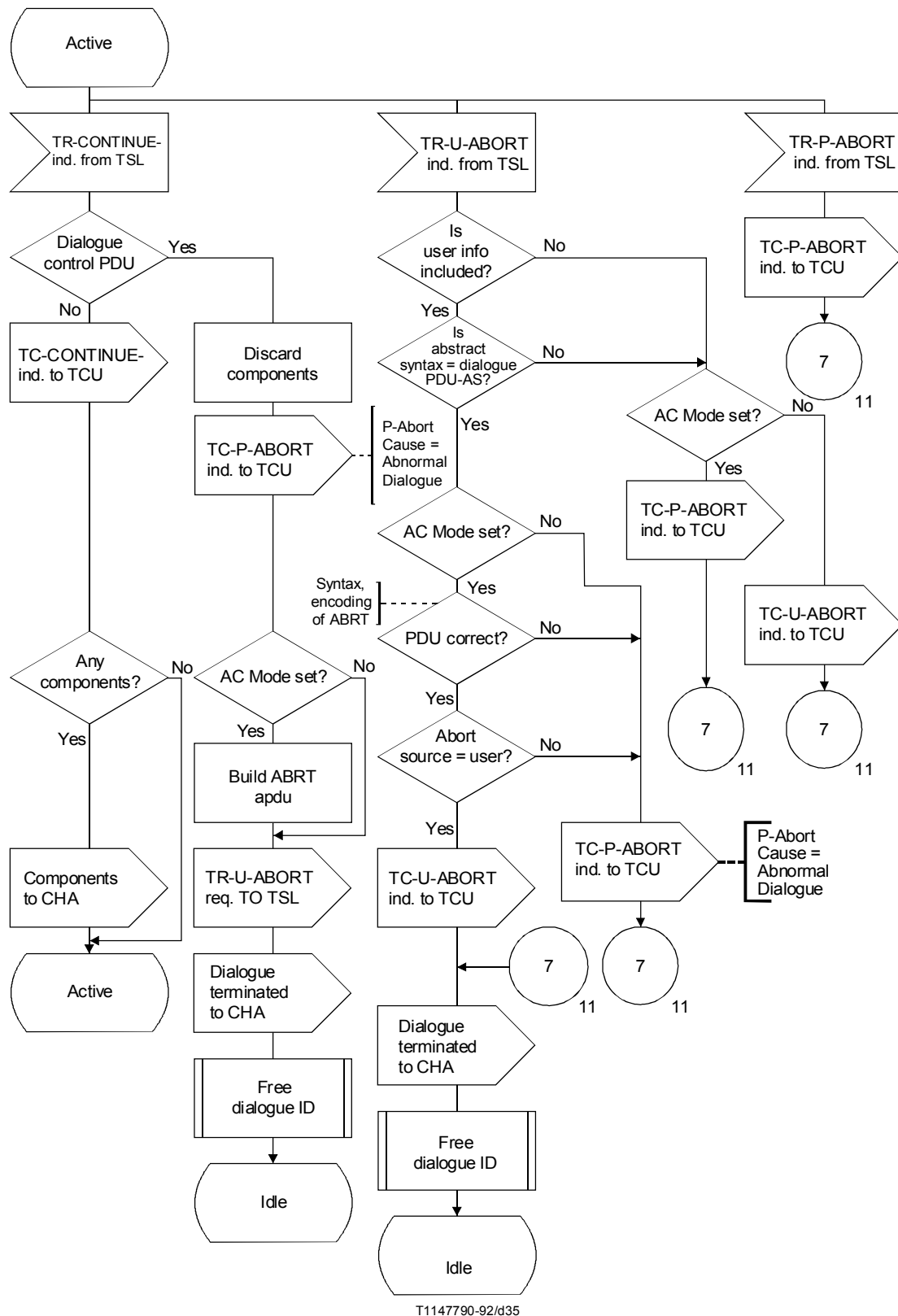
FIGURE A.5/Q.774 (sheet 11 of 11) Dialogue handling at CSL
