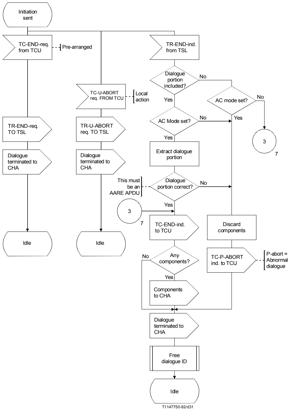
FIGURE A.5/Q.774 (sheet 7 of 11) Dialogue handling at CSL
