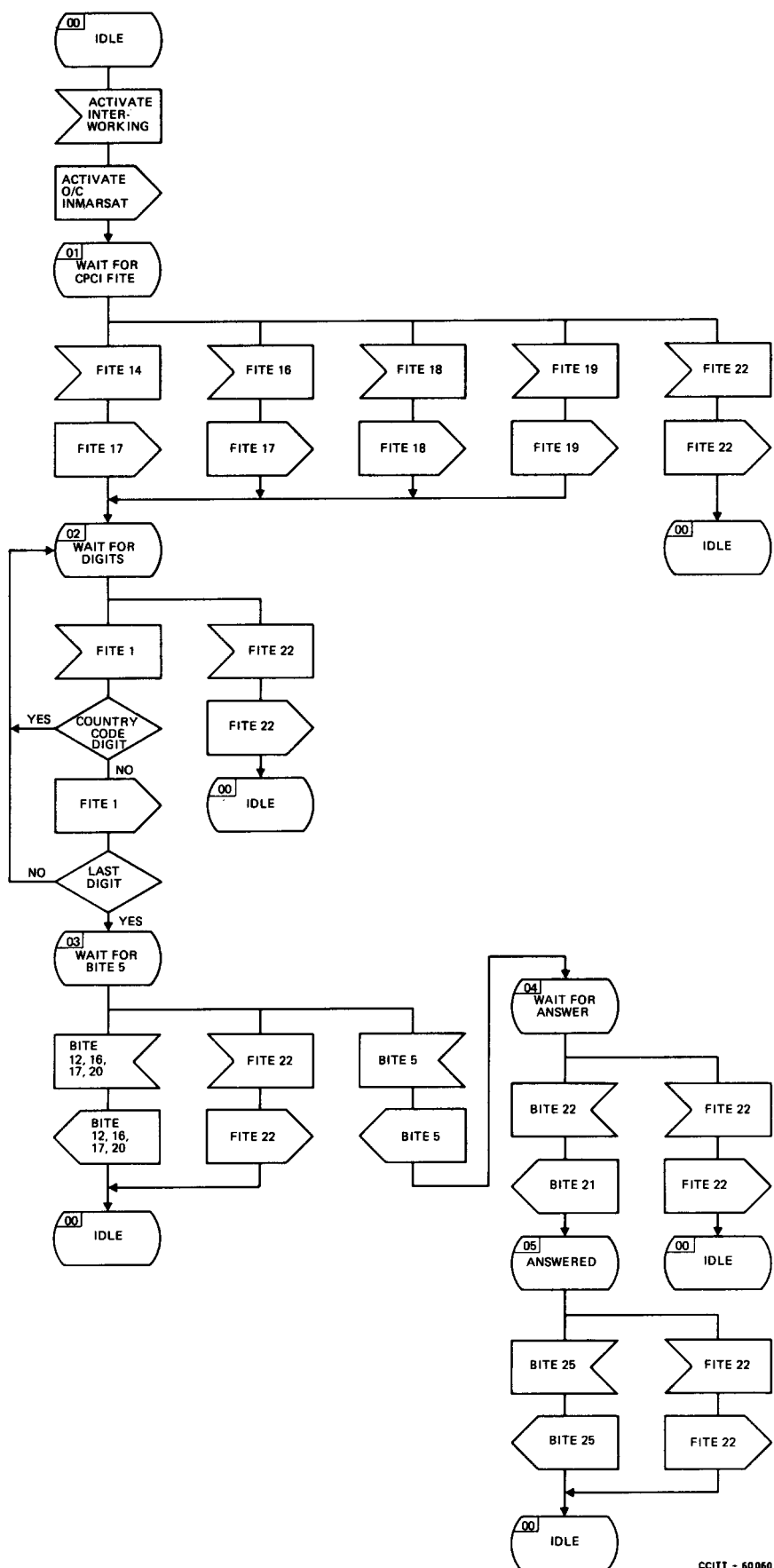
FIGURE A-3/Q.1102
