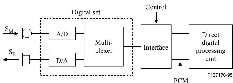
Figure B.1/P.310 – Digital telephone test arrangement (direct digital processing approach)
