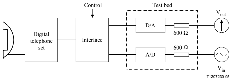
Figure B.9/P.310 – Measurement of terminal coupling loss
