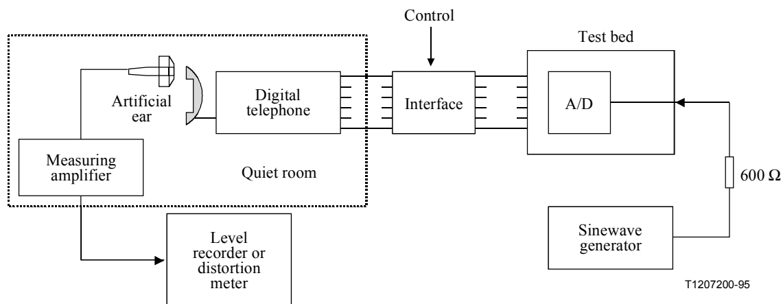
Figure B.5/P.310 – Measurement of receiving frequency characteristic
