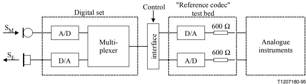
Figure B.2/P.310 – Digital telephone test arrangement (codec approach)
