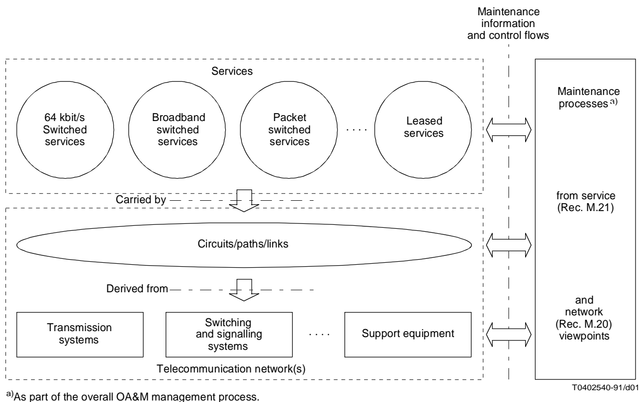
FIGURE 1/M.10 Service/network relationships for maintenance
