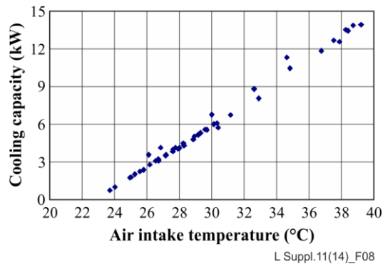
Figure 8 – Air intake temperature and cooling performance
