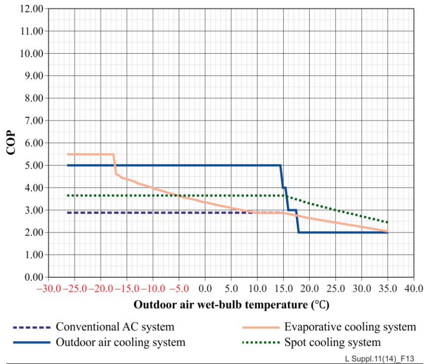
Figure 13 – Comparison of coefficient of performance (COP) with outdoor air conditions (Heat density 2 kW/m 2 )
