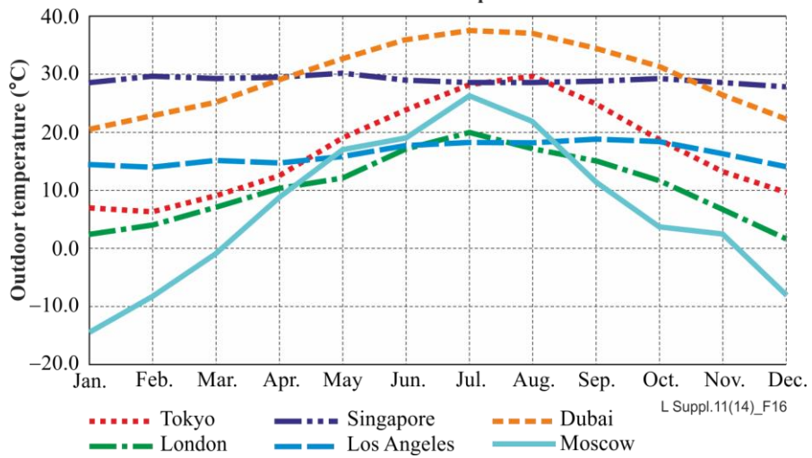
Figure 16 – Calculation of location and outdoor air temperature
