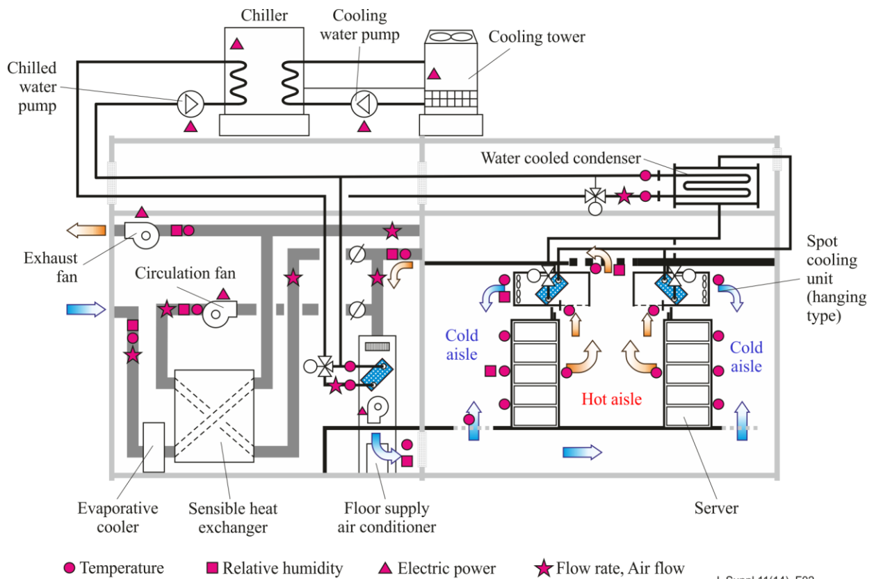
Figure 2 – Outline of measurement points
