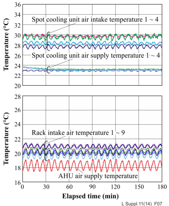
Figure 7 – Spot cooling method operational state (example)
