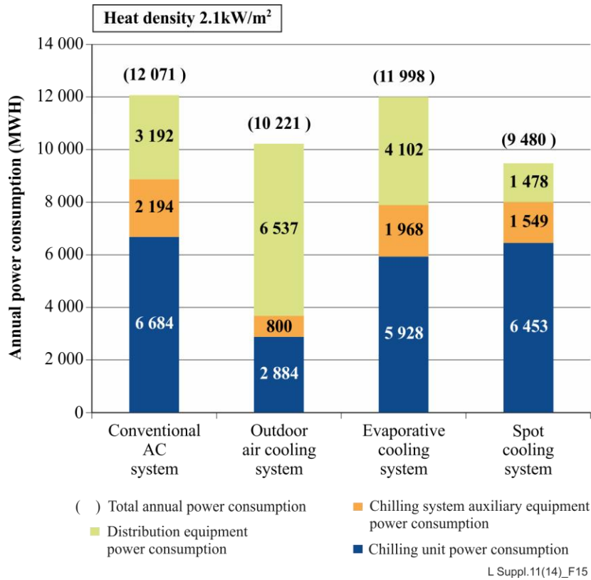
Figure 15 – Comparison of annual power consumption with air conditioning methods in Tokyo
