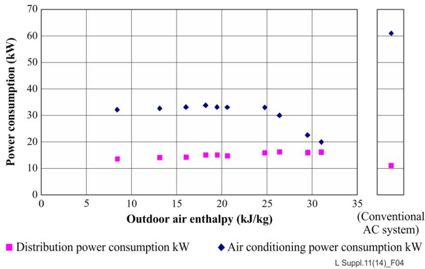
Figure 4 – Outdoor air enthalpy and distribution power consumption
