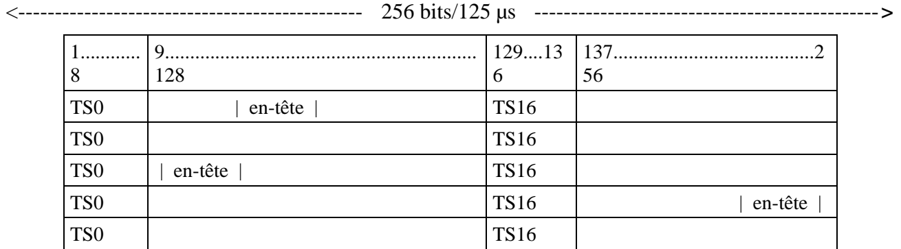
Figure 2/I.432.3 – Mappage des cellules ATM
