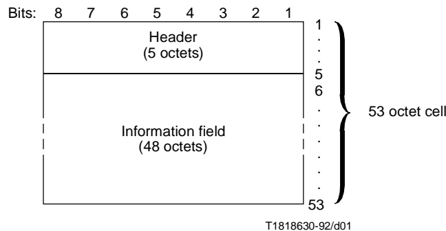
FIGURE 1/I.361 Cell structure at the UNI/NNI
