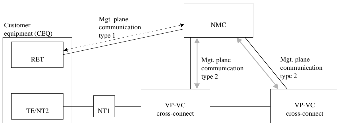
a) (Semi-) permanent/reserved VPC/VCC request
