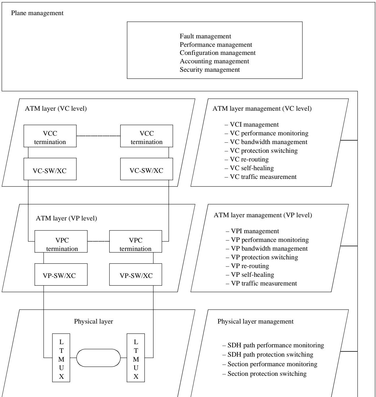
Figure II.1/I.311 – B-ISDN network management functional description
