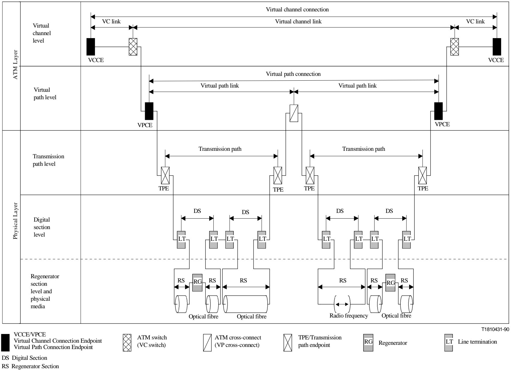
Figure A.1/I.311 – Hierarchical structure of a cell-based ATM transport network
