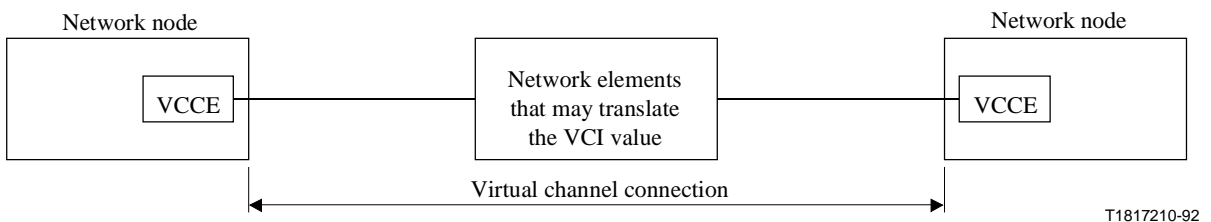
Figure 5c/I.311 – Network-network application of the virtual channel connection
