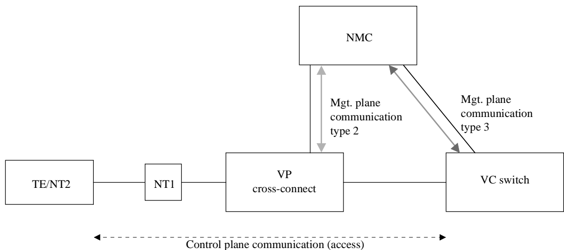
c) On-demand VPC/VCC request
