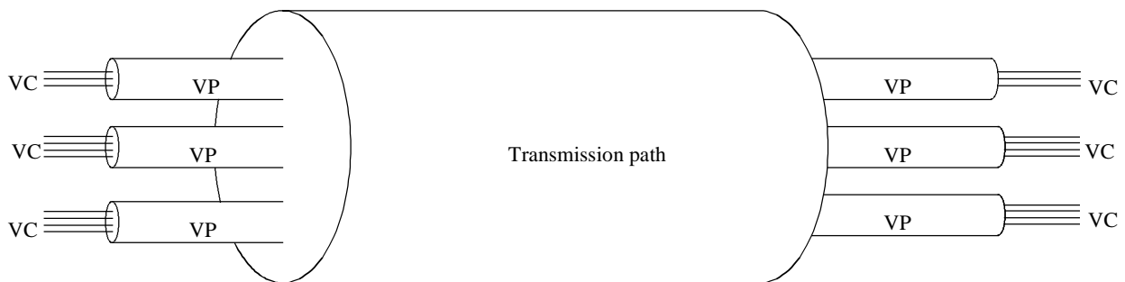
Figure 2/I.311 – Relationship between the VC, the VP and transmission path
