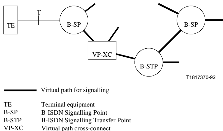
Figure I.1/I.311 – Example of a path within the B-ISDN signalling network
