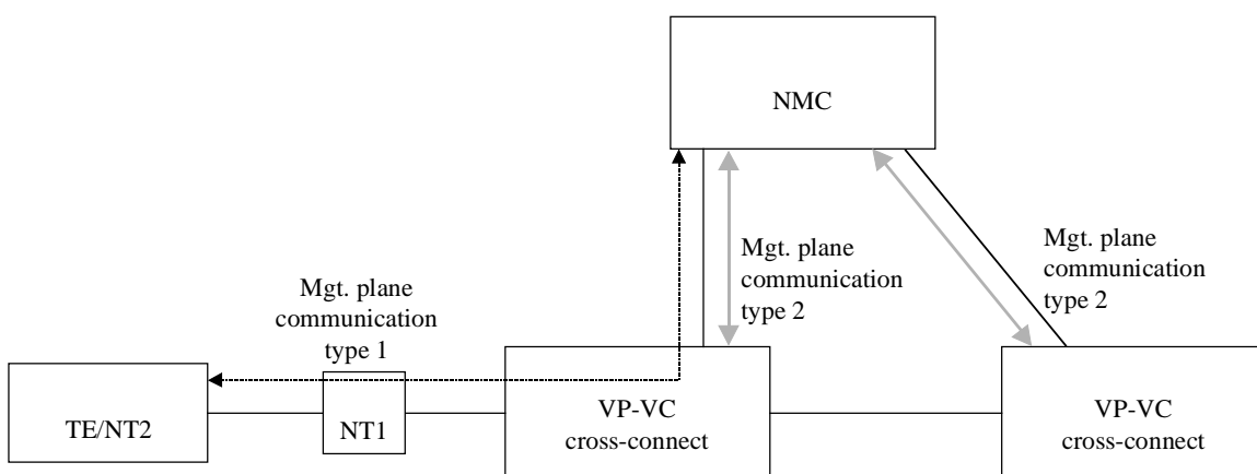
b) (Semi-) permanent/reserved VPC/VCC request
