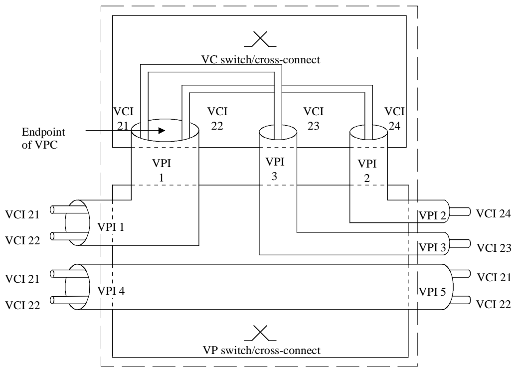
a) Representation of VC and VP switching
