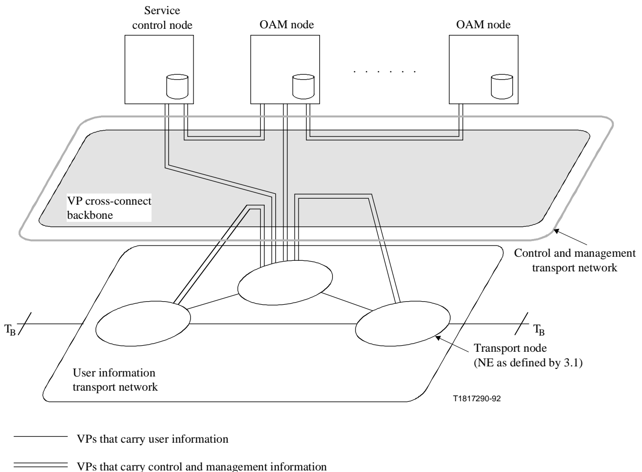
Figure 10/I.311 – An example of control and management transport network architecture using VP cross-connect backbone
