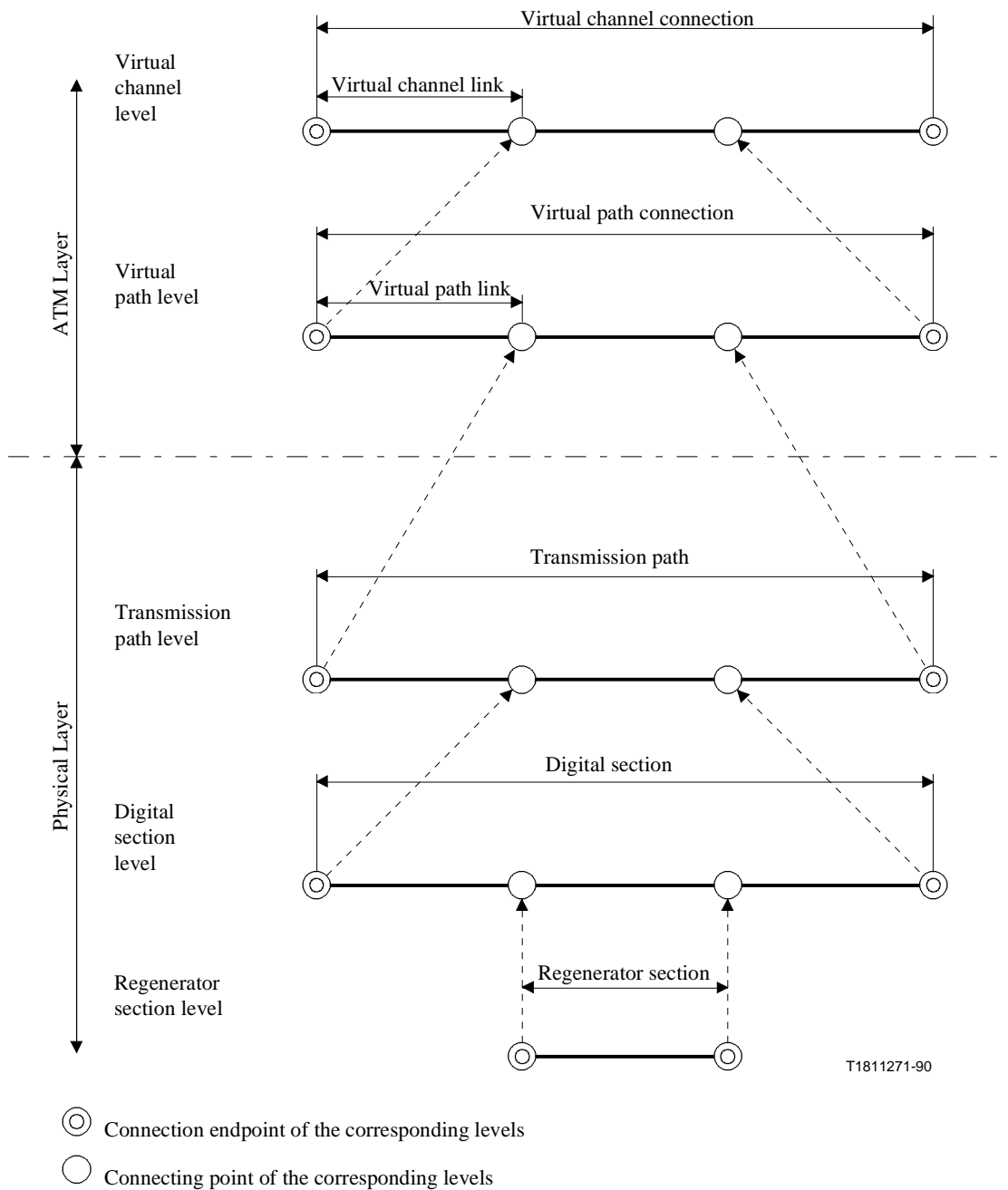
Figure 3/I.311 – Hierarchical layer-to-layer relationship
