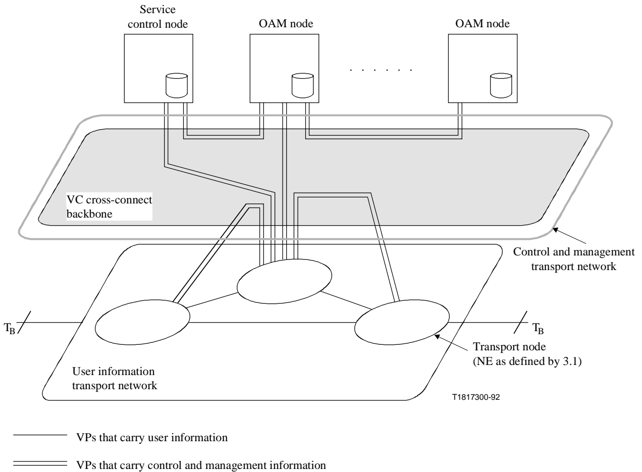
Figure 11/I.311 – An example of control and management transport network architecture using VC cross-connect backbone
