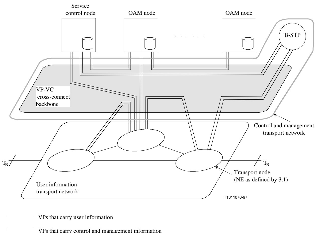
Figure 12/I.311 – An example of control and management transport network architecture with B-STP functionality
