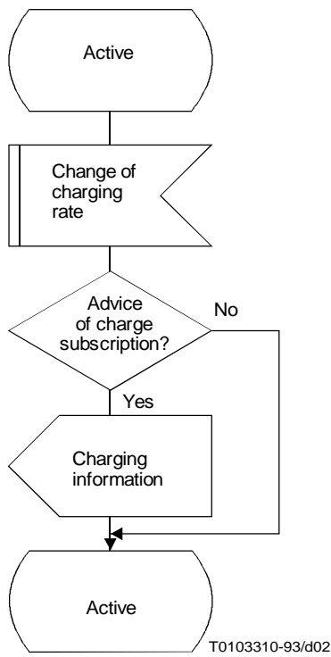
FIGURE 2/I.256.2a Charging information – Change of charging rate at the active phase of a call
