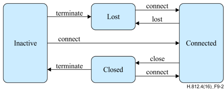
Figure 9-2 – State diagram for the status topic
