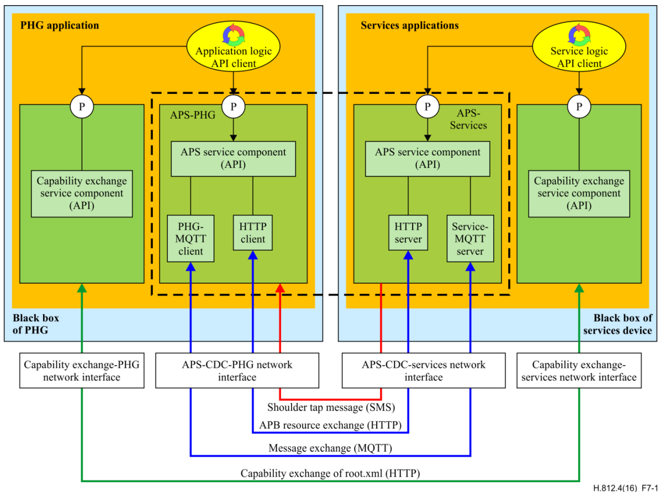
Figure 7-1 – APS framework
