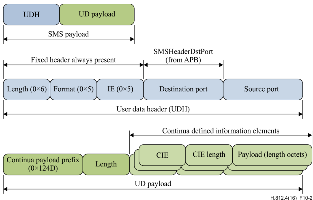
Figure 10-2 – Payload of binary SMS message
