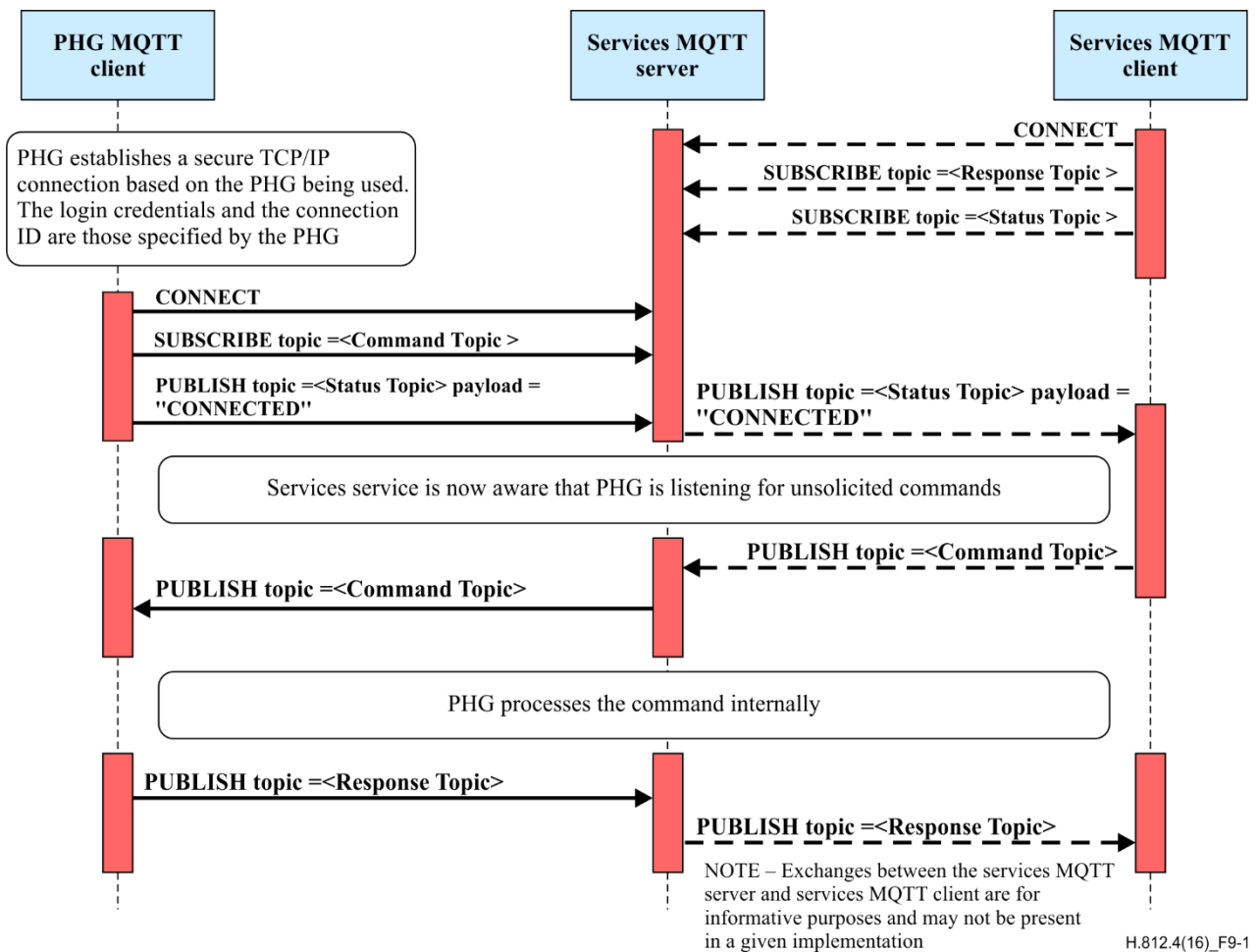
Figure 9-1 – PHG application and Health & Fitness services application MQTT client interactions
